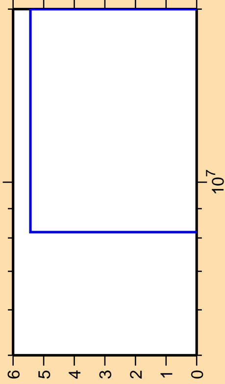
\Delta\sigma/\sigma vs. E for ^{204}\text{Po}(n,2n)
