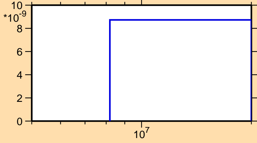
\sigma vs. E for ^{204}\text{Po}(n,\text{He}3)
