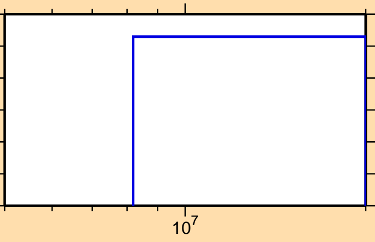
\sigma vs. E for ^{204}\text{Po}(n,3n)
