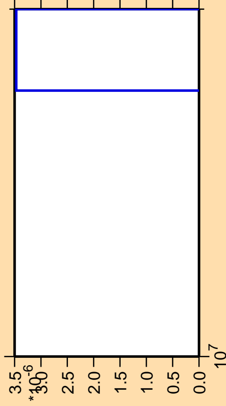
\Delta\sigma/\sigma vs. E for ^{205}\text{Po}(\text{mt } 11)
