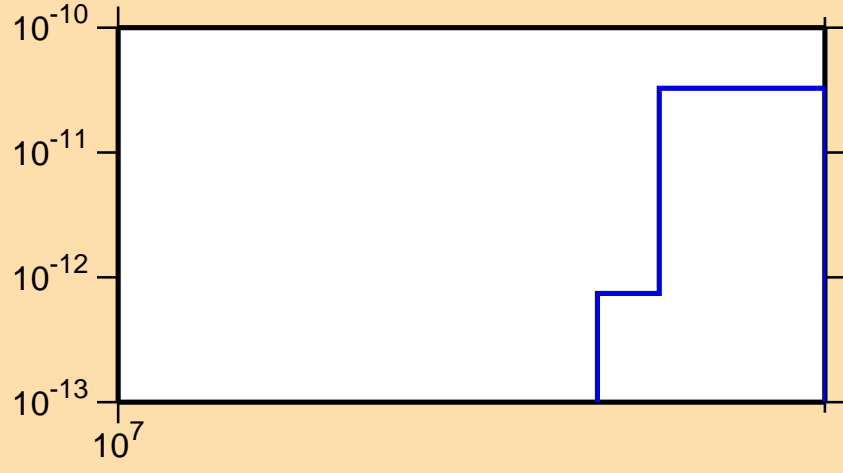
\sigma vs. E for ^{205}\text{Po} (mt 34)
