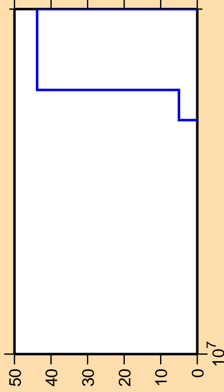
\Delta\sigma/\sigma vs. E for ^{205}\text{Po} (mt 45)
