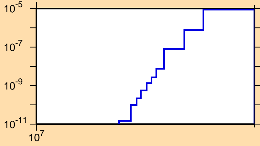
\sigma vs. E for ^{205}\text{Po}(n,\text{nd})
