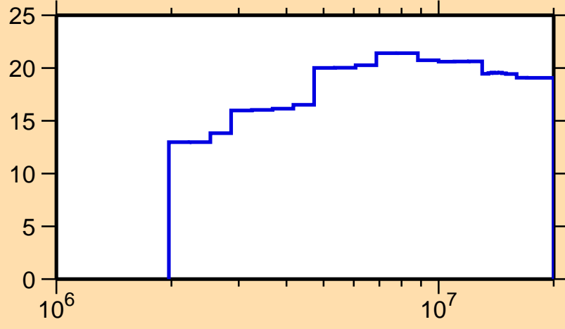
\Delta\sigma/\sigma vs. E for ^{205}\text{Po}(n, n_1)
