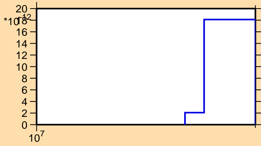
\sigma vs. E for ^{205}\text{Po} (mt 45)
