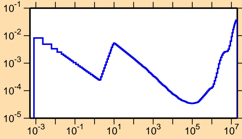
\sigma vs. E for ^{205}\text{Po}(n,p)
