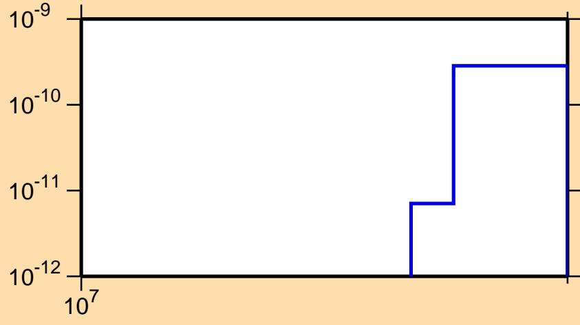
\sigma vs. E for ^{205}\text{Po}(n,\text{pt})
