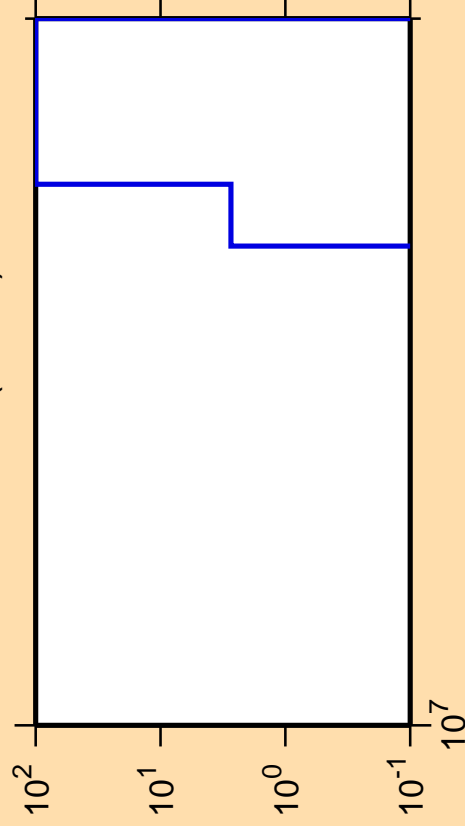
\Delta\sigma/\sigma vs. E for ^{205}\text{Po} (mt 34)
