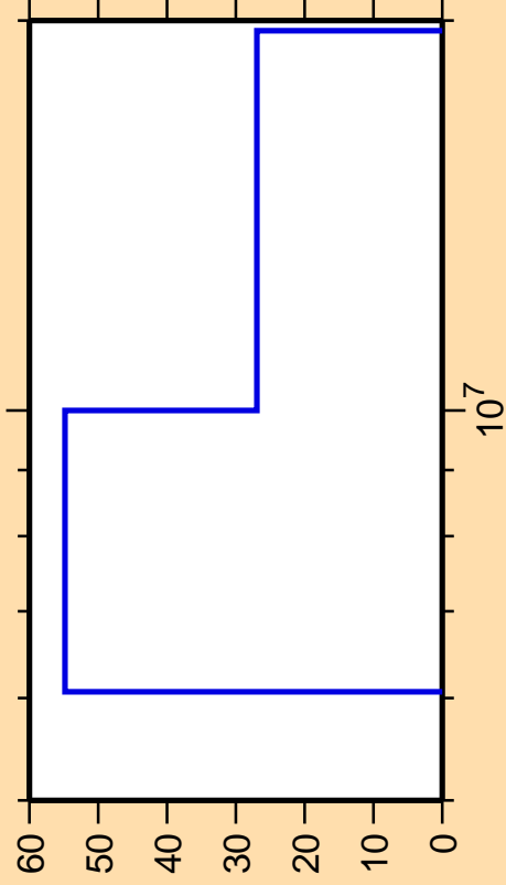
\Delta\sigma/\sigma vs. E for ^{205}\text{Po}(n,p)
