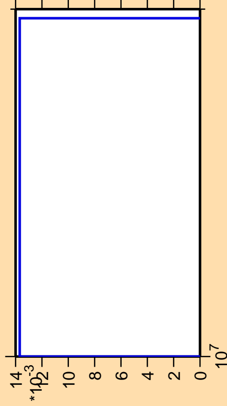
\Delta\sigma/\sigma vs. E for ^{205}\text{Po}(n,3n\alpha)
