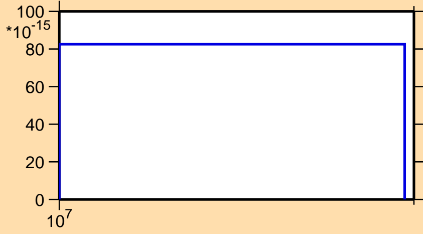
\sigma vs. E for ^{205}\text{Po}(\text{mt117})
