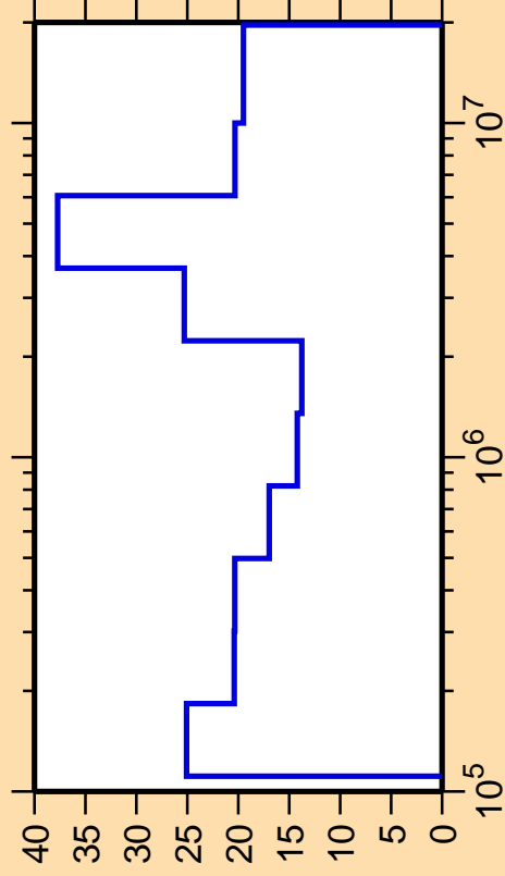
\Delta\sigma/\sigma vs. E for ^{205}\text{Po}(n,n_2)
