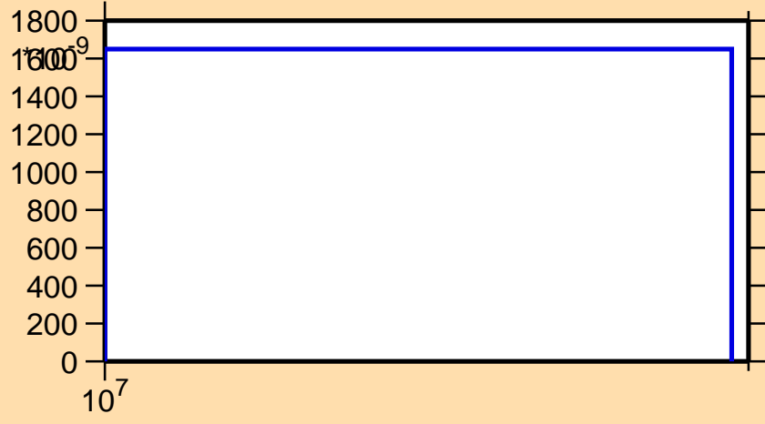
\sigma vs. E for ^{205}\text{Po}(n,2np)
