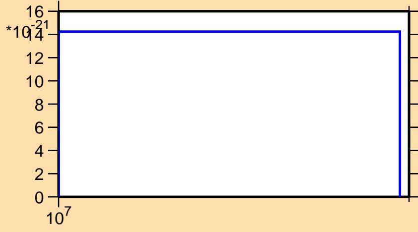
\sigma vs. E for ^{205}\text{Po} (mt 11)
