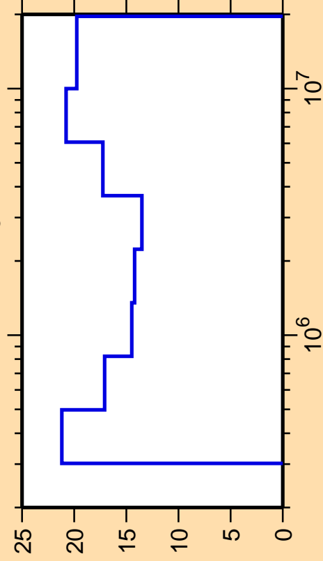
\Delta\sigma/\sigma vs. E for ^{205}\text{Po}(n,n_3)
