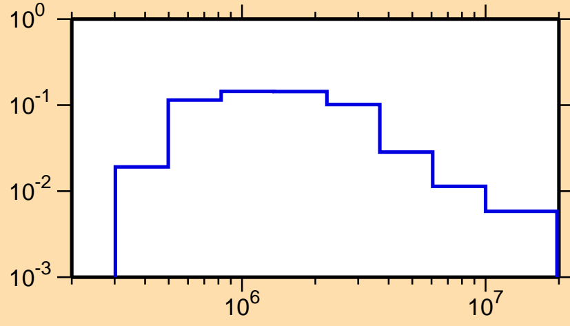
\sigma vs. E for ^{205}\text{Po}(n,n_3)
