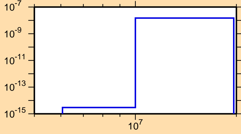
\sigma vs. E for ^{205}\text{Po}(n,\text{He}3)
