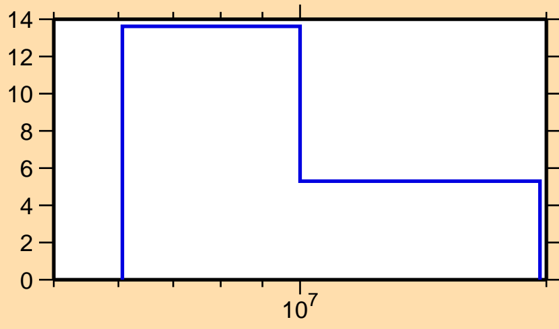
\Delta\sigma/\sigma vs. E for ^{205}\text{Po}(n,2n)
