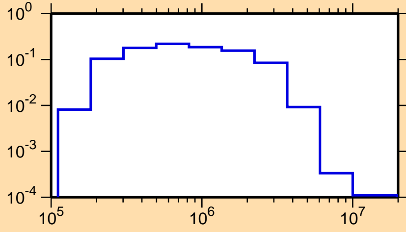
\sigma vs. E for ^{205}\text{Po}(n,n_2)
