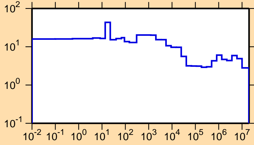
\Delta\sigma/\sigma vs. E for ^{205}\text{Po}(n,\text{el.})
