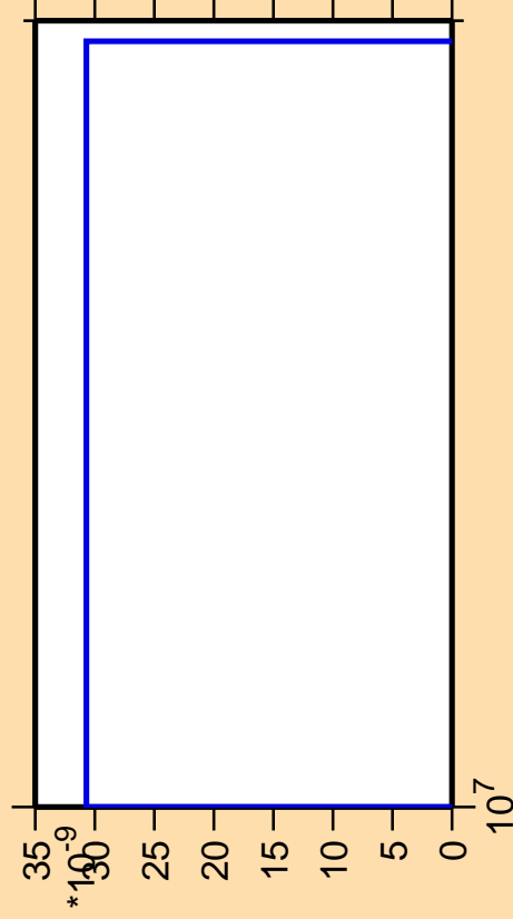
\Delta\sigma/\sigma vs. E for ^{205}\text{Po} (mt 11)
