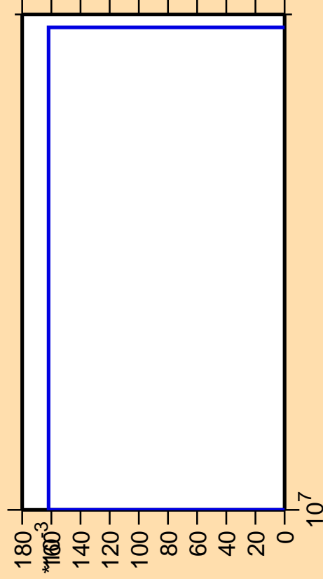
\Delta\sigma/\sigma vs. E for ^{205}\text{Po}(\text{mt117})
