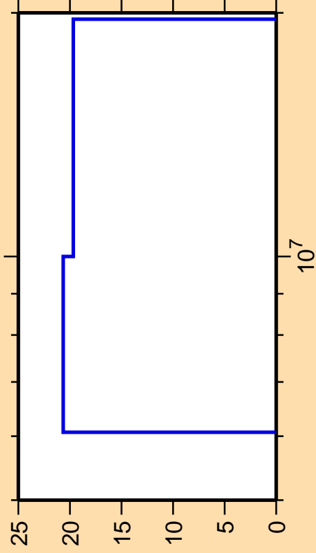
\Delta\sigma/\sigma vs. E for ^{205}\text{Po}(n,n_1)
