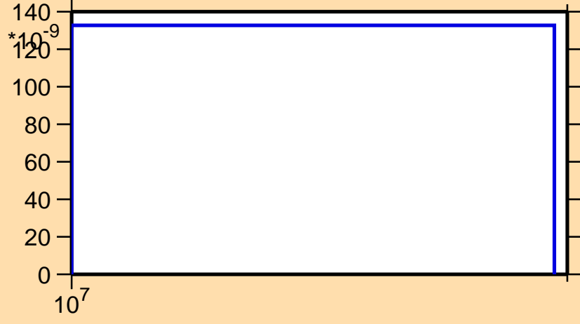
\sigma vs. E for ^{205}\text{Po}(n,\text{nd})
