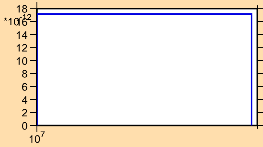
\sigma vs. E for ^{205}\text{Po}(n,\text{pd})
