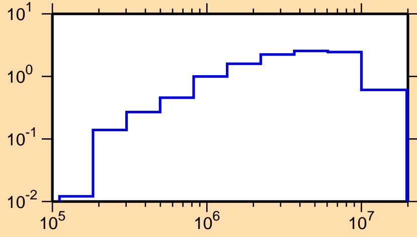
\sigma vs. E for ^{205}\text{Po}(n,\text{inel.})
