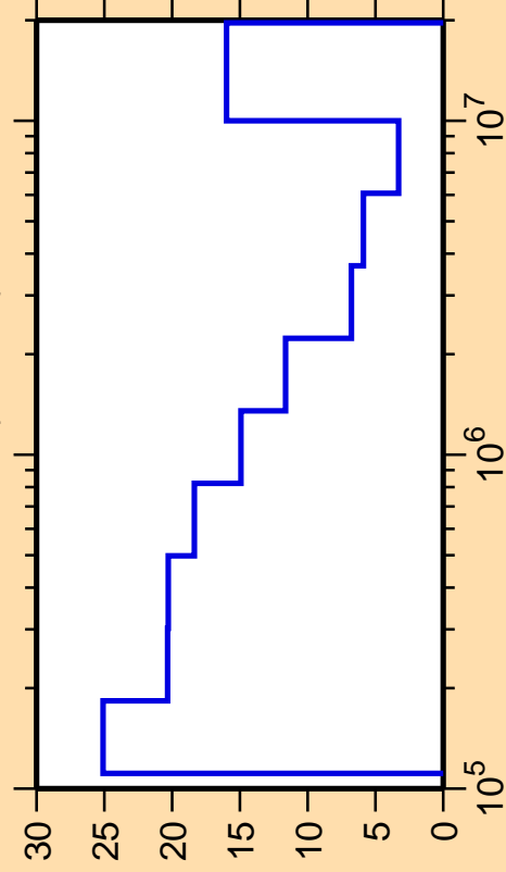
\Delta\sigma/\sigma vs. E for ^{205}\text{Po}(n,\text{inel.})
