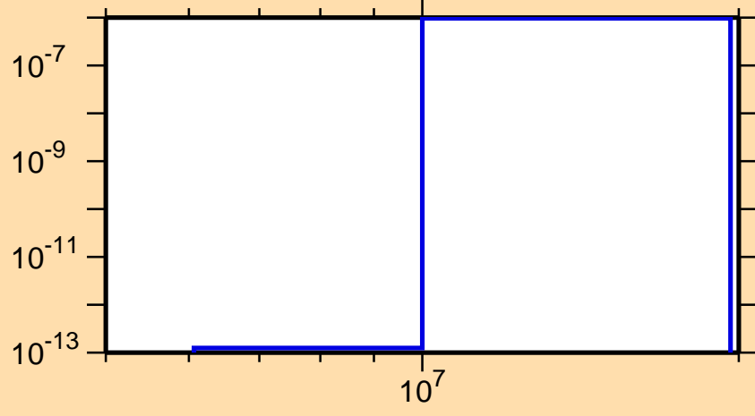
\sigma vs. E for ^{205}\text{Po}(n,2n\alpha)
