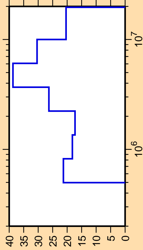
\Delta\sigma/\sigma vs. E for ^{205}\text{Po}(n,n_4)
