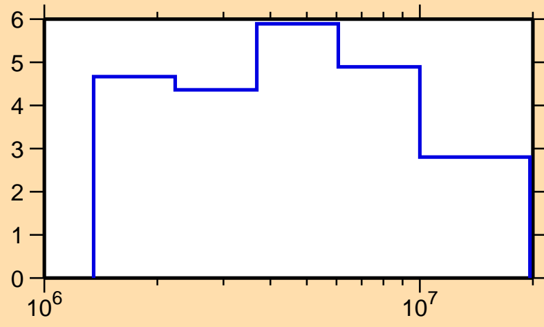
\Delta\sigma/\sigma vs. E for ^{205}\text{Po}(n, el.)
