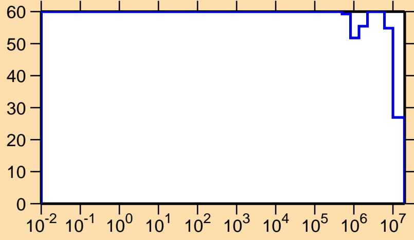
\Delta\sigma/\sigma vs. E for ^{205}\text{Po}(n,p)
