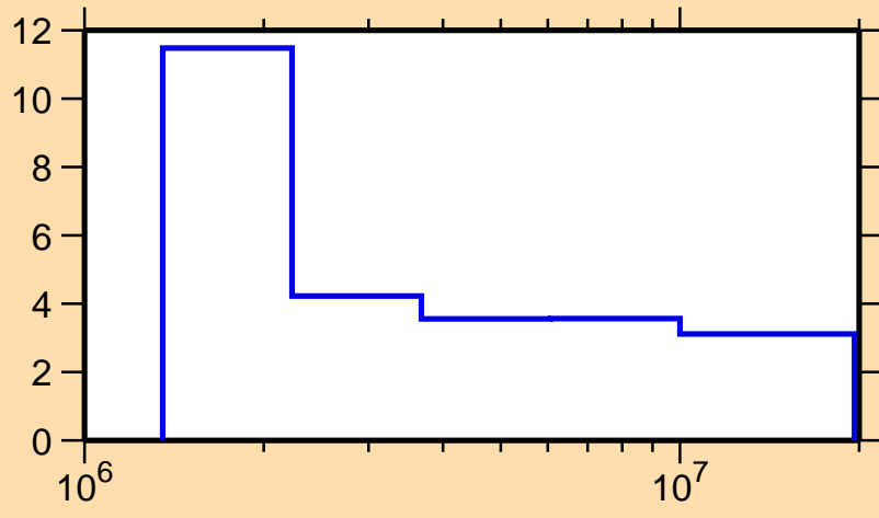
\Delta\sigma/\sigma vs. E for ^{205}\text{Po}(n,\text{nonel.})
