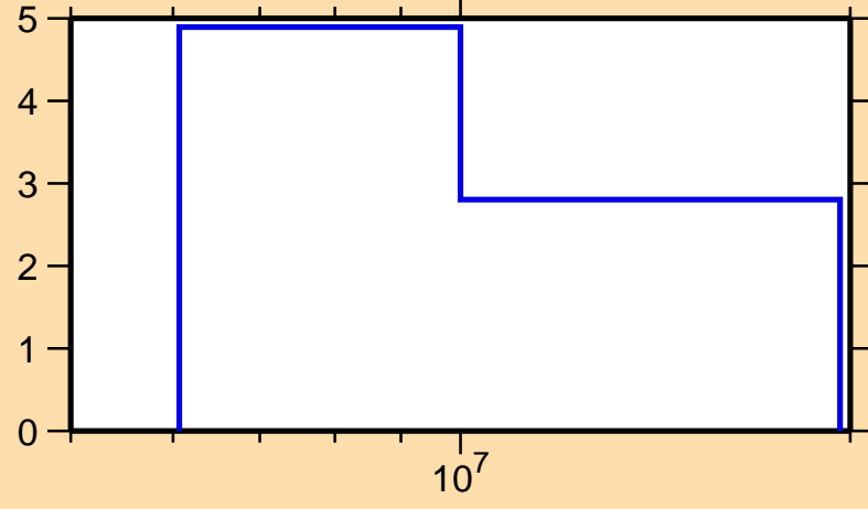
\Delta\sigma/\sigma vs. E for ^{205}\text{Po}(n,\text{el.})
