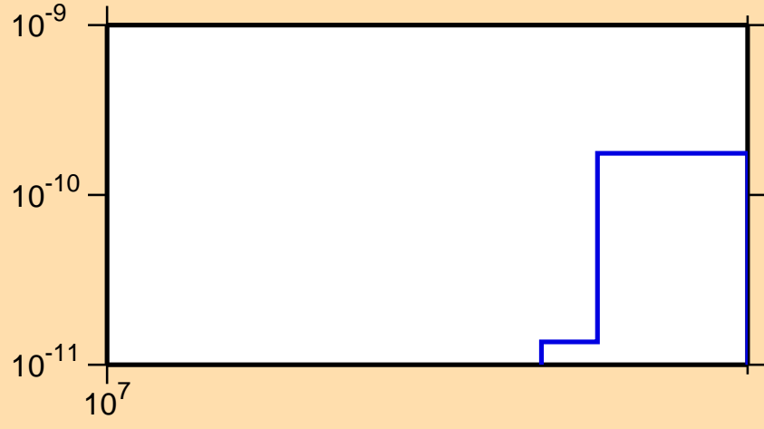
\sigma vs. E for ^{207}\text{Po}(n,\text{pd})
