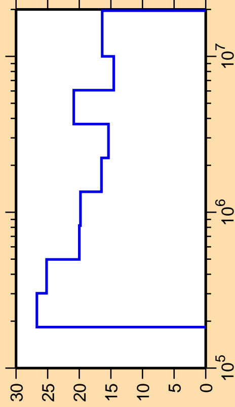
\Delta\sigma/\sigma vs. E for ^{207}\text{Po}(n,n_2)
