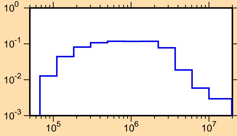
\sigma vs. E for ^{207}\text{Po}(n,n_1)
