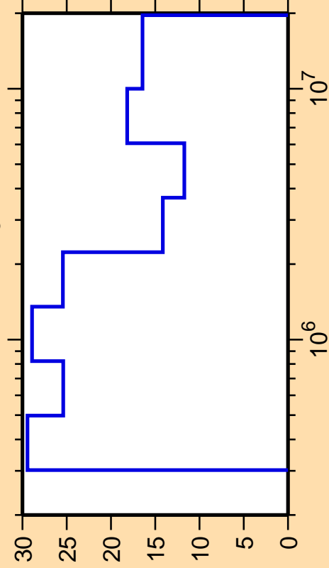
\Delta\sigma/\sigma vs. E for ^{207}\text{Po}(n,n_3)
