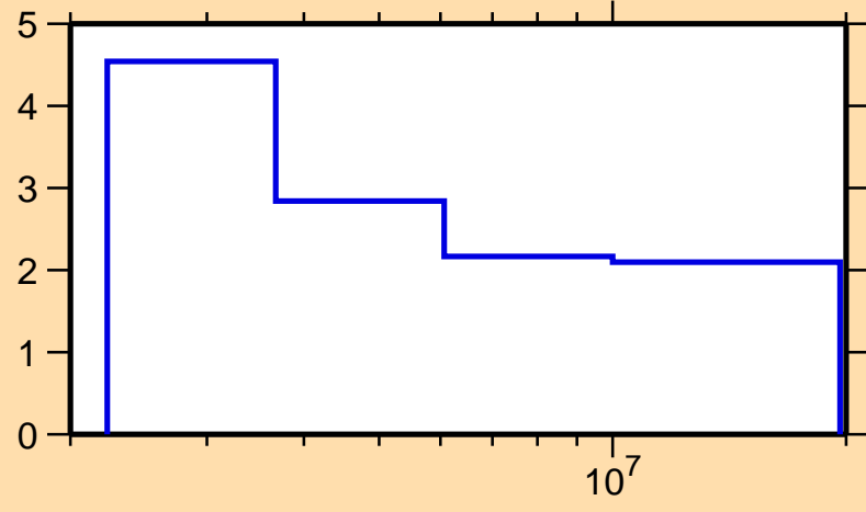
\Delta\sigma/\sigma vs. E for ^{207}\text{Po}(n,n\text{onel.})
