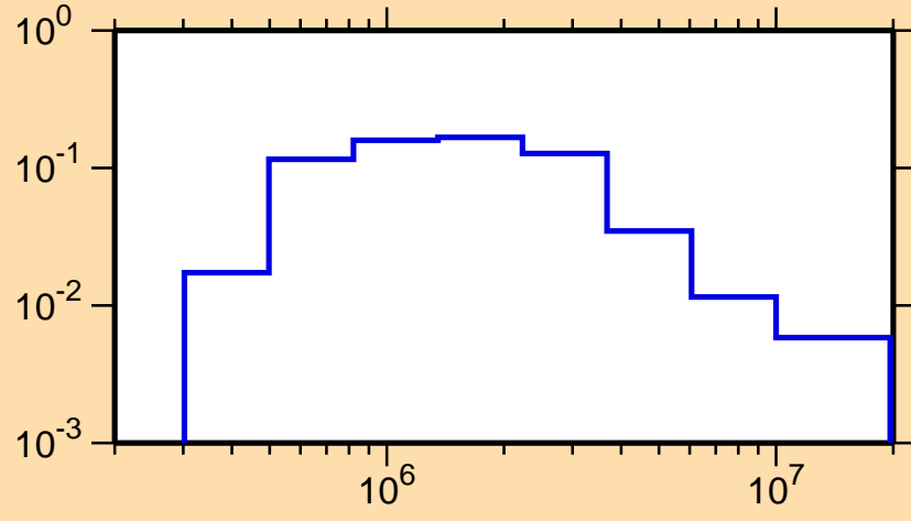
\sigma vs. E for ^{207}\text{Po}(n,n_3)
