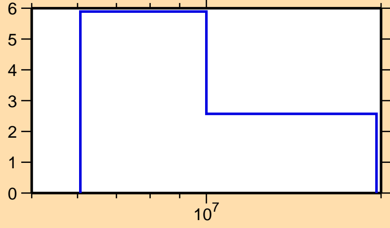
\Delta\sigma/\sigma vs. E for ^{207}\text{Po}(n,2n)
