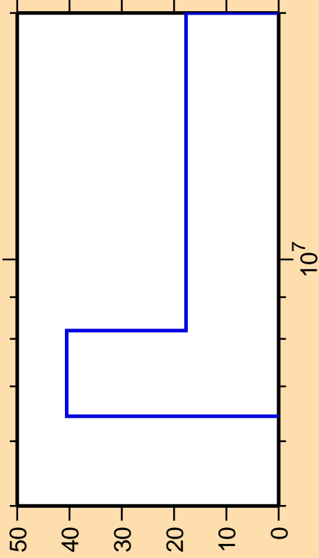
\Delta\sigma/\sigma vs. E for ^{207}\text{Po}(n,p)
