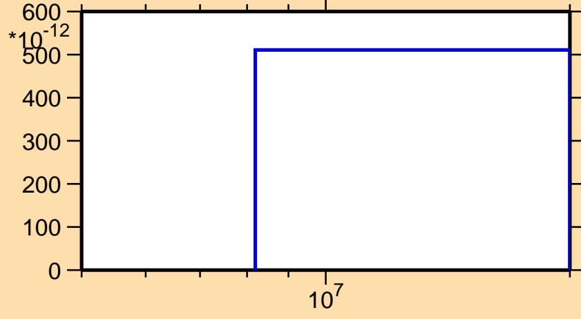
\sigma vs. E for ^{207}\text{Po}(n,nt)
