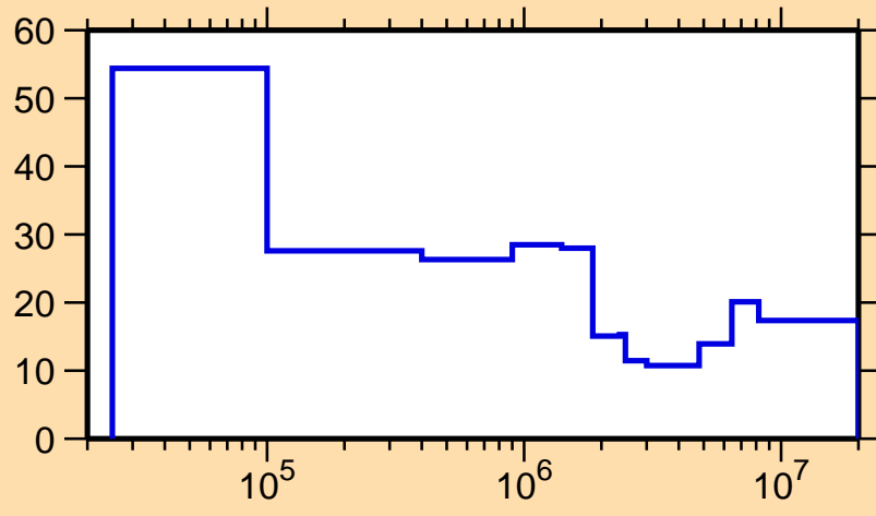
\Delta\sigma/\sigma vs. E for ^{207}\text{Po}(n,n_1)
