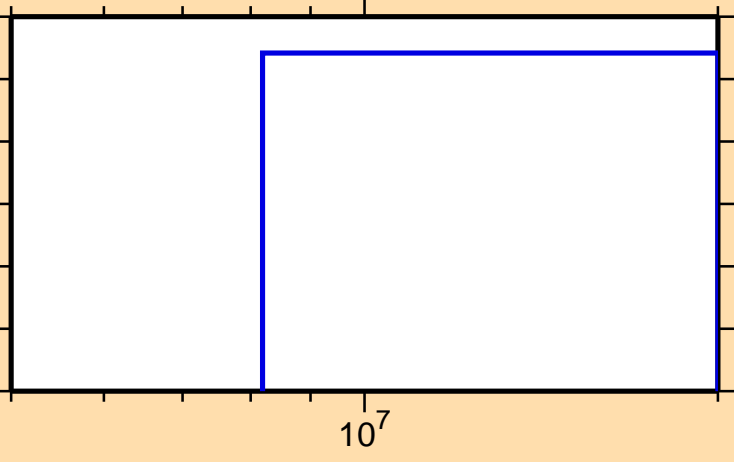
\sigma vs. E for ^{207}\text{Po}(\text{mt117})
