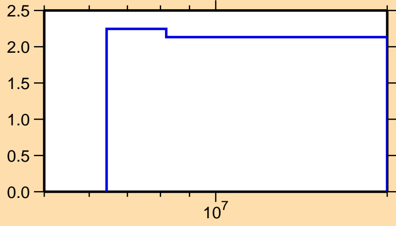
\Delta\sigma/\sigma vs. E for ^{207}\text{Po}(n,\text{nonel.})
