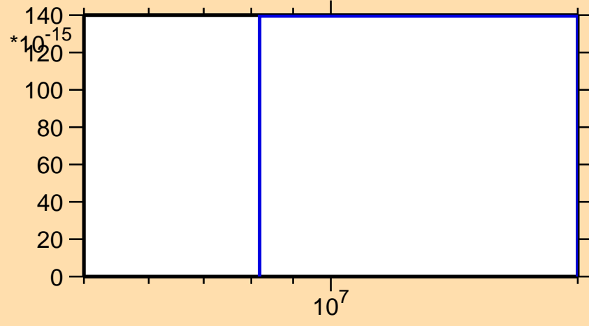
\sigma vs. E for ^{207}\text{Po}(\text{mt } 34)
