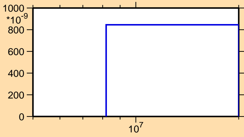
\sigma vs. E for ^{207}\text{Po}(n,2np)
