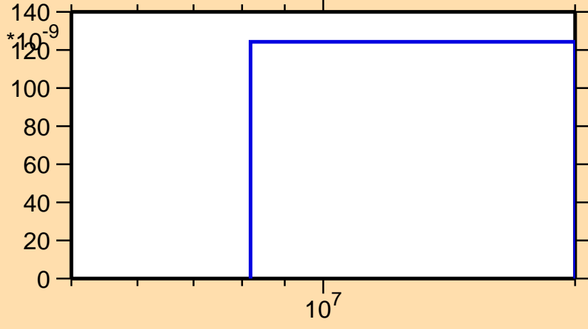
\sigma vs. E for ^{207}\text{Po}(n,\text{nd})
