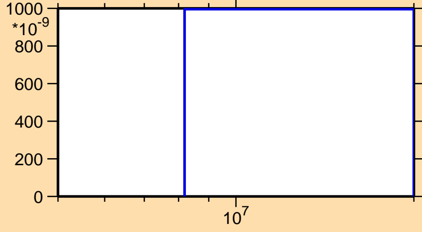
\sigma vs. E for ^{207}\text{Po}(n,2n\alpha)
