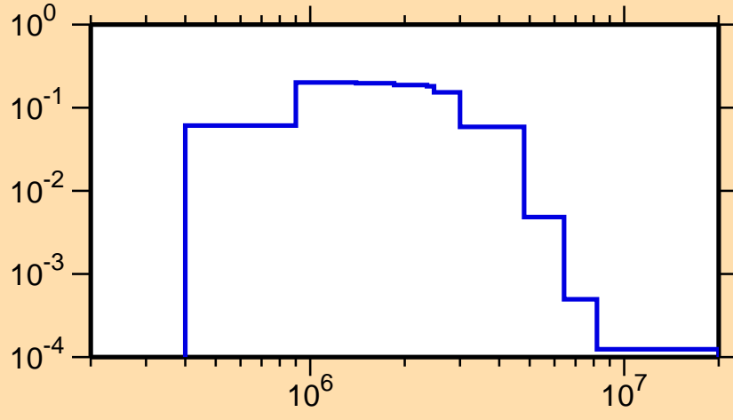
\sigma vs. E for ^{207}\text{Po}(n,n_4)
