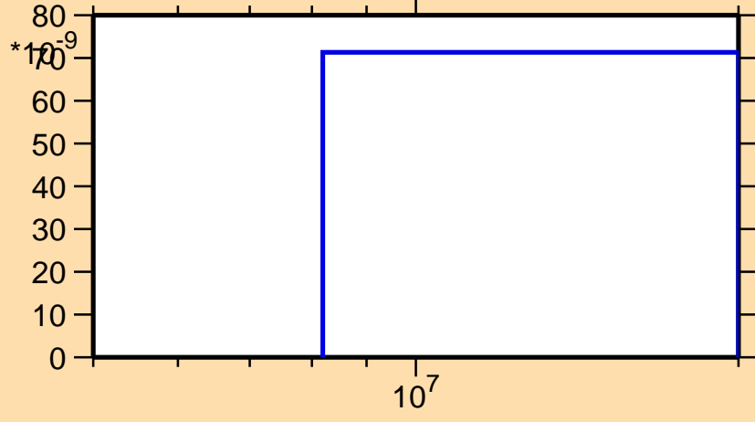
\sigma vs. E for ^{207}\text{Po}(n,p\alpha)
