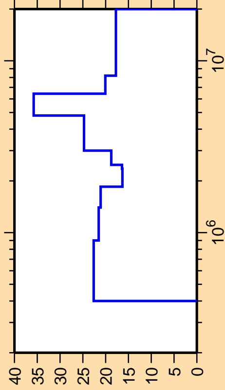
\Delta\sigma/\sigma vs. E for ^{207}\text{Po}(n,n_4)
