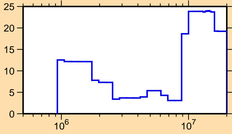
\Delta\sigma/\sigma vs. E for ^{207}\text{Po}(n,n\text{cont.})
