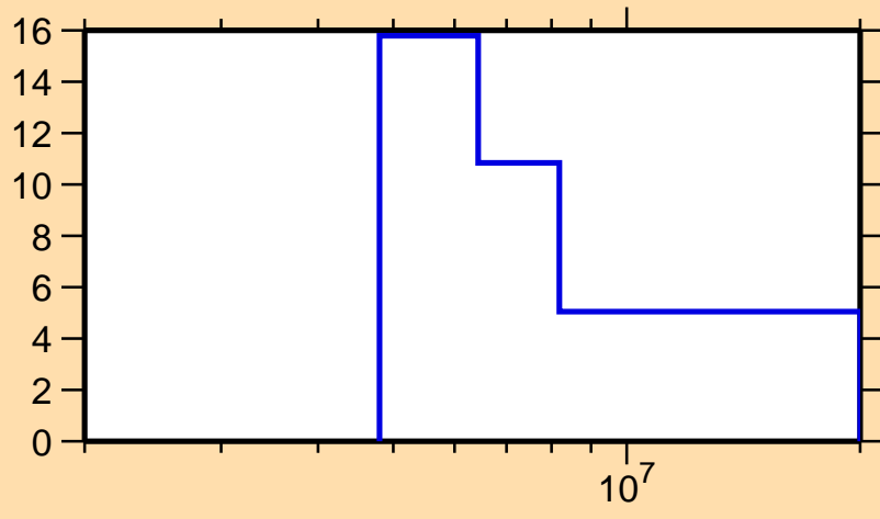
\Delta\sigma/\sigma vs. E for ^{207}\text{Po}(n,2n)
