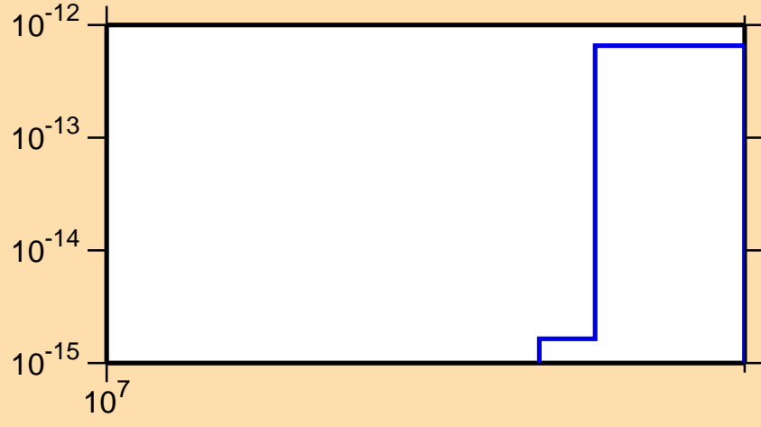
\sigma vs. E for ^{208}\text{Po} (mt 34)
