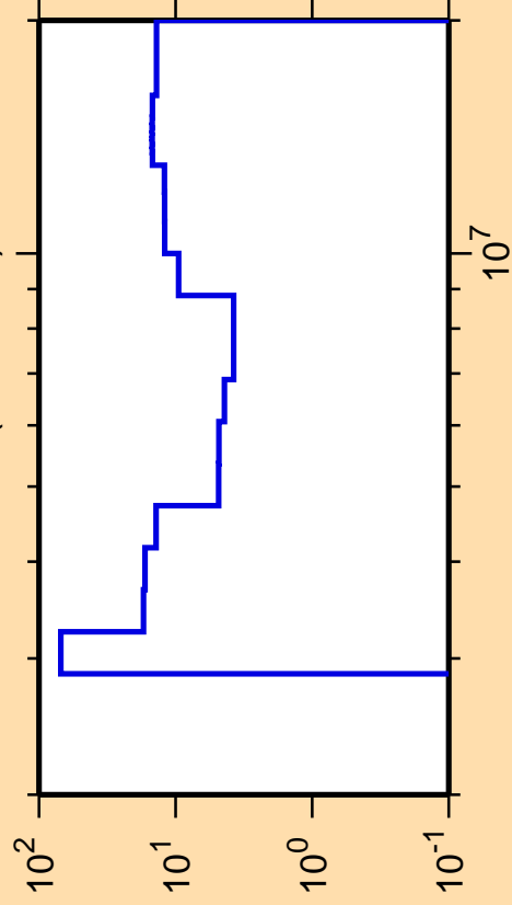
\Delta\sigma/\sigma vs. E for ^{208}\text{Po}(n,\text{ncont.})
