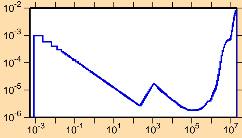
\sigma vs. E for ^{208}\text{Po}(n,\alpha)
