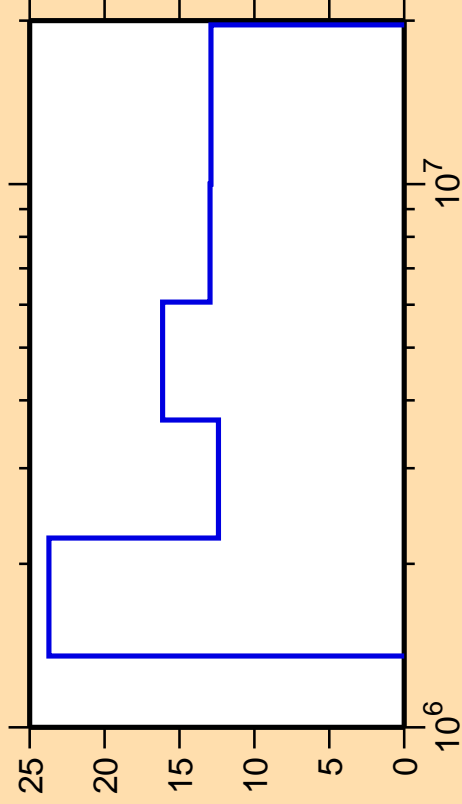
\Delta\sigma/\sigma vs. E for ^{208}\text{Po}(n,n_4)
