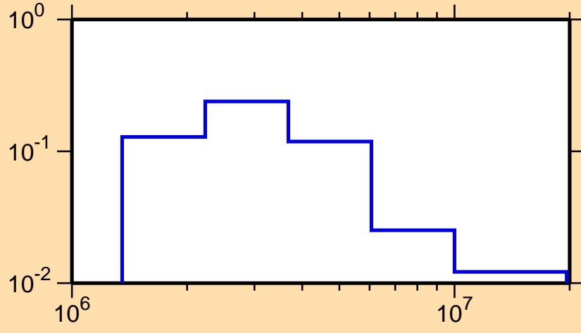
\sigma vs. E for ^{208}\text{Po}(n,n_4)
