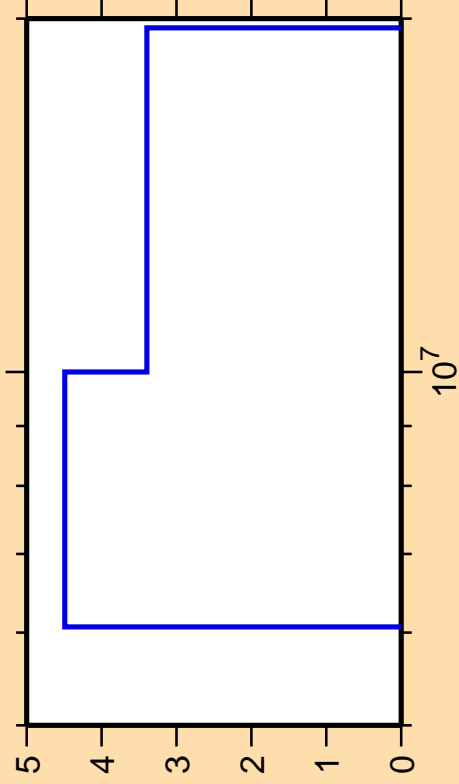
\Delta\sigma/\sigma vs. E for ^{208}\text{Po}(n,2n)
