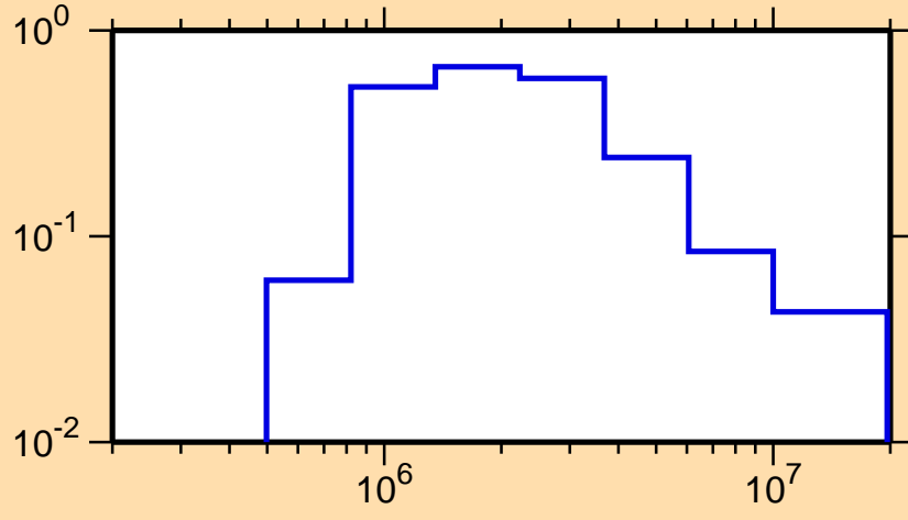
\sigma vs. E for ^{208}\text{Po}(n,n_1)
