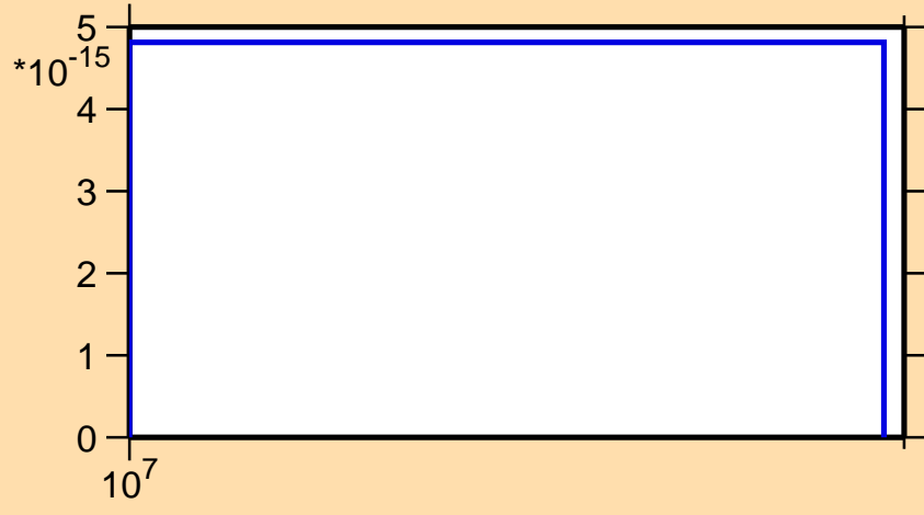
\sigma vs. E for ^{208}\text{Po} (mt 34)
