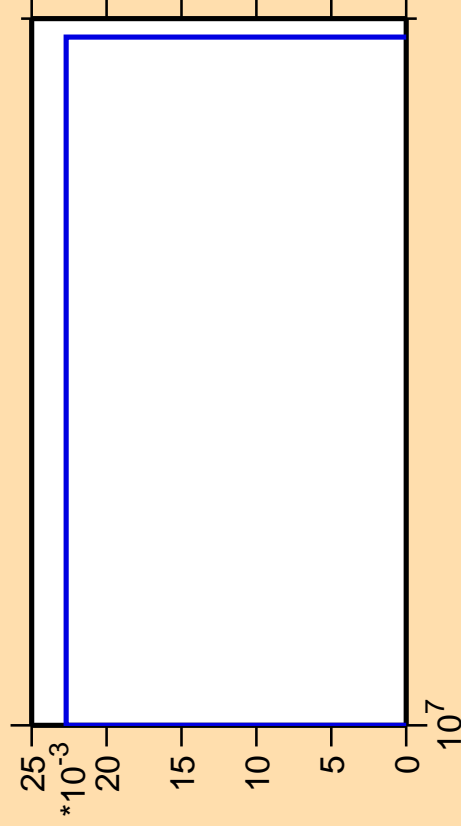
\Delta\sigma/\sigma vs. E for ^{208}\text{Po} (mt 34)
