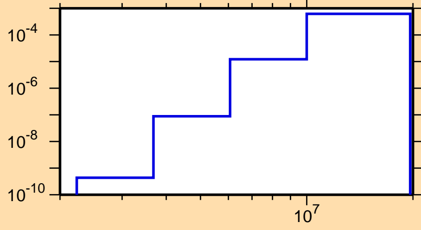
\sigma vs. E for ^{208}\text{Po}(n,n\alpha)
