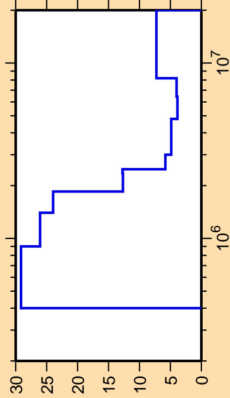
\Delta\sigma/\sigma vs. E for ^{208}\text{Po}(n,\text{inel.})
