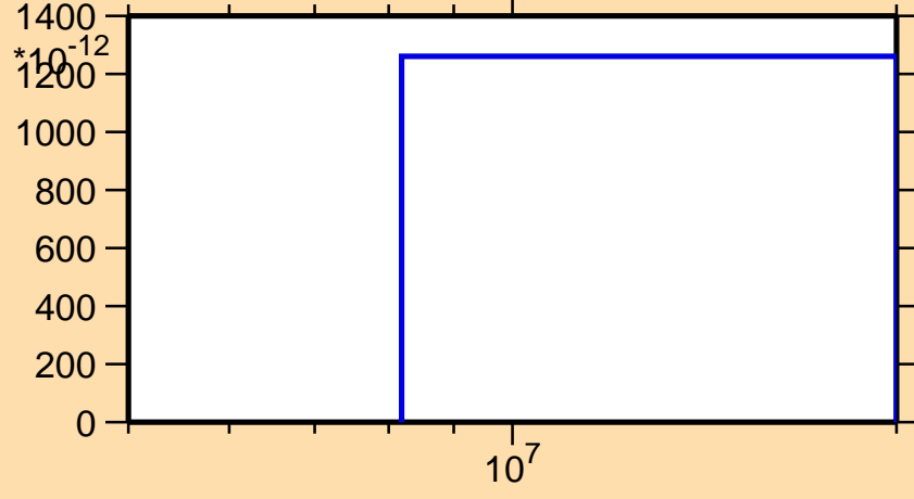
\sigma vs. E for ^{208}\text{Po}(n,\text{He}3)
