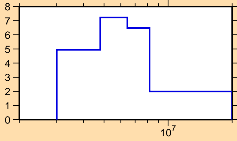
\Delta\sigma/\sigma vs. E for ^{208}\text{Po}(n, \text{el.})
