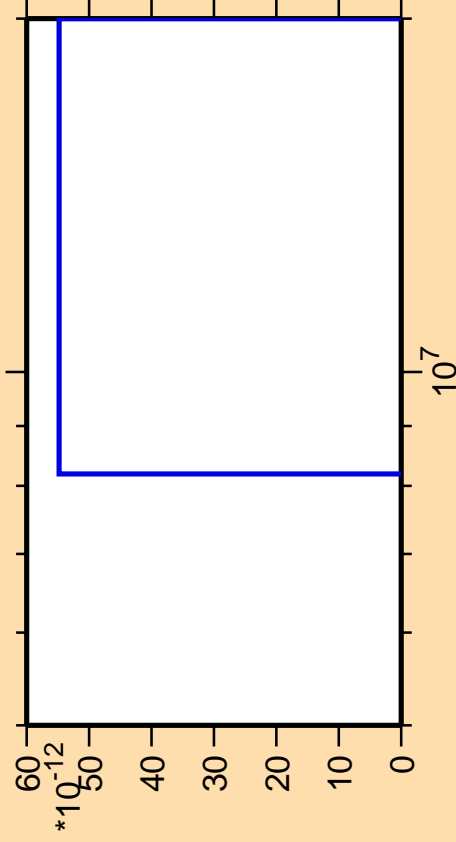
\Delta\sigma/\sigma vs. E for ^{208}\text{Po} (mt 42)
