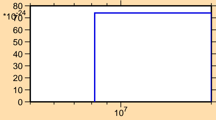
\sigma vs. E for ^{208}\text{Po} (mt 42)
