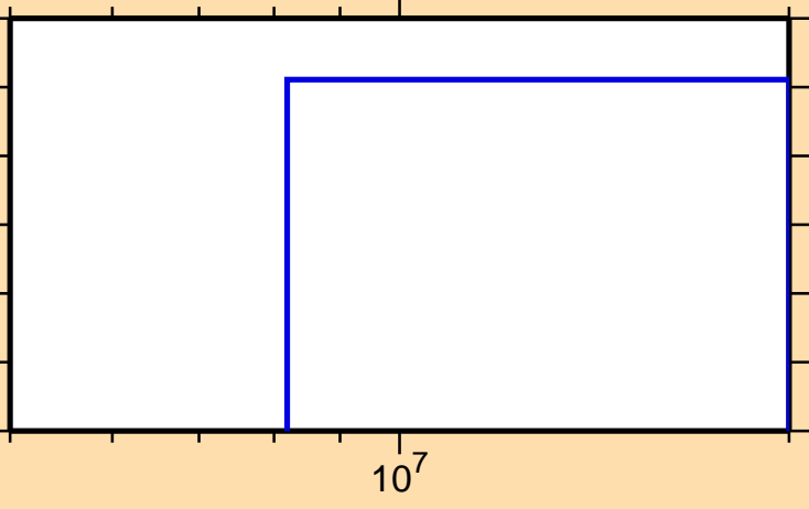
\sigma vs. E for ^{208}\text{Po}(n,3n\alpha)
