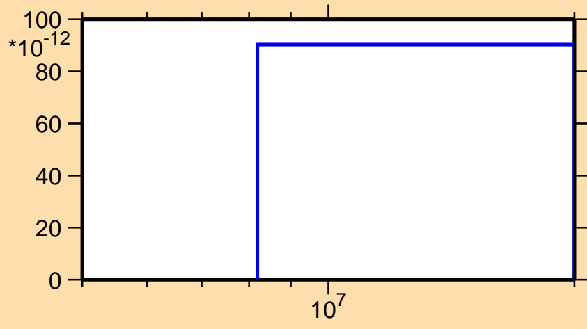
\sigma vs. E for ^{208}\text{Po}(n,p\alpha)
