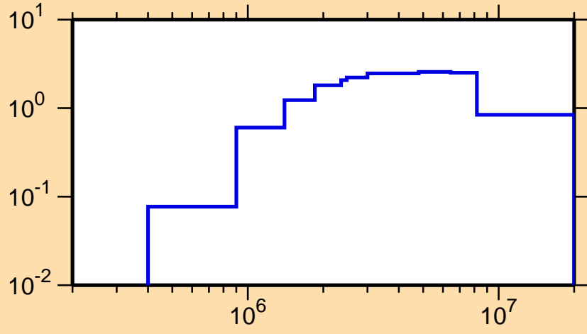
\sigma vs. E for ^{208}\text{Po}(n,\text{inel.})
