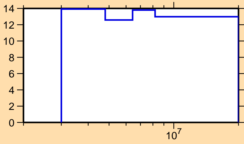
\Delta\sigma/\sigma vs. E for ^{208}\text{Po}(n, n_1)
