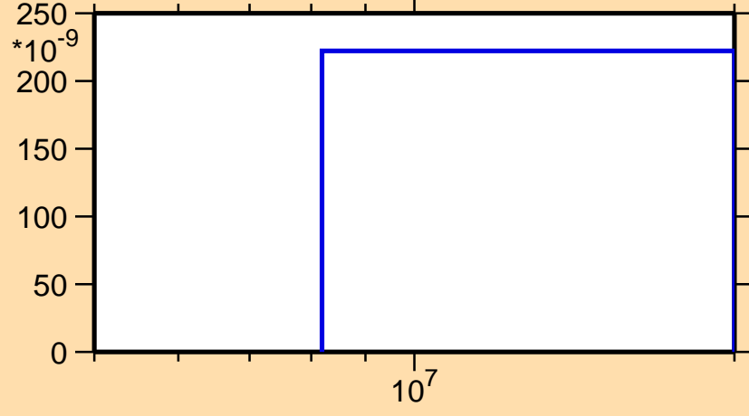
\sigma vs. E for ^{208}\text{Po}(n,2n\alpha)
