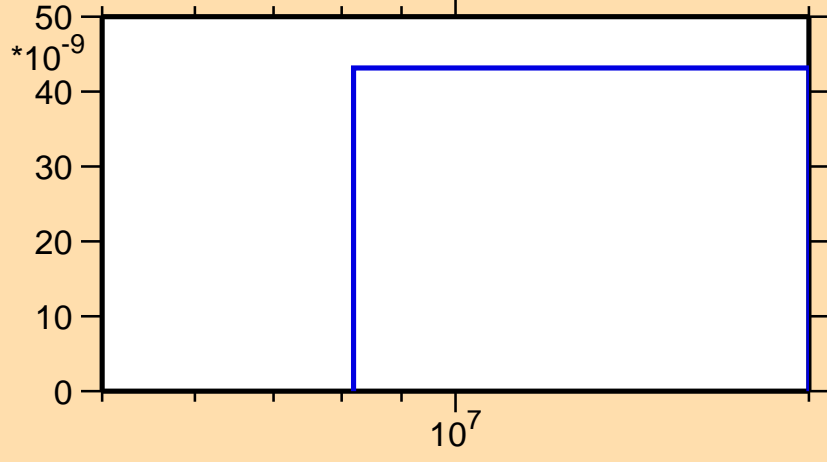
\sigma vs. E for ^{208}\text{Po}(n,2np)
