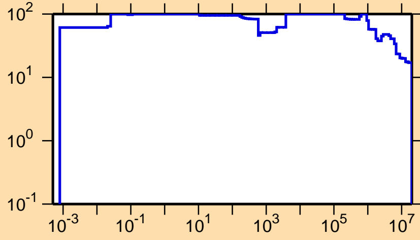
\Delta\sigma/\sigma vs. E for ^{209}\text{Po}(n,p)
