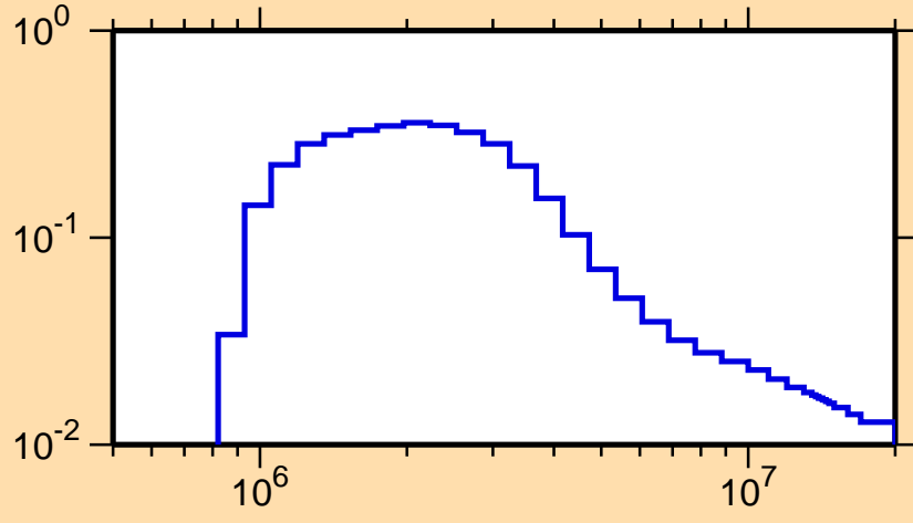
\sigma vs. E for ^{209}\text{Po}(n,n_2)
