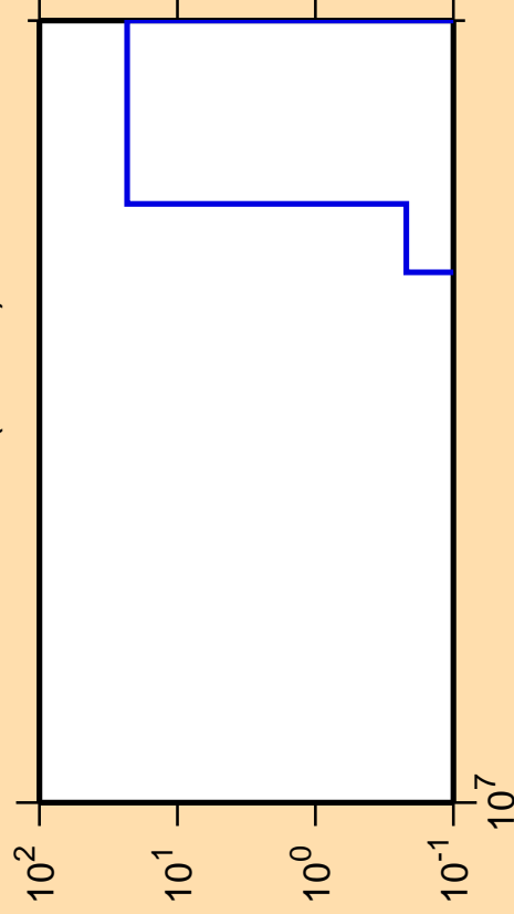
\Delta\sigma/\sigma vs. E for ^{209}\text{Po}(\text{mt } 34)
