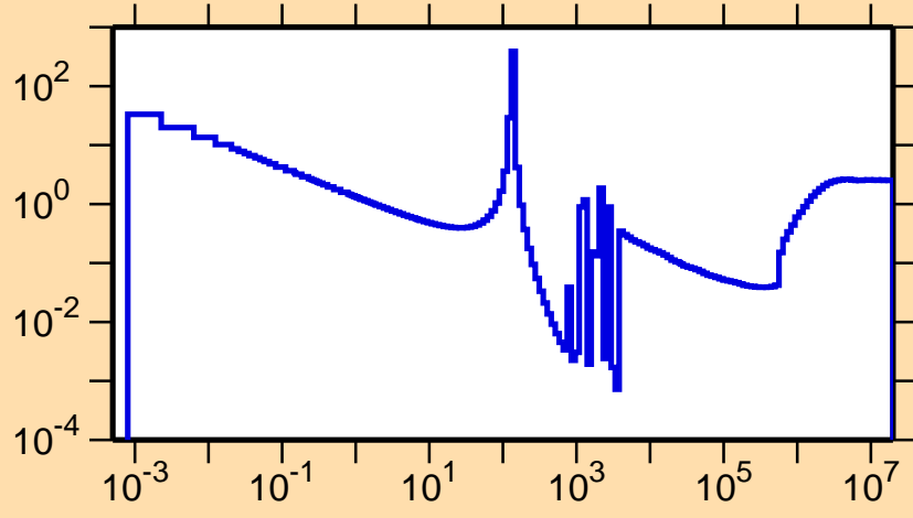
\sigma vs. E for ^{209}\text{Po}(n,\text{nonel.})
