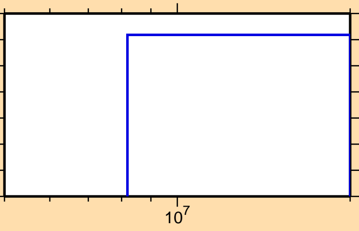
\sigma vs. E for ^{209}\text{Po}(n,3n\alpha)
