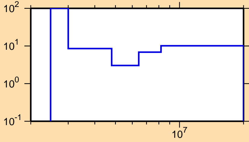
\Delta\sigma/\sigma vs. E for ^{209}\text{Po}(n,n\text{cont.})
