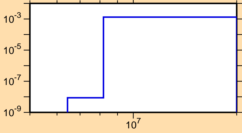
\sigma vs. E for ^{209}\text{Po}(n,np)
