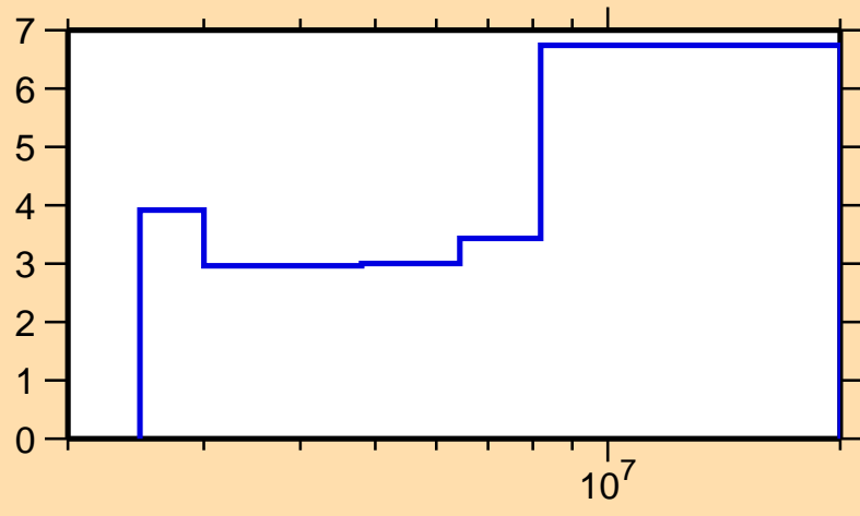
\Delta\sigma/\sigma vs. E for ^{210}\text{Po}(n,\text{inel.})
