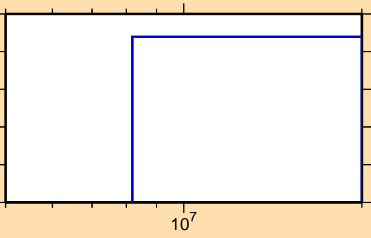
\sigma vs. E for ^{210}\text{Po}(n,nt)
