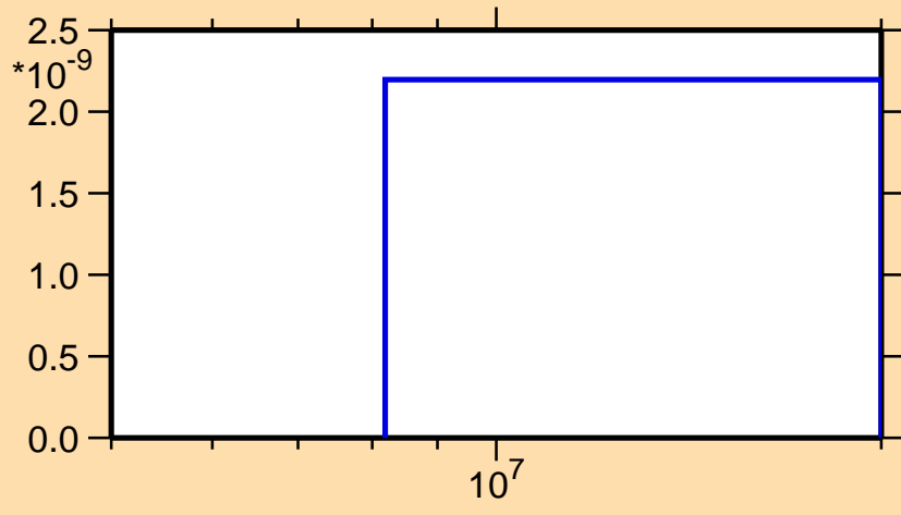
\sigma vs. E for ^{210}\text{Po}(n,nt)
