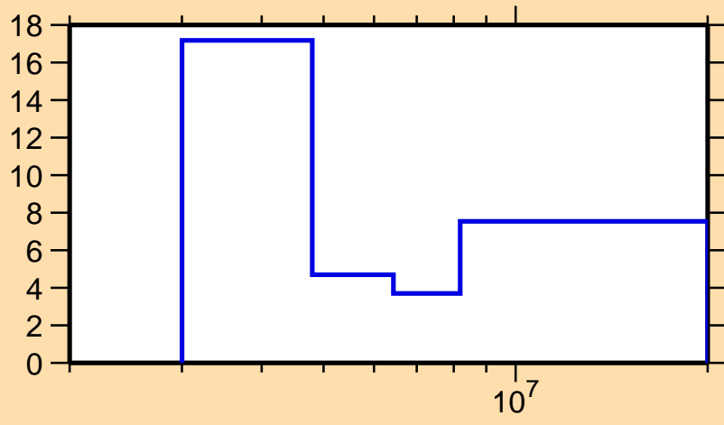
\Delta\sigma/\sigma vs. E for ^{210}\text{Po}(n,n\text{cont.})
