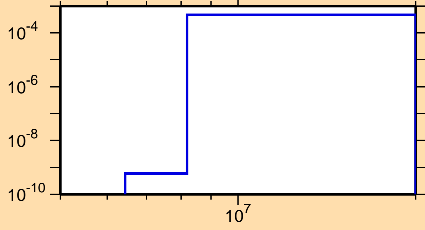
\sigma vs. E for ^{210}\text{Po}(n,d)
