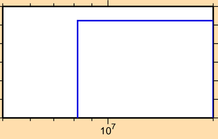
\sigma vs. E for ^{211}\text{Po}(\text{mt } 42)
