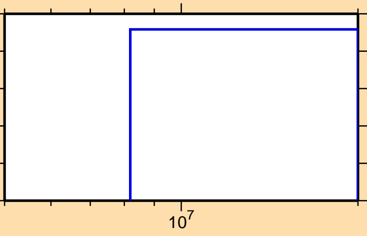
\sigma vs. E for ^{211}\text{Po}(n,\text{pd})
