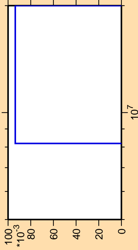
\Delta\sigma/\sigma vs. E for ^{211}\text{Po}(\text{mt } 42)
