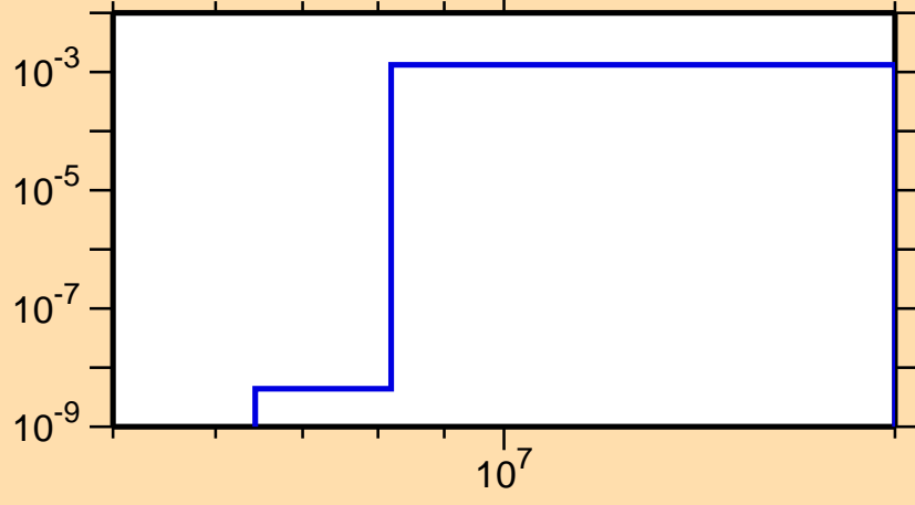
\sigma vs. E for ^{211}\text{Po}(n,np)
