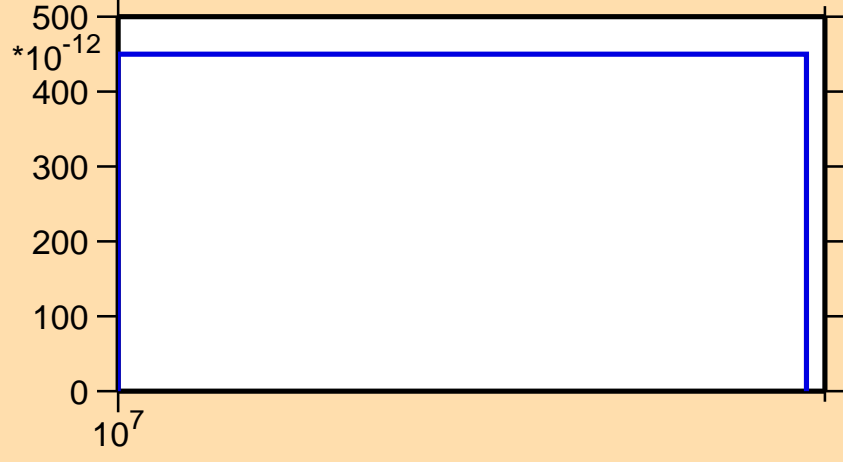
\sigma vs. E for ^{212}\text{Po} (mt 11)
