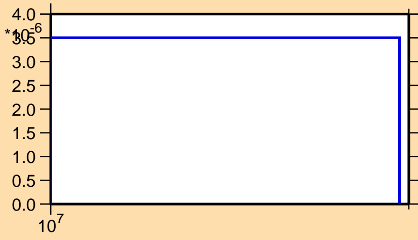
\sigma vs. E for ^{212}\text{Po}(n,2np)
