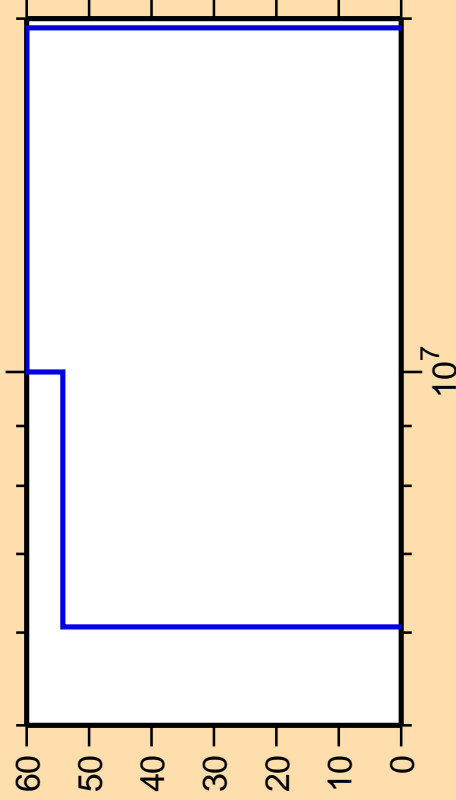
\Delta\sigma/\sigma vs. E for ^{212}\text{Po}(n,p\alpha)
