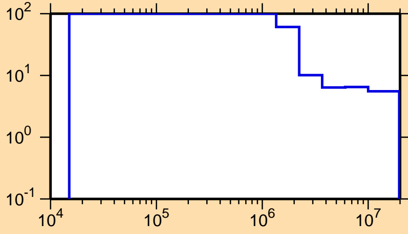
\Delta\sigma/\sigma vs. E for ^{212}\text{Po}(n,\text{nonel.})
