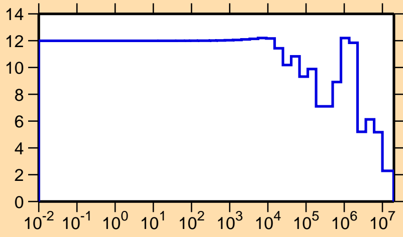
\Delta\sigma/\sigma vs. E for ^{212}\text{Po}(n,\text{el.})
