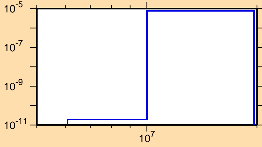
\sigma vs. E for ^{212}\text{Po}(n,p\alpha)
