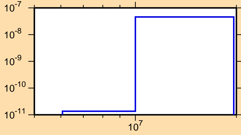
\sigma vs. E for ^{212}\text{Po}(\text{mt } 45)
