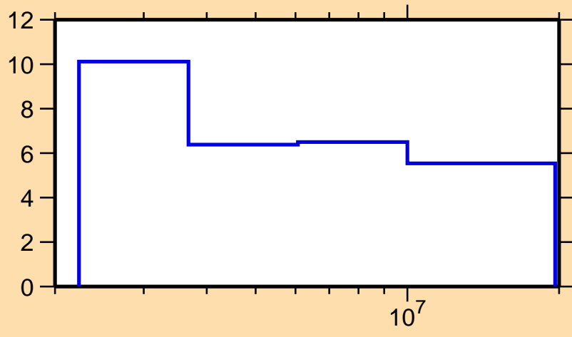
\Delta\sigma/\sigma vs. E for ^{212}\text{Po}(n,\text{nonel.})
