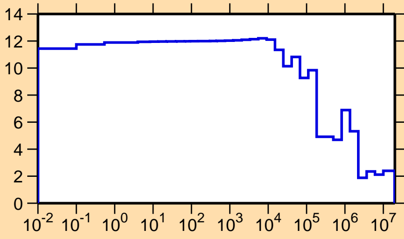
\Delta\sigma/\sigma vs. E for ^{212}\text{Po}(n,\text{tot.})
