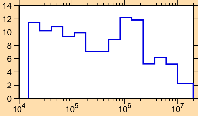
\Delta\sigma/\sigma vs. E for ^{212}\text{Po}(n, el.)
