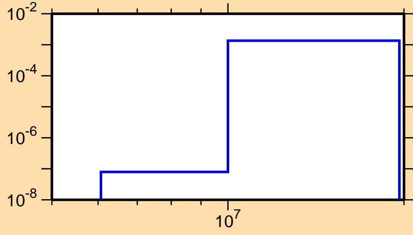
\sigma vs. E for ^{212}\text{Po}(n,np)
