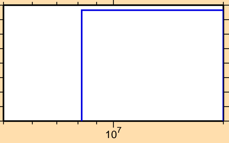
\sigma vs. E for ^{212}\text{Po}(n,nt)
