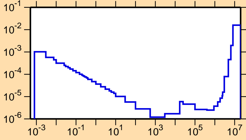
\sigma vs. E for ^{212}\text{Po}(n,\alpha)
