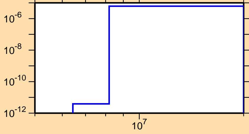
\sigma vs. E for ^{212}\text{Po}(n,p\alpha)
