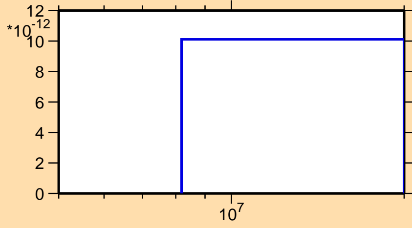
\sigma vs. E for ^{212}\text{Po}(\text{mt } 34)
