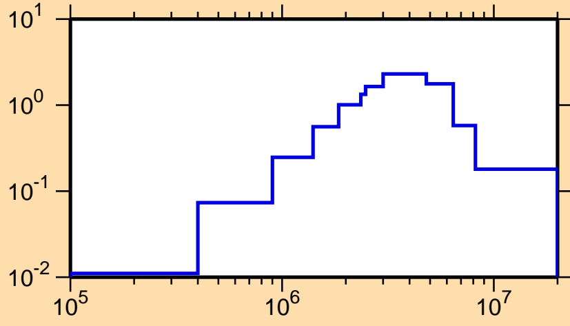
\sigma vs. E for ^{212}\text{Po}(n,\text{inel.})
