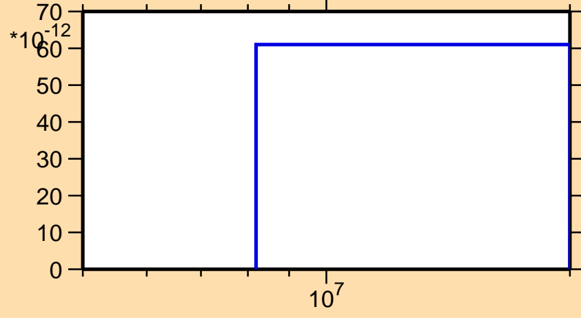
\sigma vs. E for ^{212}\text{Po}(\text{mt } 42)
