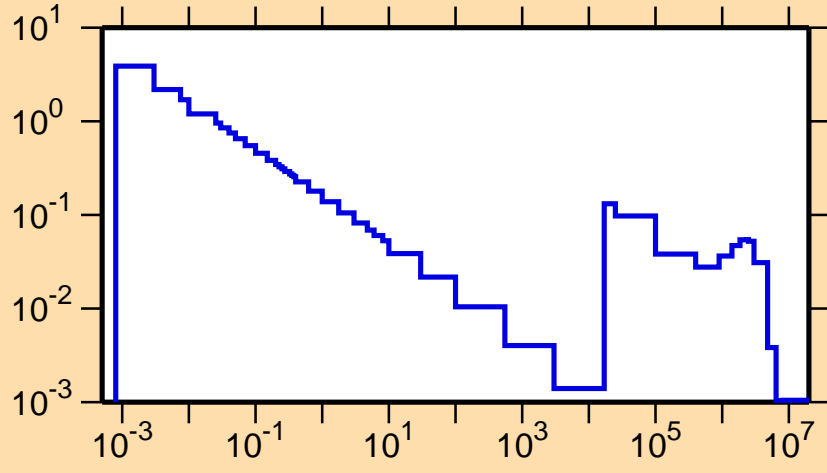
\sigma vs. E for ^{212}\text{Po}(n,\gamma)
