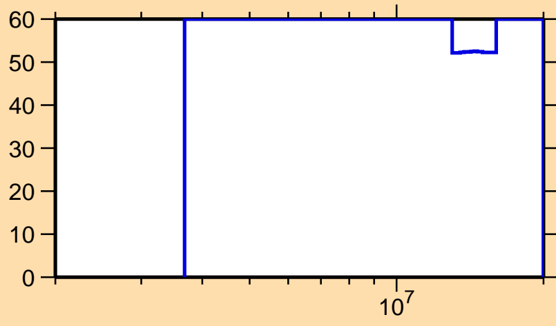
\Delta\sigma/\sigma vs. E for ^{217}\text{Po}(n,2n)
