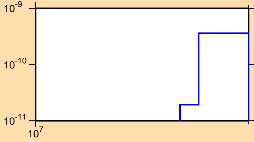
\sigma vs. E for ^{217}\text{Po}(n,\text{He}3)
