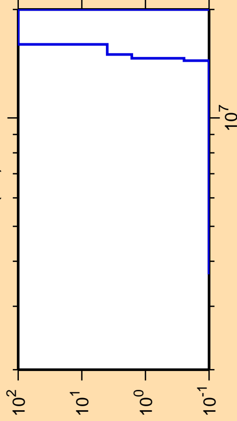
\Delta\sigma/\sigma vs. E for ^{217}\text{Po}(n,f)
