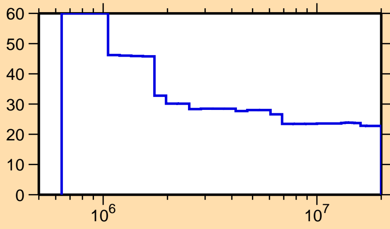
\Delta\sigma/\sigma vs. E for ^{217}\text{Po}(n,\text{nonel.})
