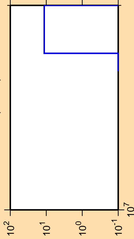
\Delta\sigma/\sigma vs. E for ^{217}\text{Po}(\text{mt } 34)
