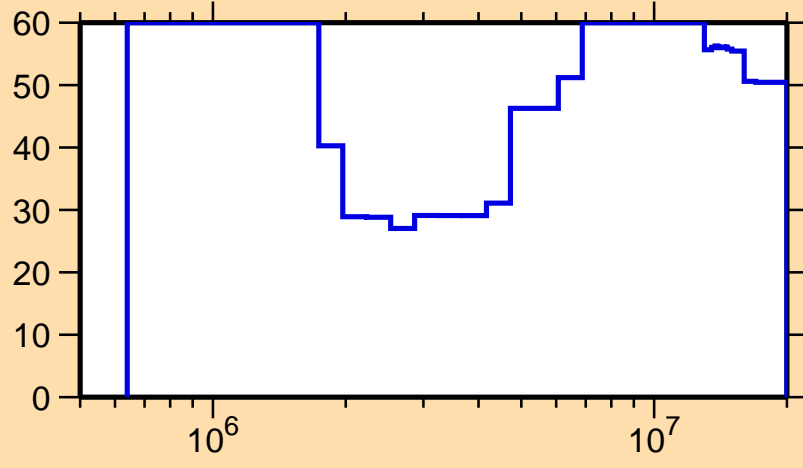
\Delta\sigma/\sigma vs. E for ^{217}\text{Po}(n,\text{tot.})
