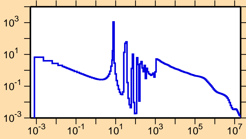
\sigma vs. E for ^{217}\text{Po}(n,\gamma)
