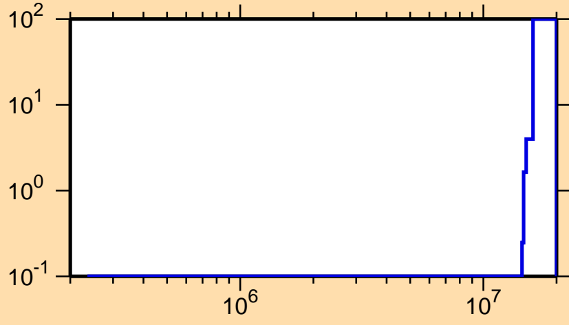
\Delta\sigma/\sigma vs. E for ^{217}\text{Po}(n,f)
