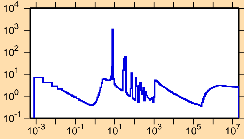
\sigma vs. E for ^{217}\text{Po}(n,\text{nonel.})
