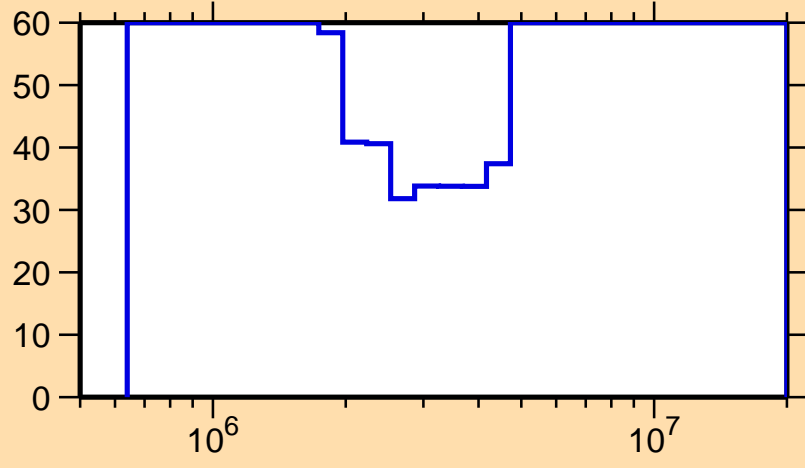
\Delta\sigma/\sigma vs. E for ^{217}\text{Po}(n,\text{el.})
