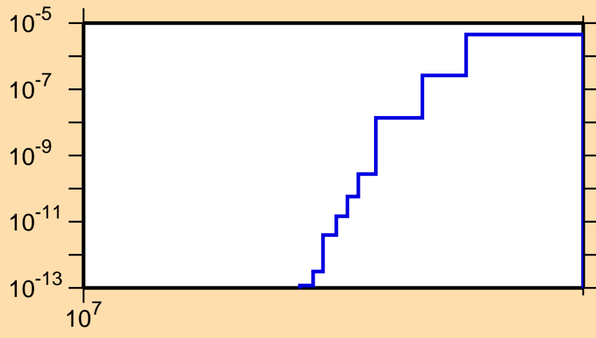
\sigma vs. E for ^{217}\text{Po}(n,2np)
