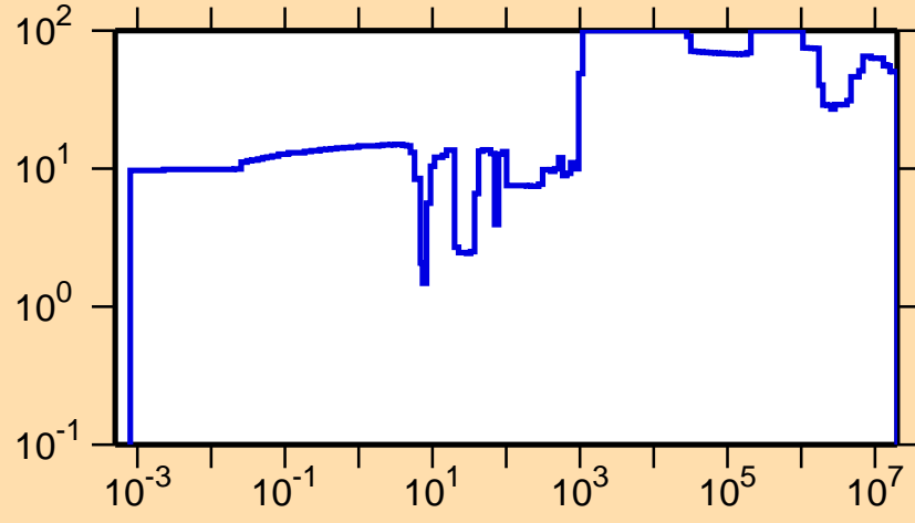
\Delta\sigma/\sigma vs. E for ^{217}\text{Po}(n, \text{tot.})
