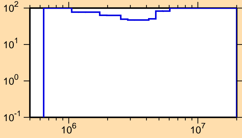
\Delta\sigma/\sigma vs. E for ^{217}\text{Po}(n,n\text{cont.})
