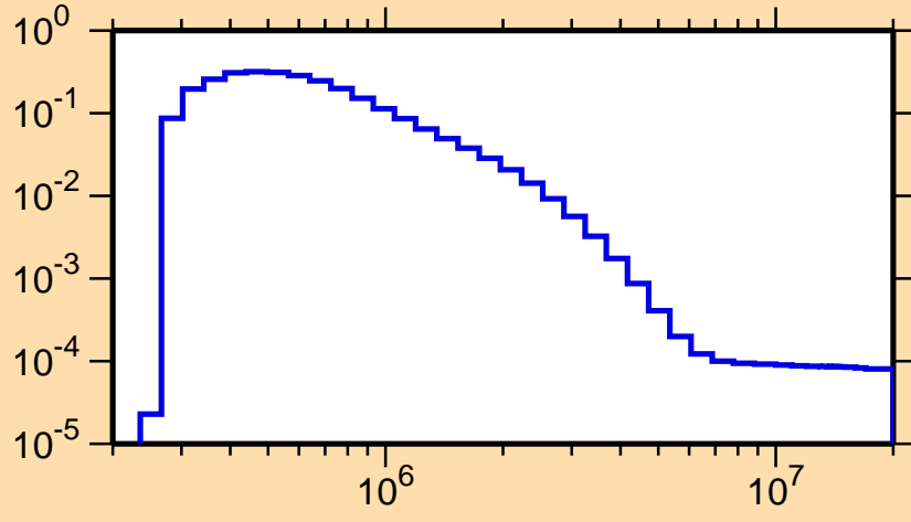
\sigma vs. E for ^{217}\text{Po}(n,n_2)
