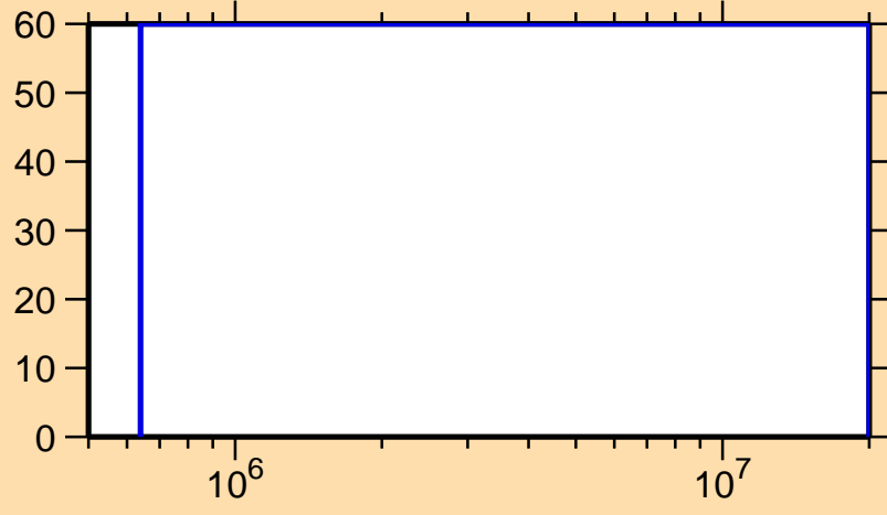
\Delta\sigma/\sigma vs. E for ^{217}\text{Po}(n,n_1)
