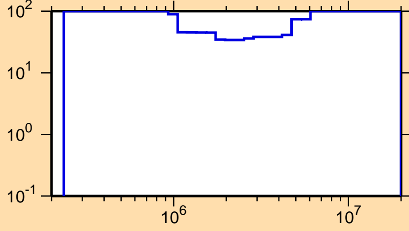
\Delta\sigma/\sigma vs. E for ^{217}\text{Po}(n,\text{inel.})
