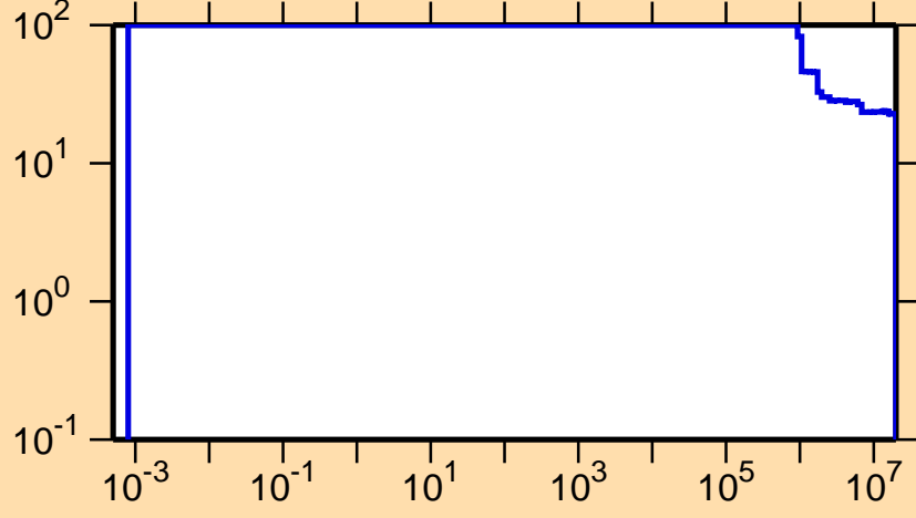
\Delta\sigma/\sigma vs. E for ^{217}\text{Po}(n,\text{nonel.})
