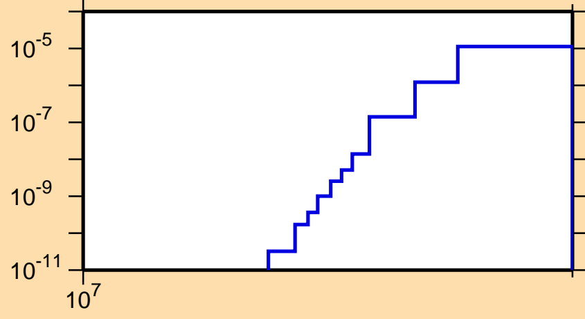
\sigma vs. E for ^{217}\text{Po}(n,\text{nd})
