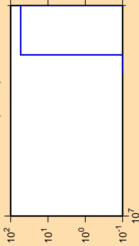
\Delta\sigma/\sigma vs. E for ^{217}\text{Po} (mt 11)
