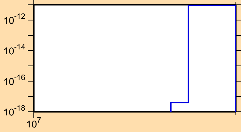
\sigma vs. E for ^{217}\text{Po} (mt 11)
