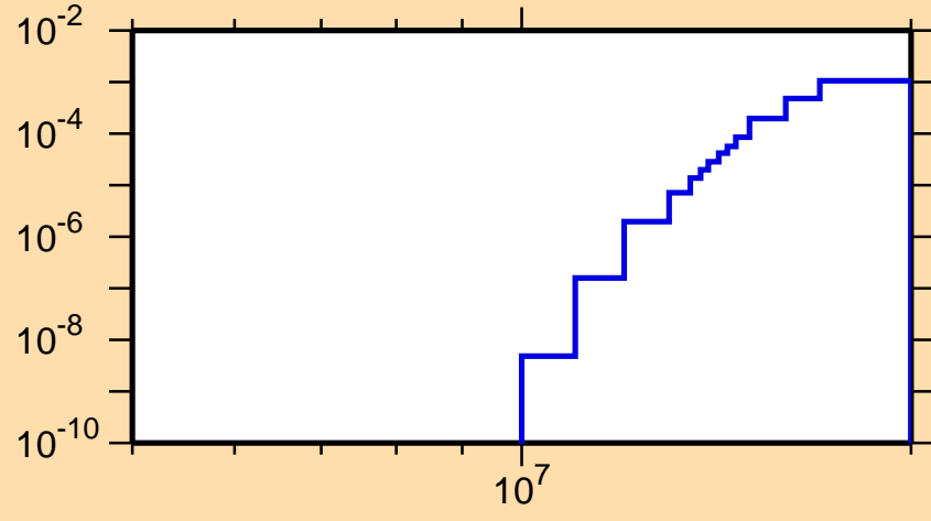
\sigma vs. E for ^{217}\text{Po}(n,d)
