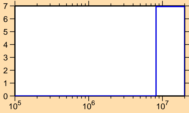
\Delta\sigma/\sigma vs. E for ^{217}\text{Po}(n,f)
