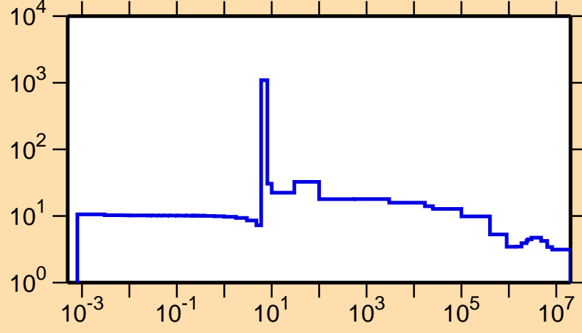
\sigma vs. E for ^{217}\text{Po}(n,\text{el.})
