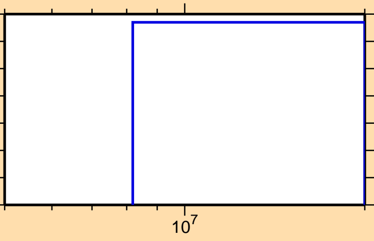
\sigma vs. E for ^{217}\text{Po}(n,d)
