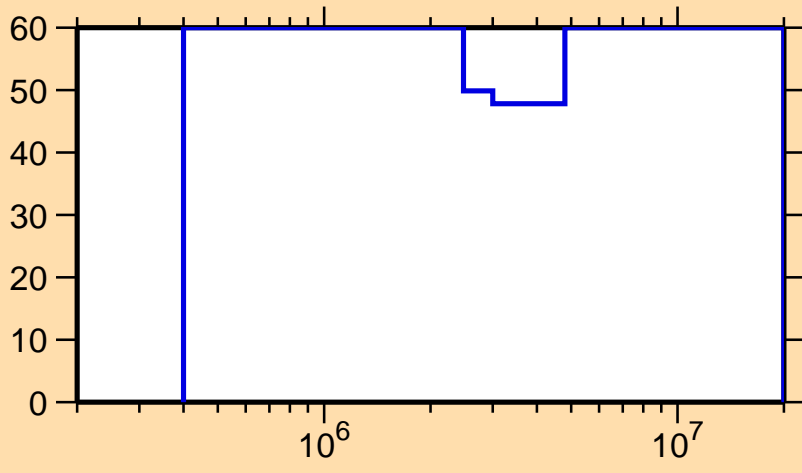
\Delta\sigma/\sigma vs. E for ^{217}\text{Po}(n,n\text{cont.})
