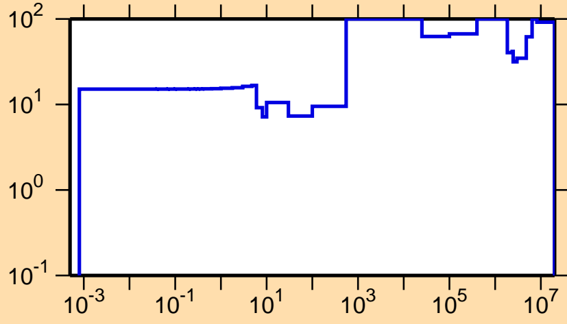
\Delta\sigma/\sigma vs. E for ^{217}\text{Po}(n,el.)
