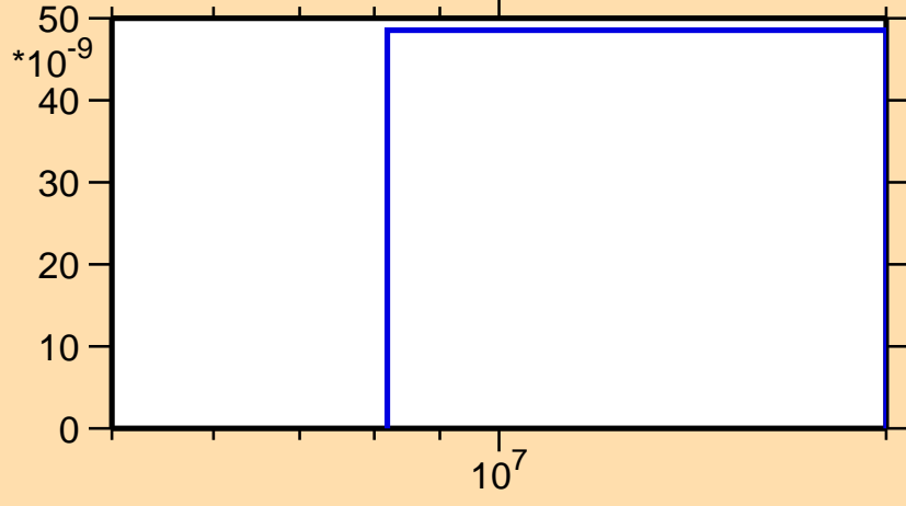
\sigma vs. E for ^{217}\text{Po}(n,2np)
