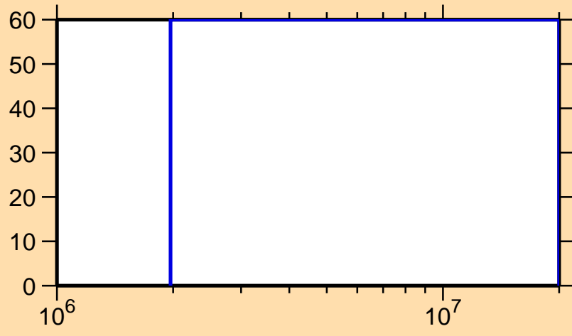
\Delta\sigma/\sigma vs. E for ^{218}\text{Po}(n,n\text{cont.})
