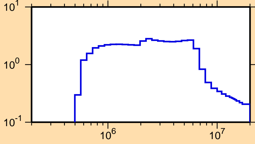
\sigma vs. E for ^{218}\text{Po}(n,\text{inel.})
