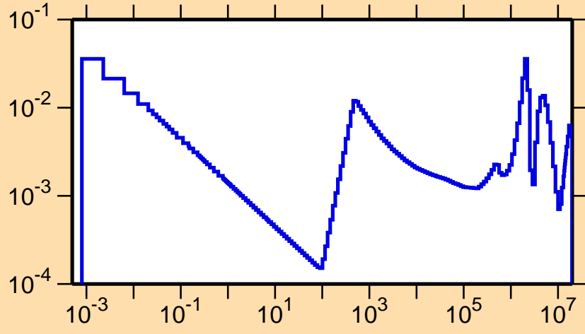
\sigma vs. E for ^{218}\text{Po}(n,\alpha)
