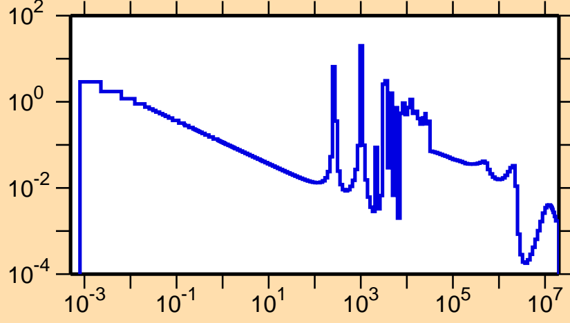
\sigma vs. E for ^{218}\text{Po}(n,\gamma)
