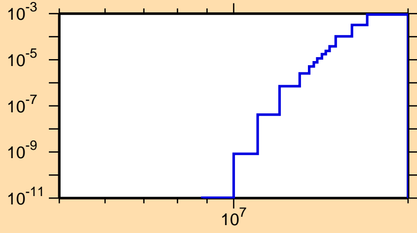
\sigma vs. E for ^{218}\text{Po}(n,d)
