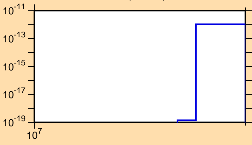
\sigma vs. E for ^{218}\text{Po}(\text{mt 11})
