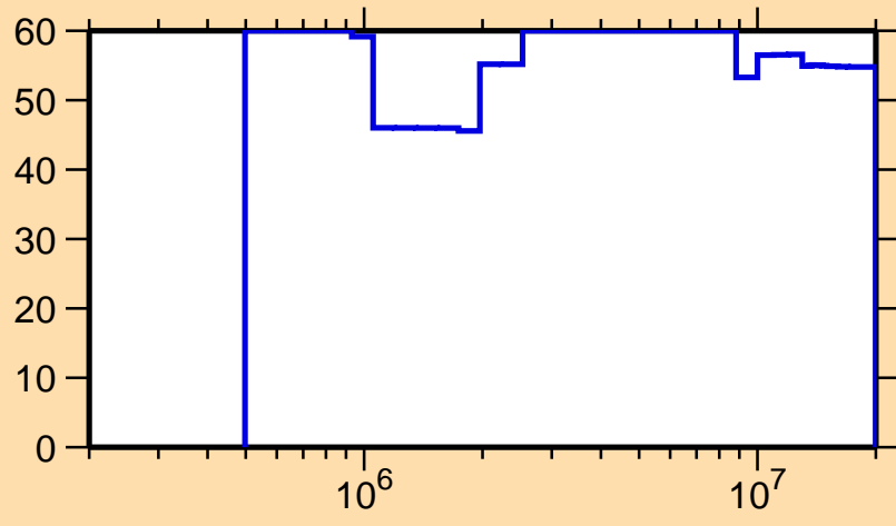
\Delta\sigma/\sigma vs. E for ^{218}\text{Po}(n,\text{inel.})
