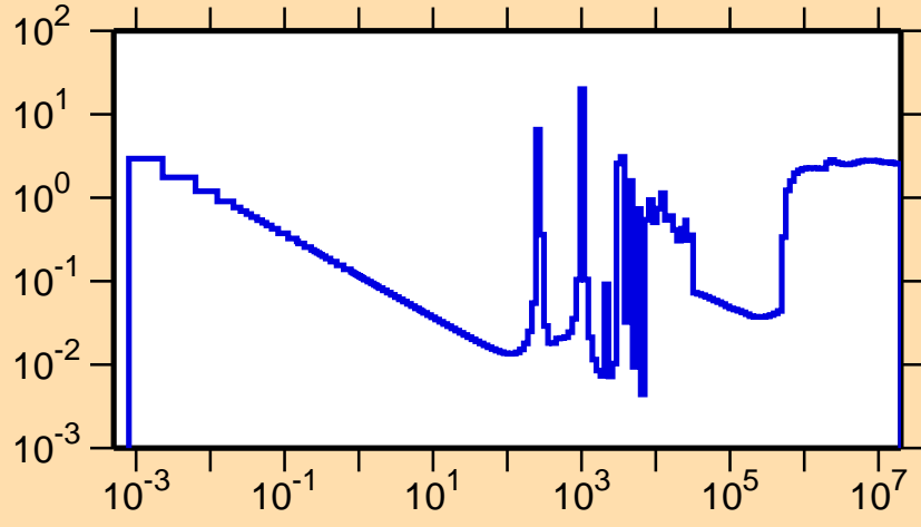
\sigma vs. E for ^{218}\text{Po}(n,\text{nonel.})
