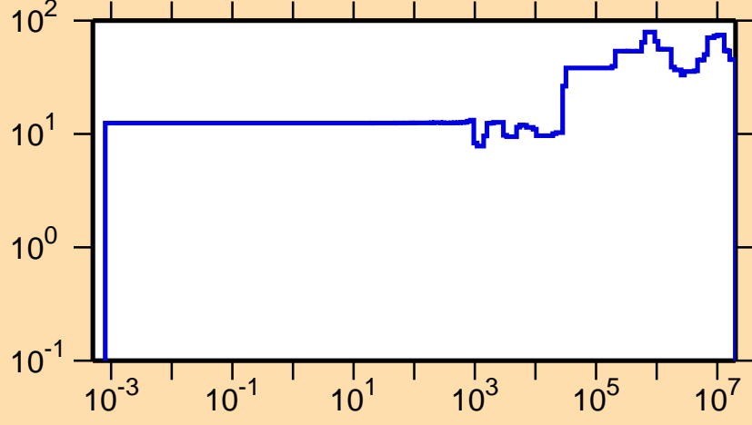
\Delta\sigma/\sigma vs. E for ^{218}\text{Po}(n,el.)
