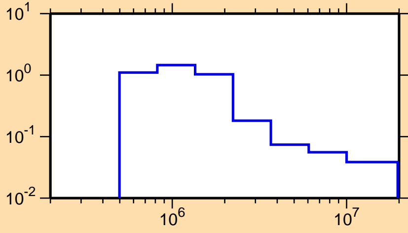
\sigma vs. E for ^{218}\text{Po}(n,n_1)
