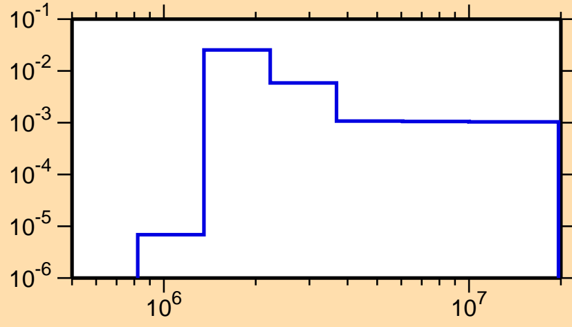
\sigma vs. E for ^{218}\text{Po}(n,n_4)
