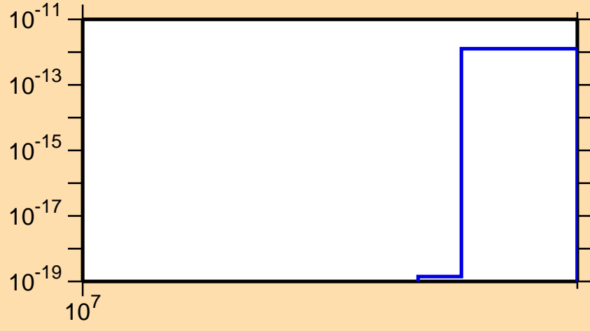
\sigma vs. E for ^{219}\text{Po}(\text{mt 11})
