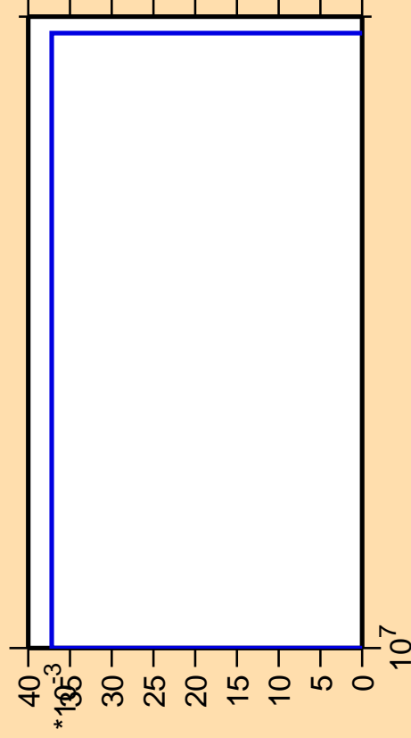
\Delta\sigma/\sigma vs. E for ^{219}\text{Po} (mt 11)
