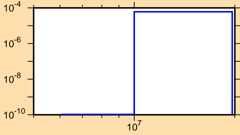
\sigma vs. E for ^{219}\text{Po}(n,t)
