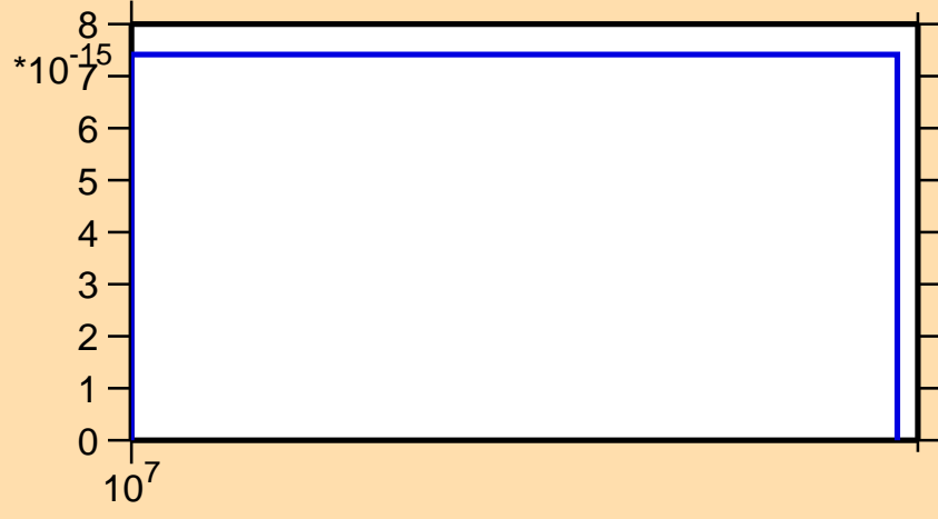
\sigma vs. E for ^{219}\text{Po} (mt 11)
