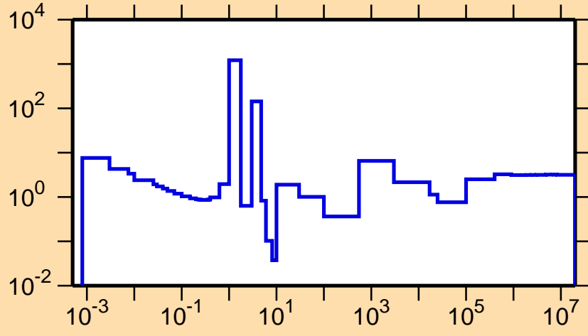
\sigma vs. E for ^{219}\text{Po}(n,\text{nonel.})
