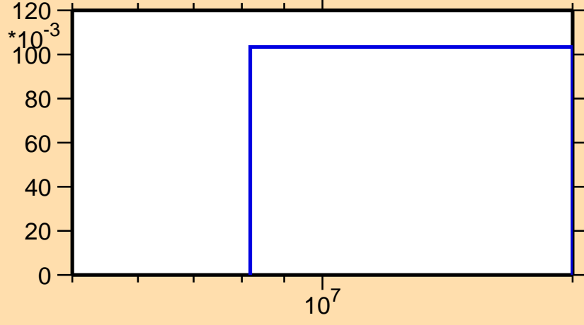
\sigma vs. E for ^{219}\text{Po}(n,3n)
