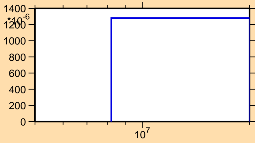
\sigma vs. E for ^{219}\text{Po}(n,3n\alpha)
