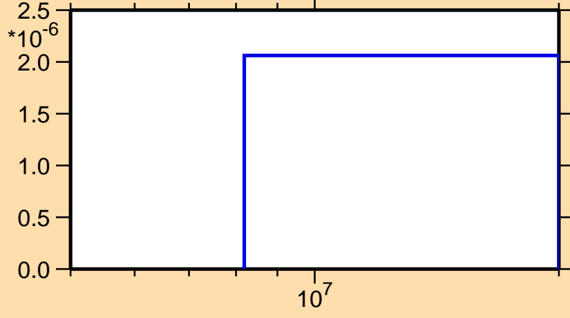
\sigma vs. E for ^{219}\text{Po}(n,2np)
