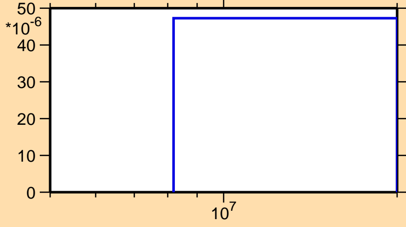
\sigma vs. E for ^{219}\text{Po}(n,d)
