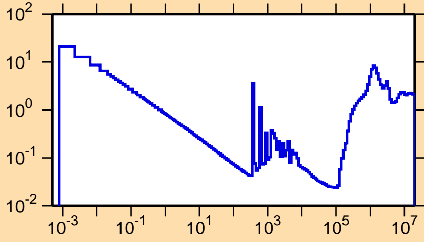
\sigma vs. E for ^{220}\text{Po}(n,\text{nonel.})
