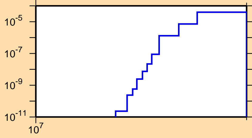
\sigma vs. E for ^{220}\text{Po}(n,nt)
