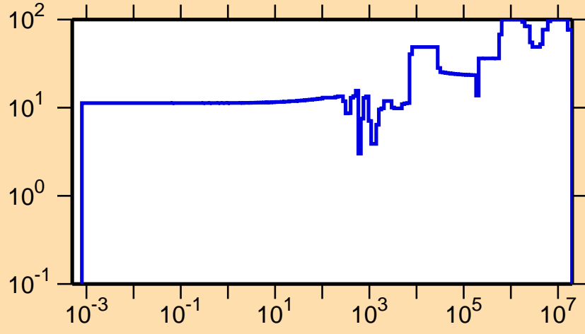
\Delta\sigma/\sigma vs. E for ^{220}\text{Po}(n,\text{el.})
