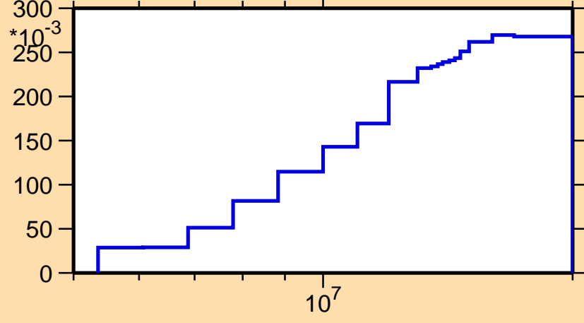
\sigma vs. E for ^{220}\text{Po}(n,2n)
