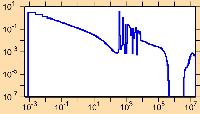
\sigma vs. E for ^{220}\text{Po}(n,\gamma)
