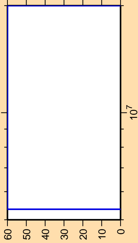
\Delta\sigma/\sigma vs. E for ^{220}\text{Po}(n,\gamma)
