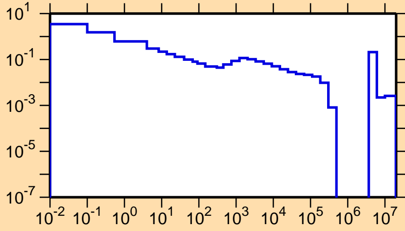
\sigma vs. E for ^{220}\text{Po}(n,\alpha)
