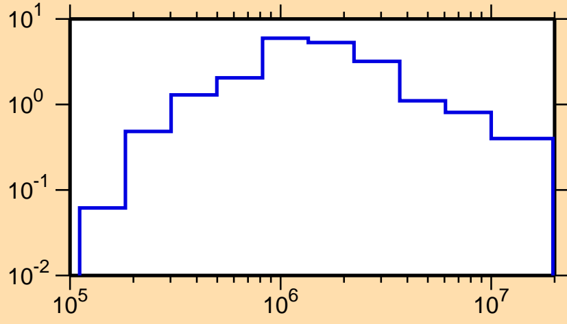
\sigma vs. E for ^{220}\text{Po}(n,\text{inel.})
