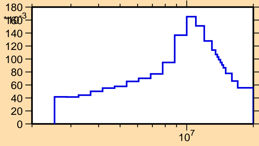
\sigma vs. E for ^{221}\text{Po}(n,n\alpha)
