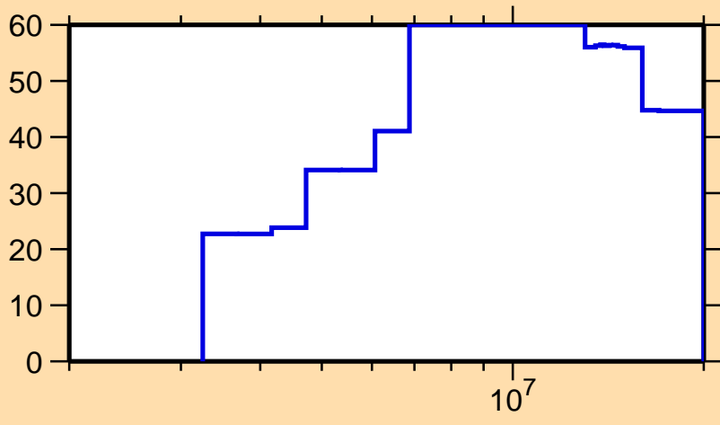
\Delta\sigma/\sigma vs. E for ^{221}\text{Po}(n,\text{tot.})
