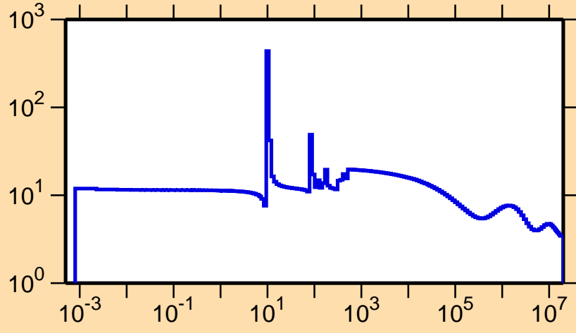
\sigma vs. E for ^{221}\text{Po}(n,\text{el.})
