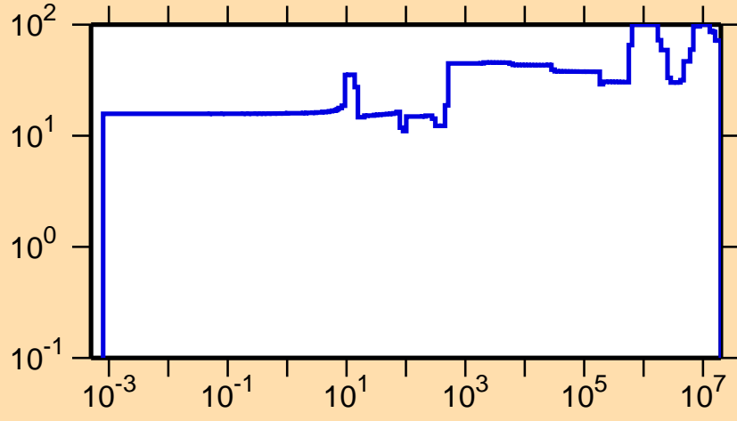
\Delta\sigma/\sigma vs. E for ^{221}\text{Po}(n,\text{el.})
