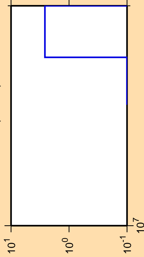
\Delta\sigma/\sigma vs. E for ^{221}\text{Po}(\text{mt } 11)
