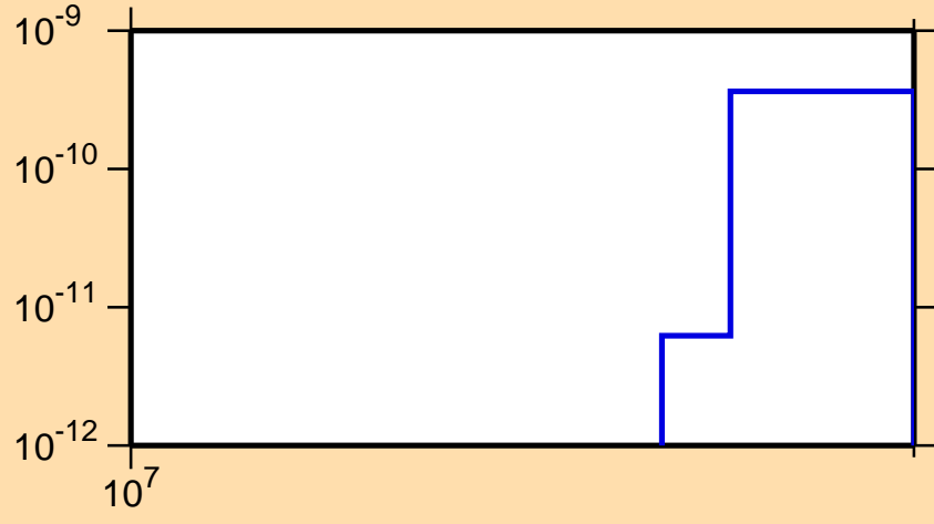
\sigma vs. E for ^{221}\text{Po}(n,\text{He}3)
