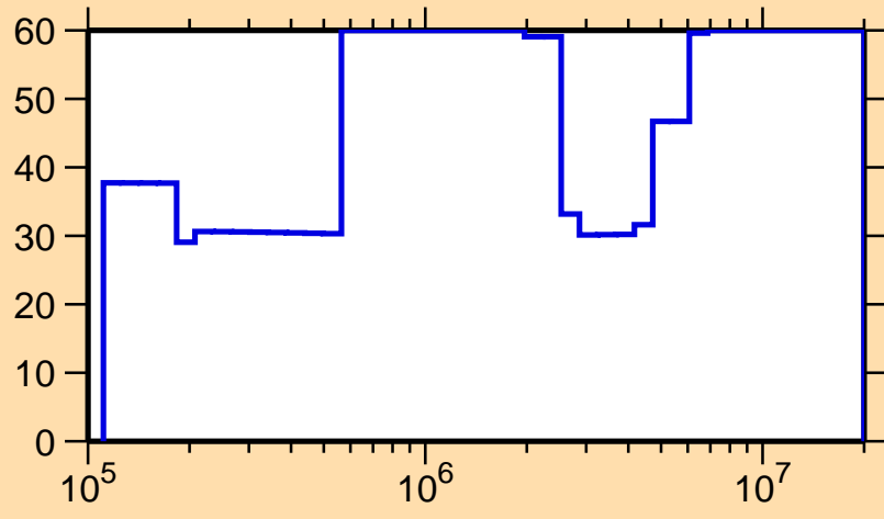
\Delta\sigma/\sigma vs. E for ^{221}\text{Po}(n,\text{el.})
