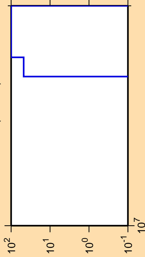
\Delta\sigma/\sigma vs. E for ^{221}\text{Po}(n,\text{He}3)
