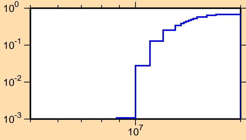
\sigma vs. E for ^{221}\text{Po}(n,3n)
