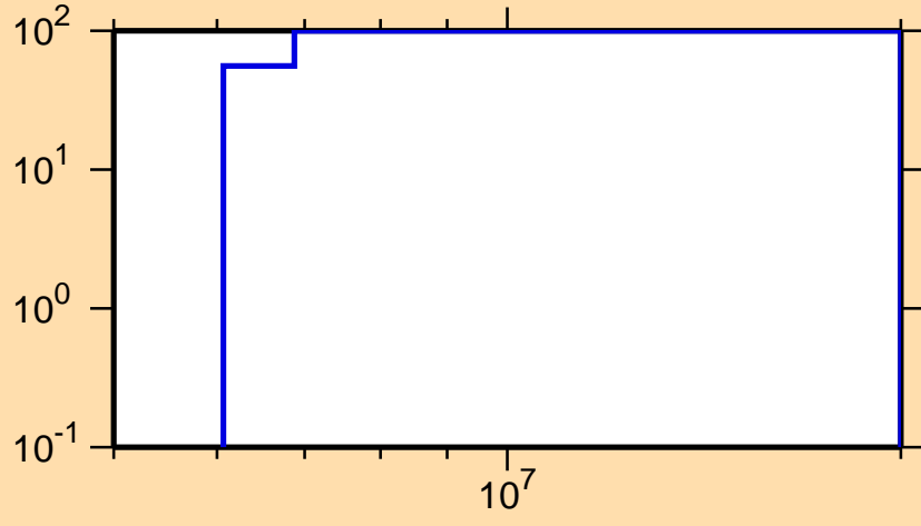
\Delta\sigma/\sigma vs. E for ^{221}\text{Po}(n,p)
