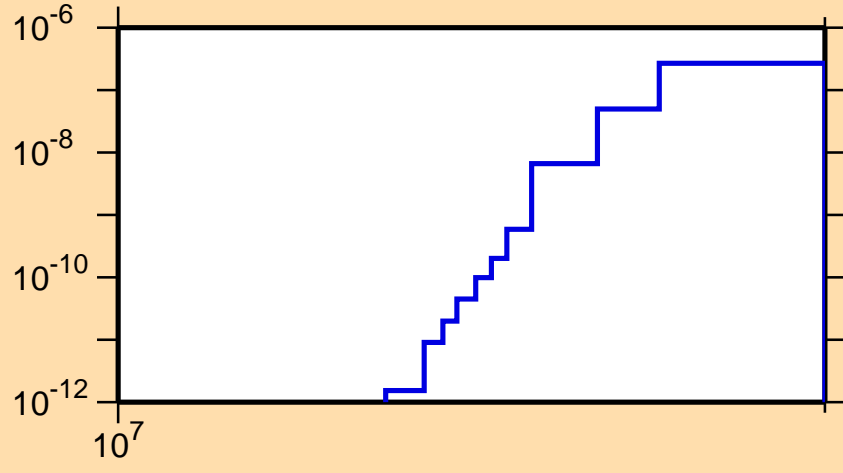
\sigma vs. E for ^{221}\text{Po}(n,nt)
