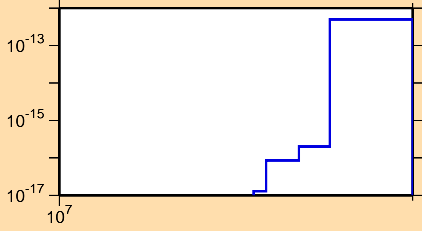
\sigma vs. E for ^{221}\text{Po}(\text{mt } 11)
