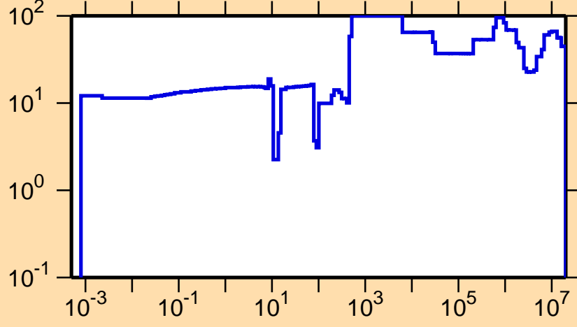
\Delta\sigma/\sigma vs. E for ^{221}\text{Po}(n,\text{tot.})
