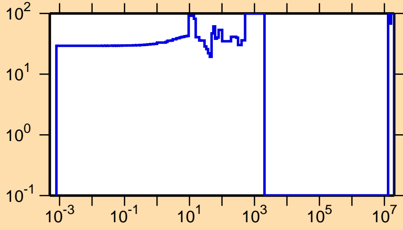
\Delta\sigma/\sigma vs. E for ^{221}\text{Po}(n,f)
