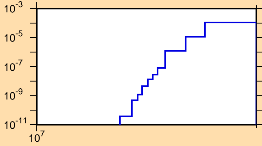
\sigma vs. E for ^{221}\text{Po}(n,\text{nd})
