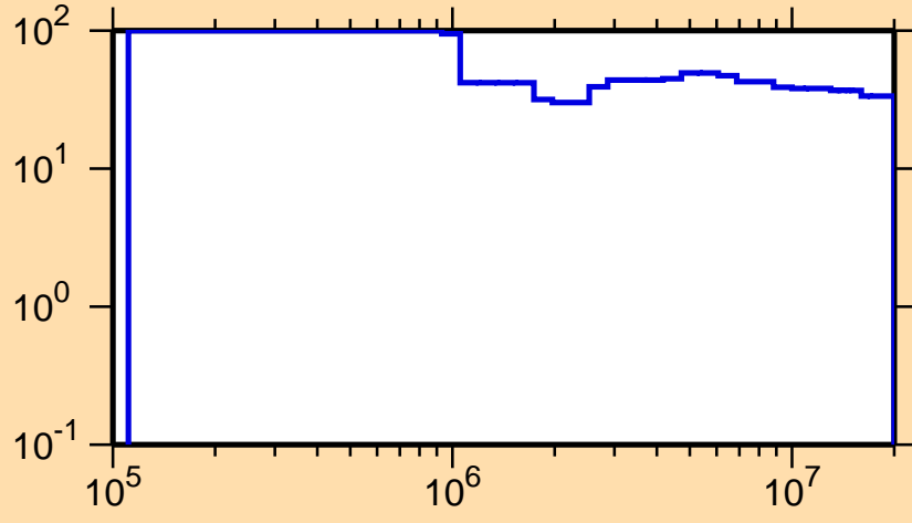
\Delta\sigma/\sigma vs. E for ^{221}\text{Po}(n,\text{nonel.})
