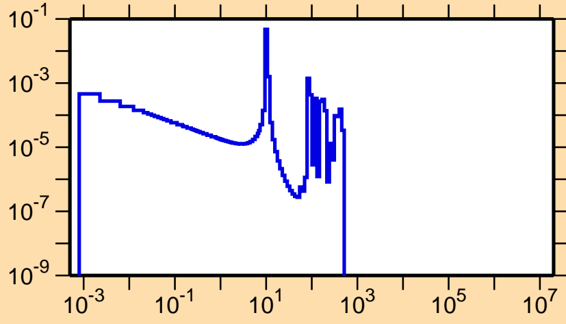
\sigma vs. E for ^{221}\text{Po}(n,f)
