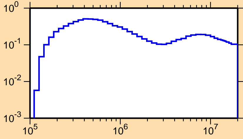
\sigma vs. E for ^{221}\text{Po}(n,n\text{cont.})
