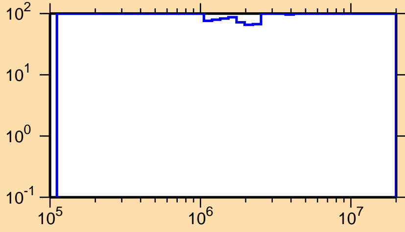
\Delta\sigma/\sigma vs. E for ^{221}\text{Po}(n,n\text{cont.})
