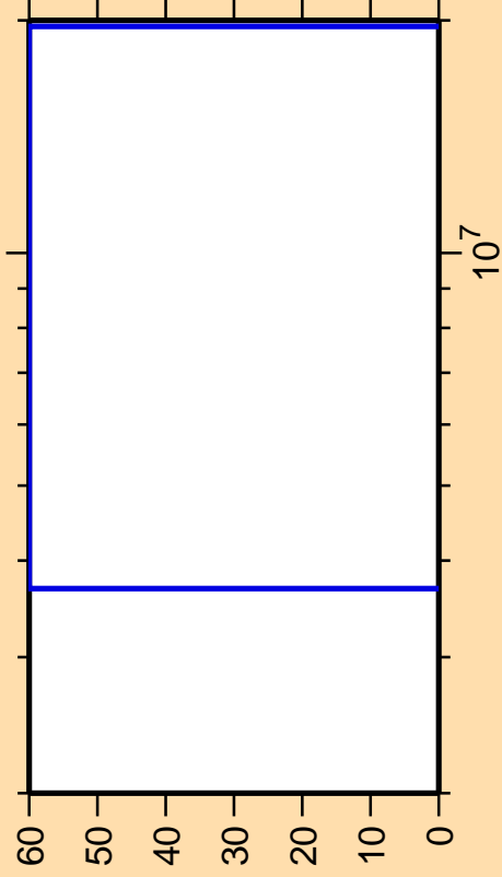
\Delta\sigma/\sigma vs. E for ^{221}\text{Po}(n,2n\alpha)
