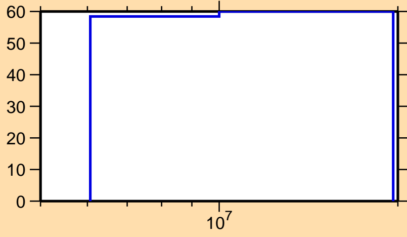
\Delta\sigma/\sigma vs. E for ^{221}\text{Po}(n,2n)
