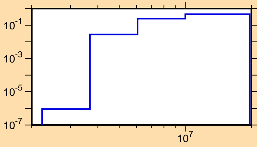
\sigma vs. E for ^{221}\text{Po}(n,2n)
