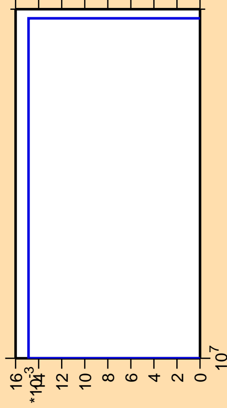
\Delta\sigma/\sigma vs. E for ^{221}\text{Po} (mt 11)
