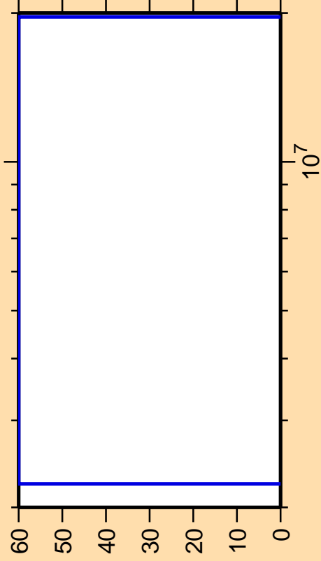
\Delta\sigma/\sigma vs. E for ^{221}\text{Po}(n,n\text{cont.})
