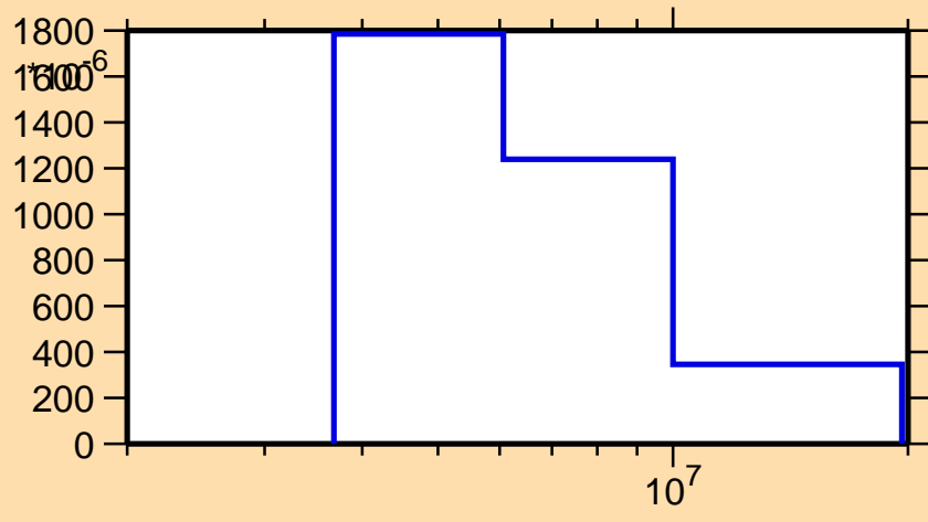
\sigma vs. E for ^{221}\text{Po}(n,2n\alpha)
