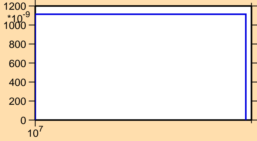
\sigma vs. E for ^{221}\text{Po}(n,2np)
