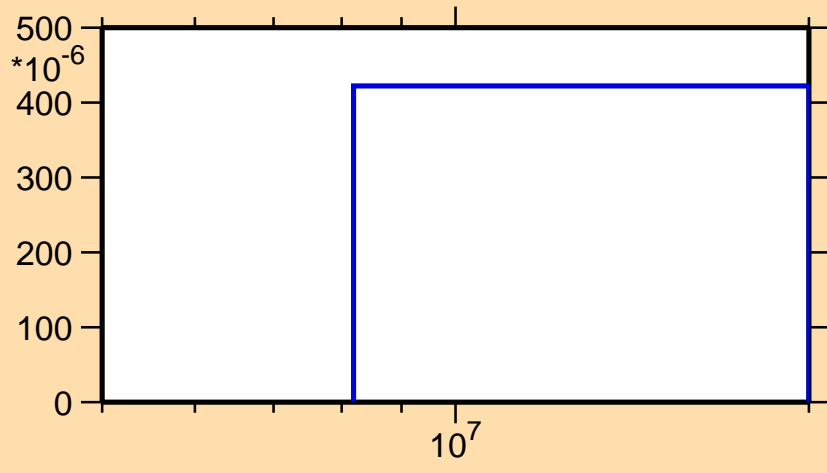
\sigma vs. E for ^{221}\text{Po}(n,t)
