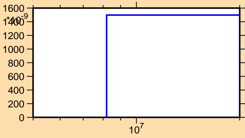
\sigma vs. E for ^{221}\text{Po}(n,\text{nd})
