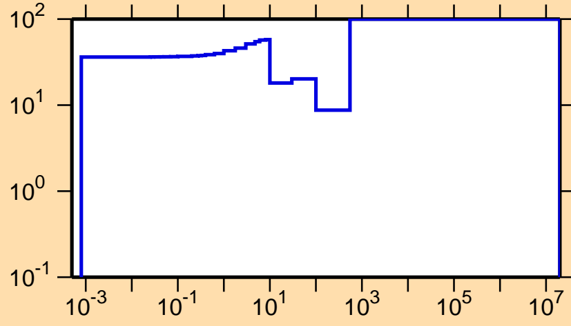
\Delta\sigma/\sigma vs. E for ^{221}\text{Po}(n,\gamma)
