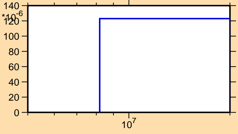
\sigma vs. E for ^{221}\text{Po}(n,d)
