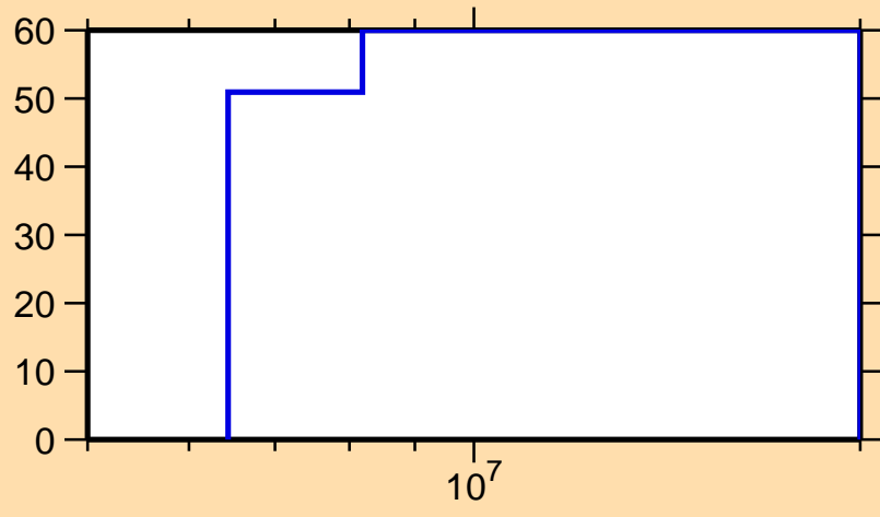
\Delta\sigma/\sigma vs. E for ^{221}\text{Po}(n,2n)
