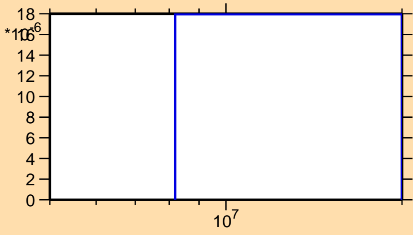
\sigma vs. E for ^{221}\text{Po}(n,np)
