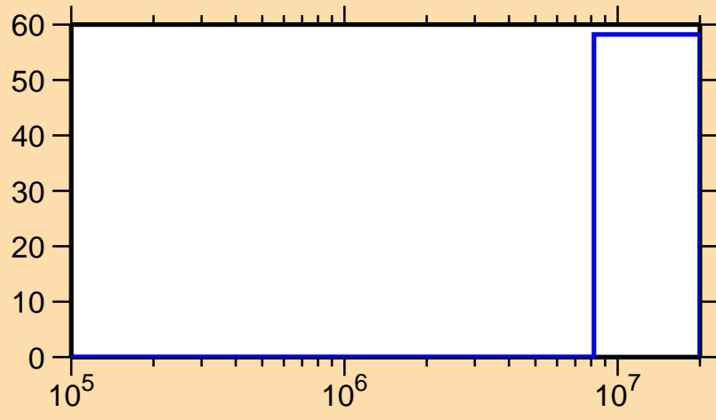
\Delta\sigma/\sigma vs. E for ^{221}\text{Po}(n,f)
