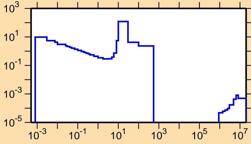
\sigma vs. E for ^{221}\text{Po}(n,\gamma)
