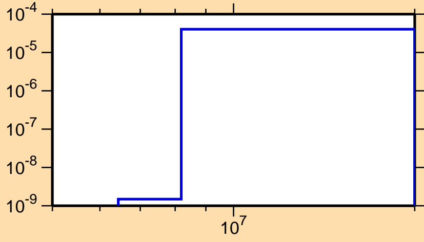
\sigma vs. E for ^{221}\text{Po}(n,p)
