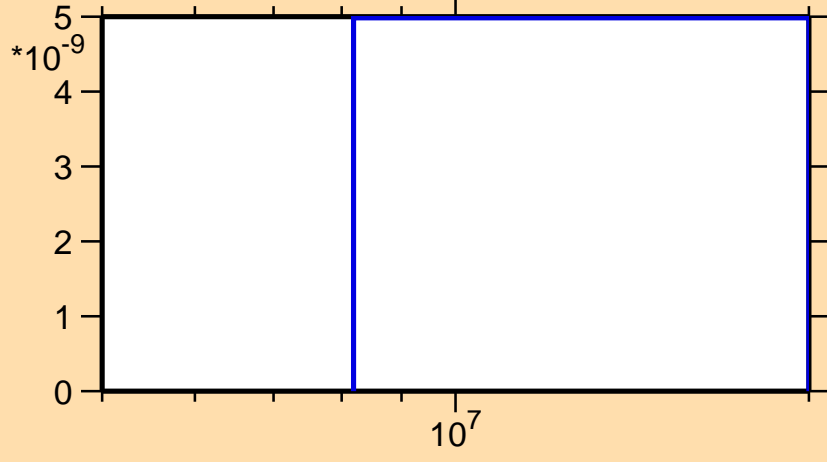
\sigma vs. E for ^{221}\text{Po}(n,nt)
