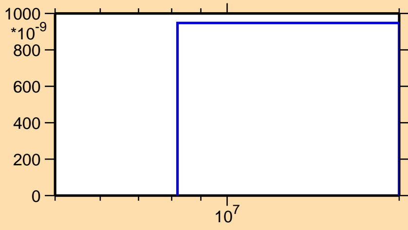
\sigma vs. E for ^{221}\text{Po}(n,2np)
