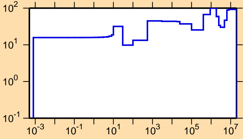
\Delta\sigma/\sigma vs. E for ^{221}\text{Po}(n,el.)
