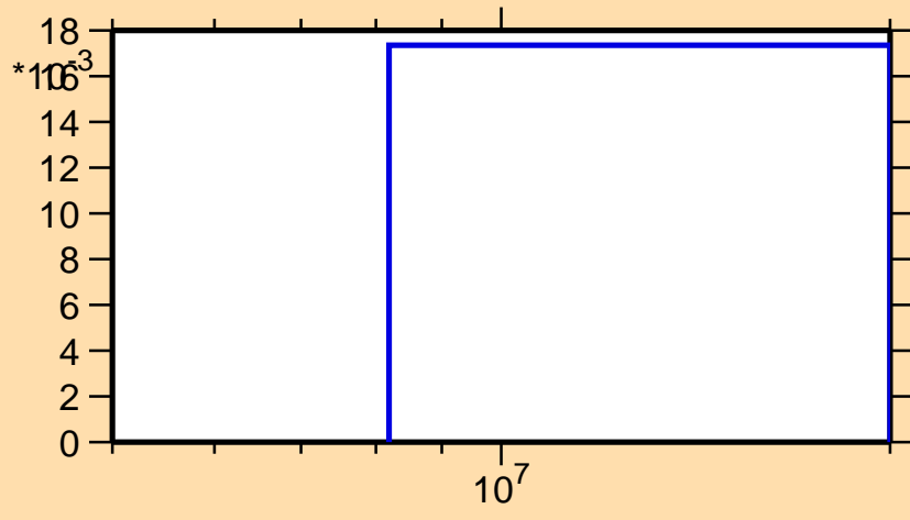
\sigma vs. E for ^{221}\text{Po}(n,3n\alpha)
