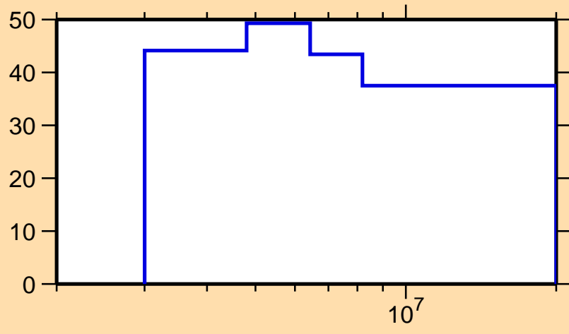
\Delta\sigma/\sigma vs. E for ^{221}\text{Po}(n,\text{nonel.})
