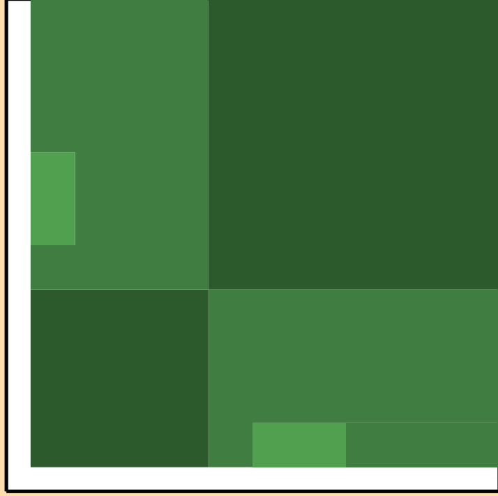
\sigma vs. E for ^{222}\text{Po}(n,2n)
