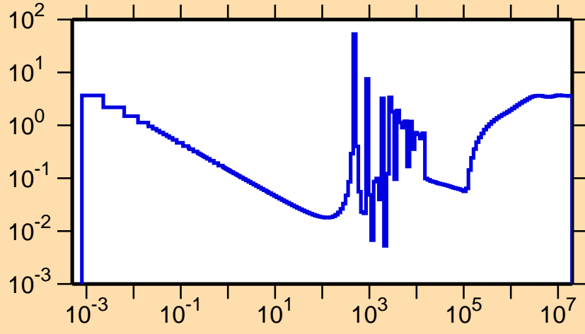
\sigma vs. E for ^{222}\text{Po}(n,\text{nonel.})
