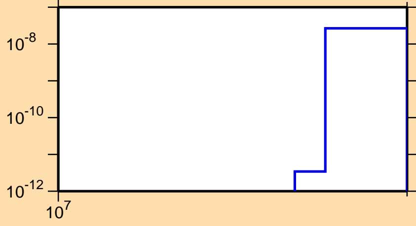
\sigma vs. E for ^{222}\text{Po}(n,2np)
