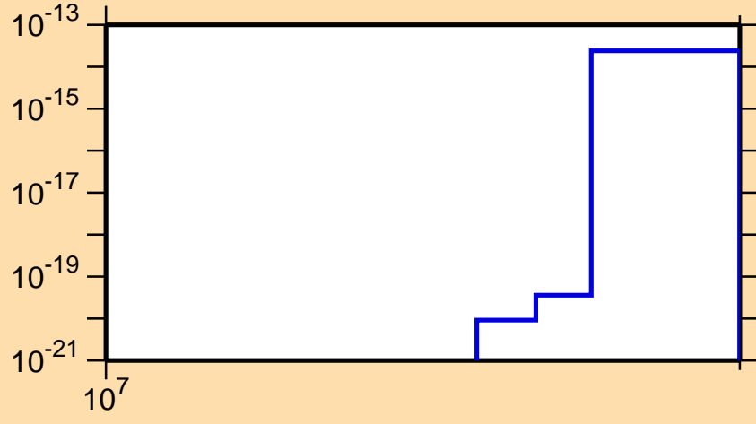
\sigma vs. E for ^{222}\text{Po}(\text{mt 11})
