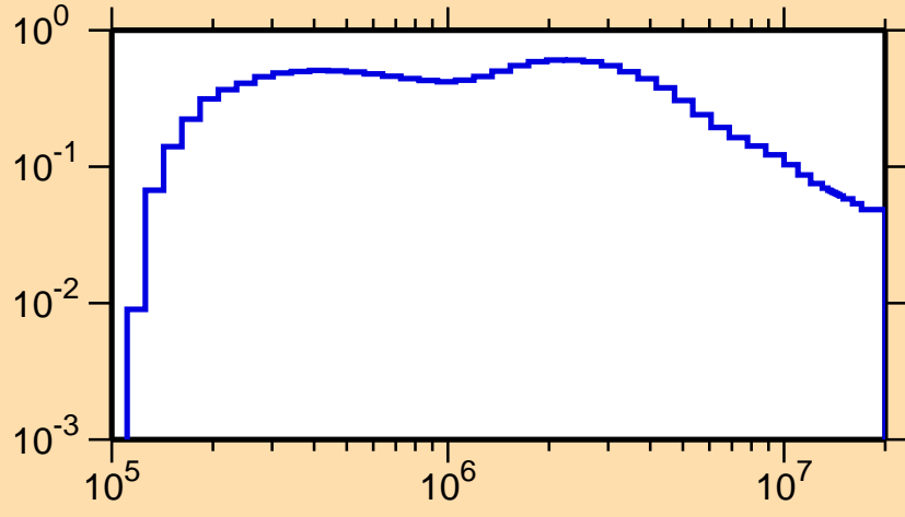
\sigma vs. E for ^{222}\text{Po}(n,n_1)
