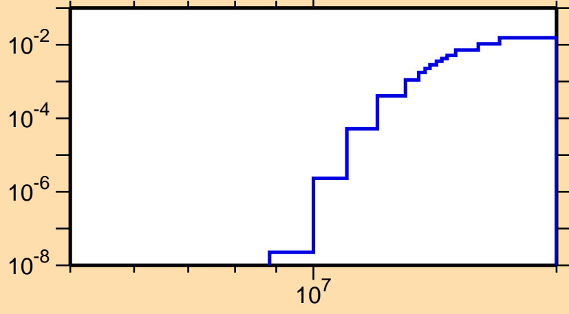
\sigma vs. E for ^{222}\text{Po}(n,t)
