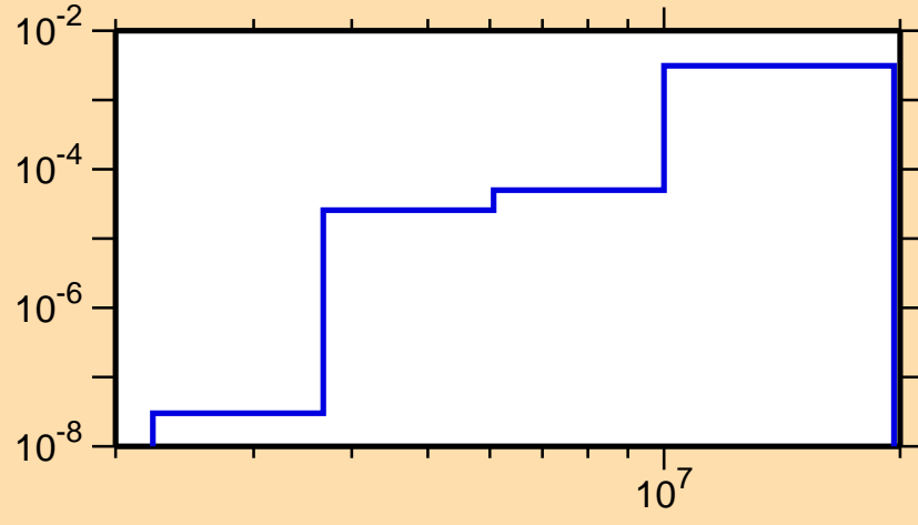
\sigma vs. E for ^{222}\text{Po}(n,n\alpha)
