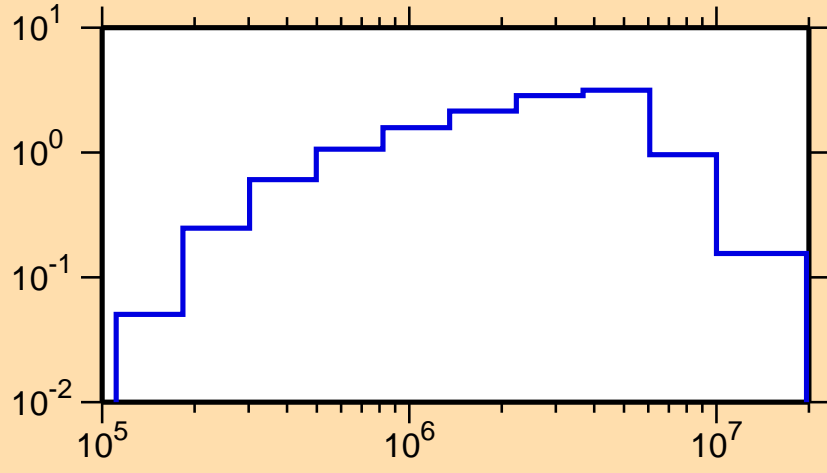
\sigma vs. E for ^{222}\text{Po}(n,n\text{cont.})
