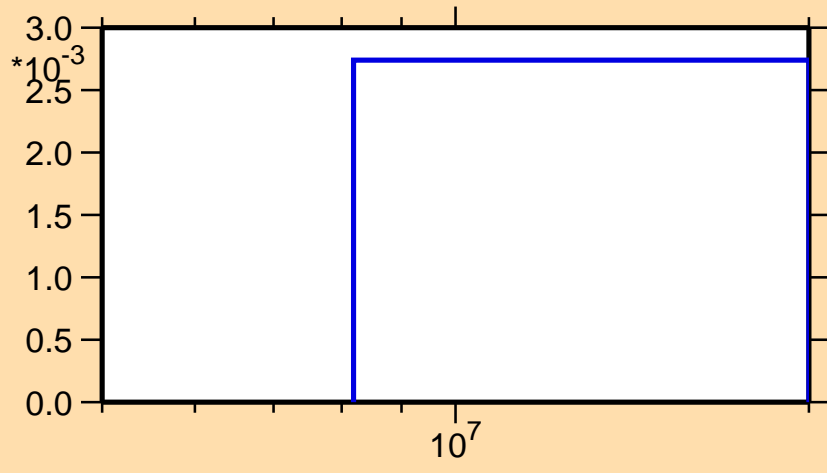
\sigma vs. E for ^{222}\text{Po}(n,t)
