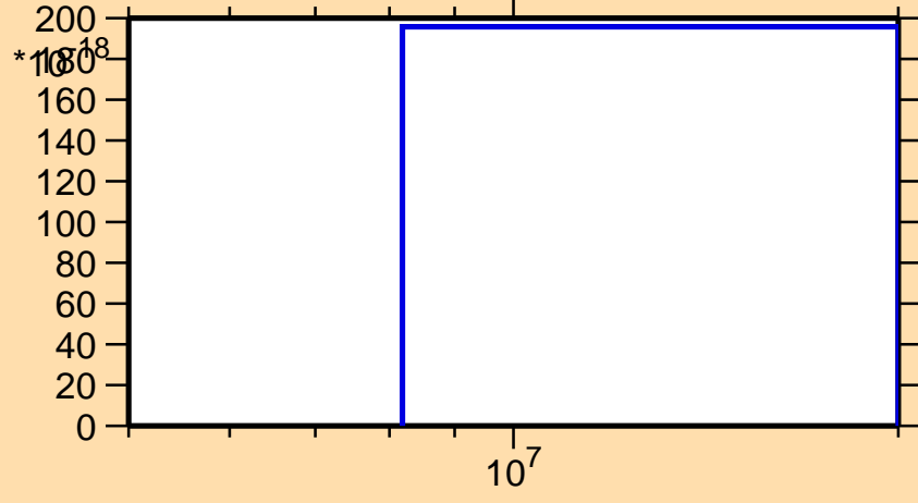
\sigma vs. E for ^{222}\text{Po} (mt 11)
