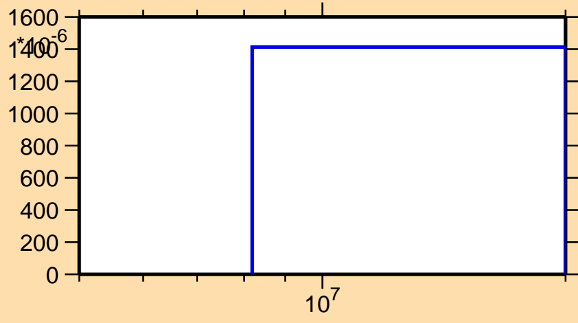
\sigma vs. E for ^{222}\text{Po}(n,3n)
