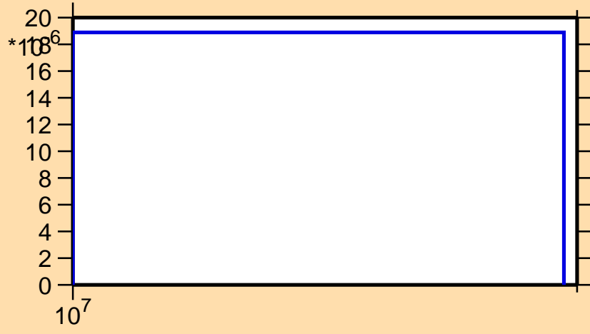
\sigma vs. E for ^{223}\text{Po}(n,3n\alpha)
