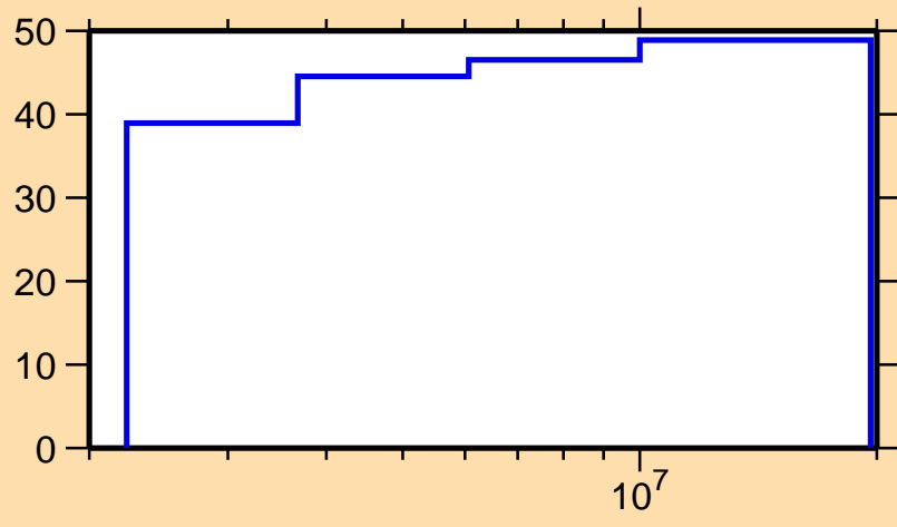
\Delta\sigma/\sigma vs. E for ^{223}\text{Po}(n,\text{nonel.})
