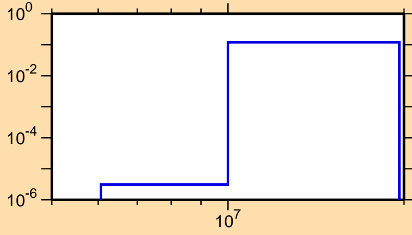
\sigma vs. E for ^{223}\text{Po}(n,2n\alpha)
