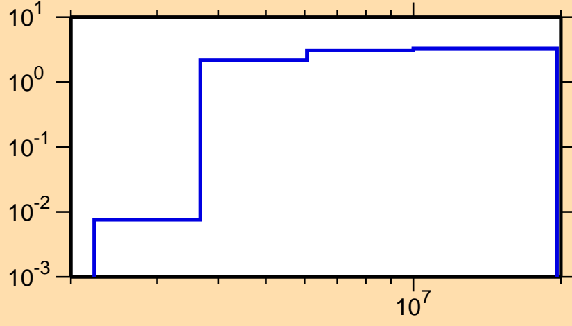
\sigma vs. E for ^{223}\text{Po}(n,2n)
