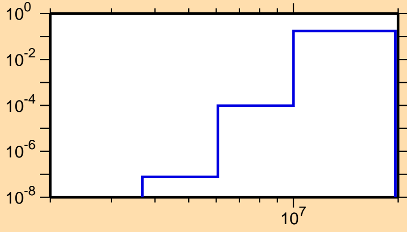
\sigma vs. E for ^{223}\text{Po}(n,n\alpha)
