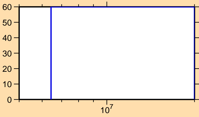
\Delta\sigma/\sigma vs. E for ^{223}\text{Po}(n,el.)
