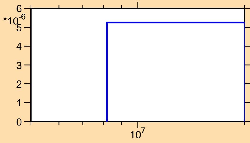
\sigma vs. E for ^{223}\text{Po}(n,np)
