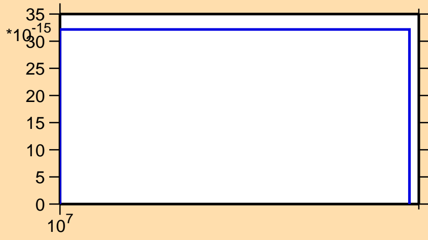
\sigma vs. E for ^{224}\text{Po}(n,2np)
