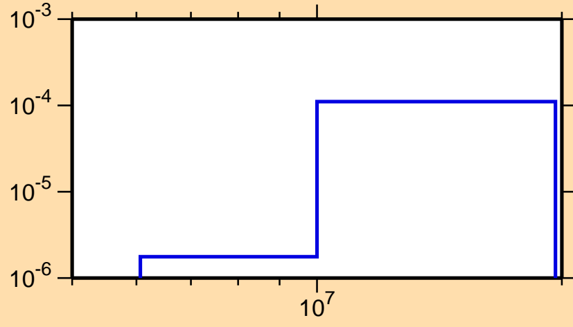
\sigma vs. E for ^{224}\text{Po}(n,n\alpha)
