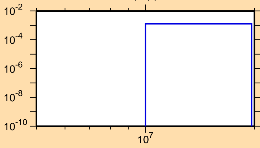
\sigma vs. E for ^{224}\text{Po}(n,p)
