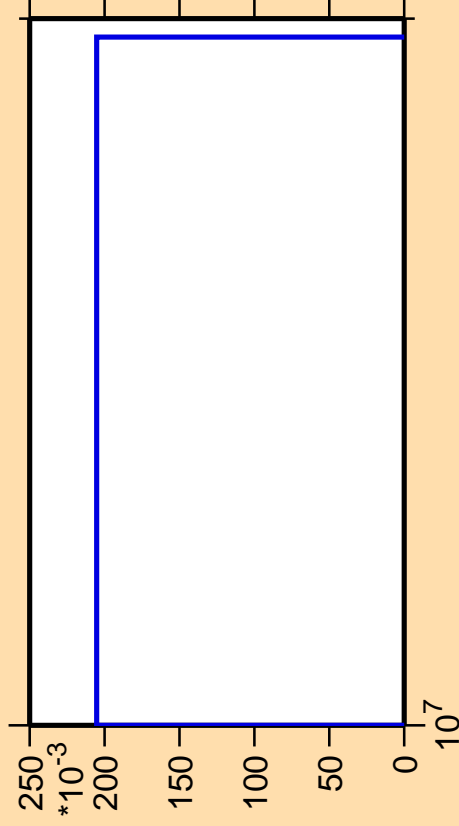
\Delta\sigma/\sigma vs. E for ^{224}\text{Po}(n,2np)
