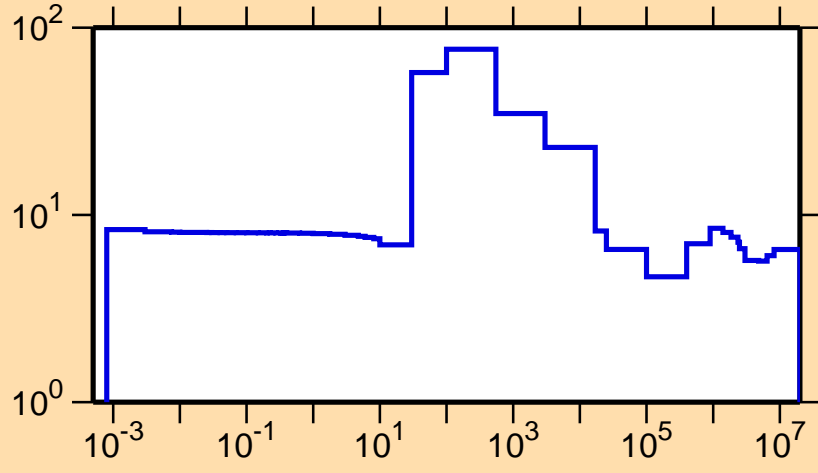
\sigma vs. E for ^{224}\text{Po}(n,\text{el.})
