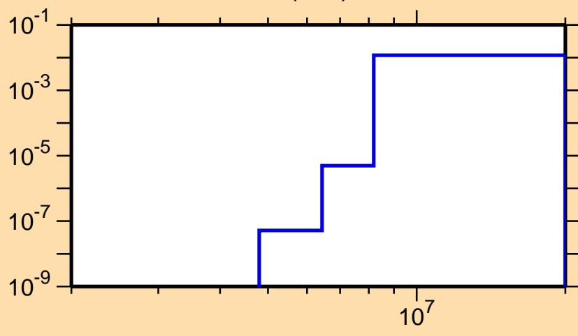
\sigma vs. E for ^{225}\text{Po}(n,\alpha)
