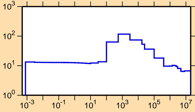
\sigma vs. E for ^{225}\text{Po}(n,\text{el.})
