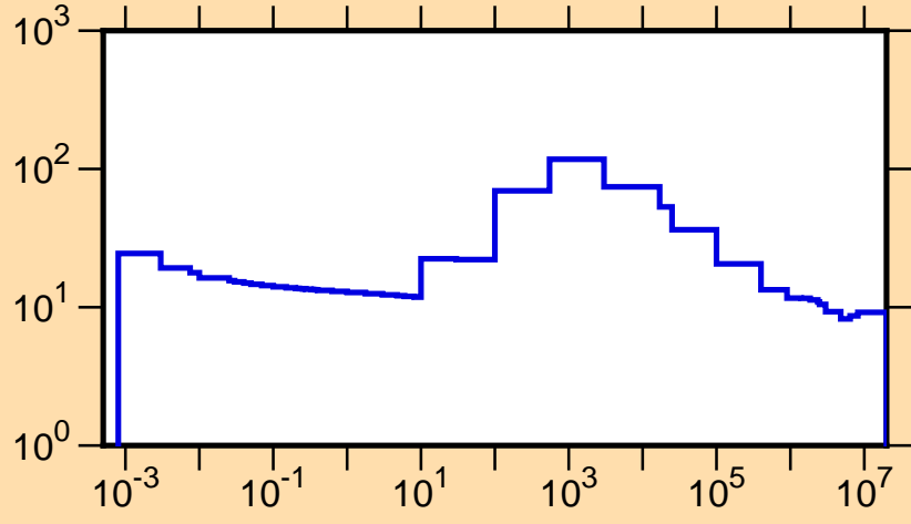
\sigma vs. E for ^{225}\text{Po}(n,\text{tot.})
