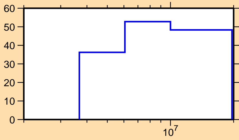
\Delta\sigma/\sigma vs. E for ^{226}\text{Po}(n,\text{tot.})
