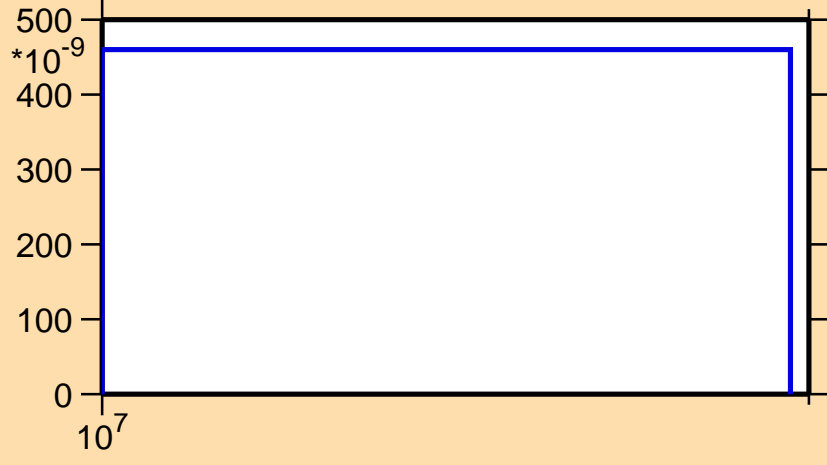
\sigma vs. E for ^{226}\text{Po}(n,np)
