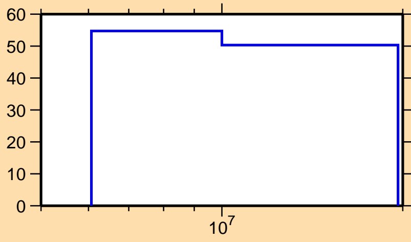
\Delta\sigma/\sigma vs. E for ^{226}\text{Po}(n,\text{nonel.})
