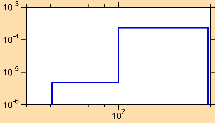
\sigma vs. E for ^{226}\text{Po}(n,n\alpha)
