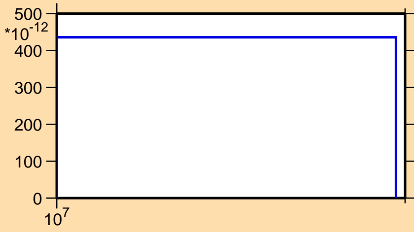
\sigma vs. E for ^{226}\text{Po}(n,\text{nd})
