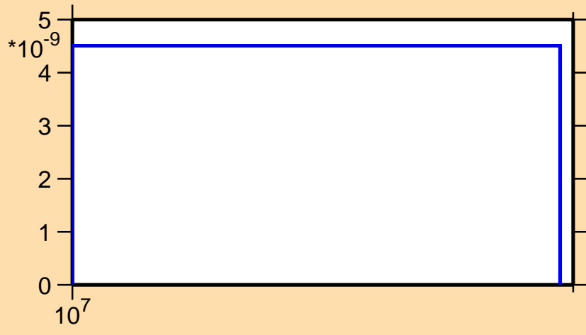
\sigma vs. E for ^{226}\text{Po}(n,3n\alpha)
