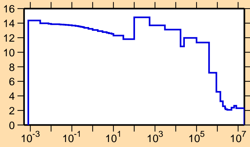
\sigma vs. E for ^{226}\text{Po}(n,\text{el.})
