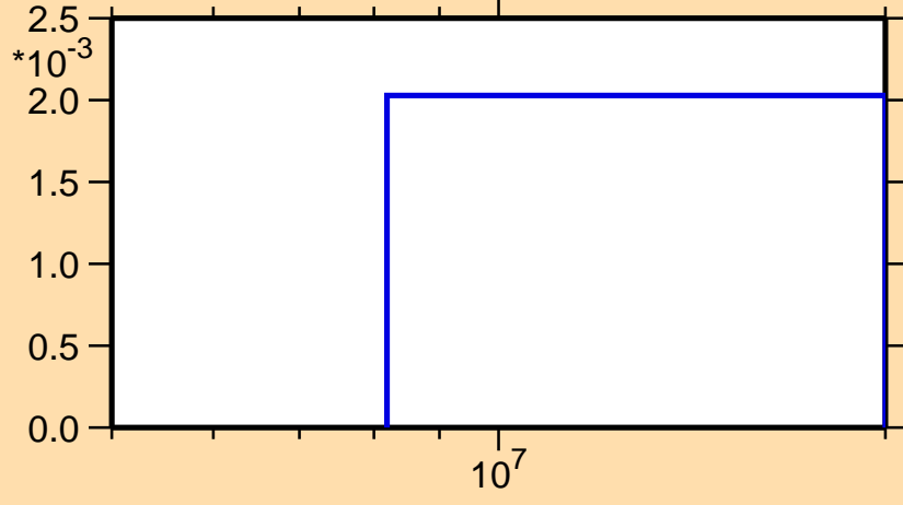
\sigma vs. E for ^{226}\text{Po}(n,p)
