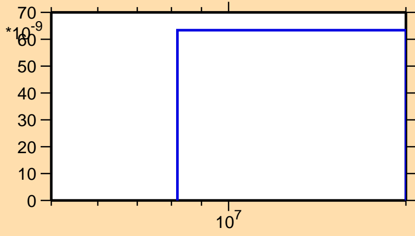
\sigma vs. E for ^{226}\text{Po}(n,nt)
