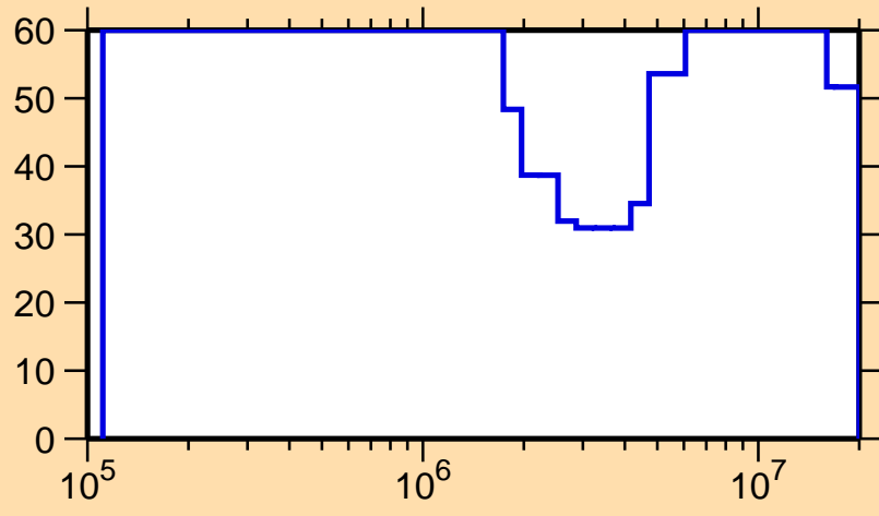
\Delta\sigma/\sigma vs. E for ^{227}\text{Po}(n,\text{tot.})
