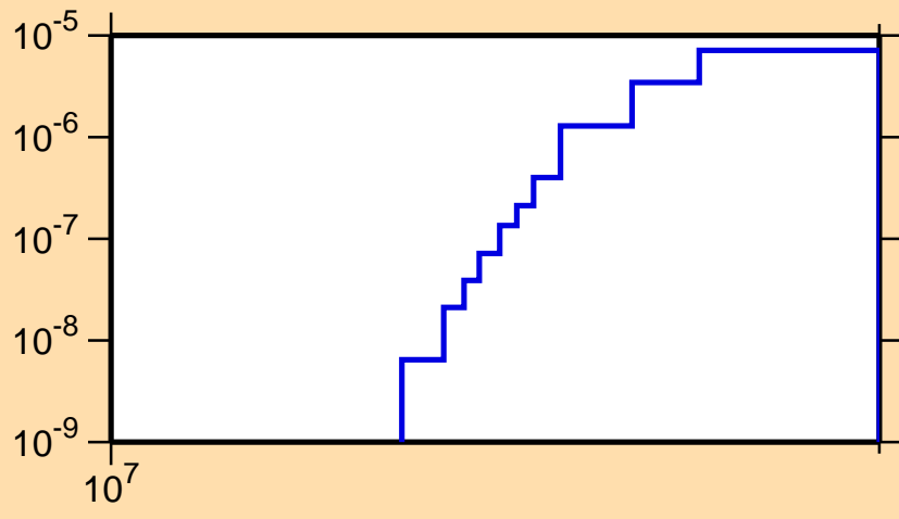
\sigma vs. E for ^{227}\text{Po}(n,2n\alpha)
