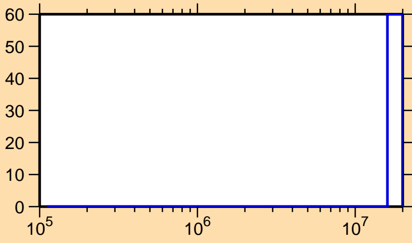
\Delta\sigma/\sigma vs. E for ^{227}\text{Po}(n,f)
