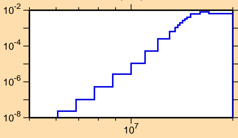
\sigma vs. E for ^{227}\text{Po}(n,\alpha)
