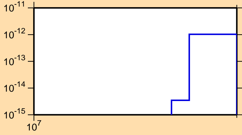
\sigma vs. E for ^{227}\text{Po}(n,3n\alpha)
