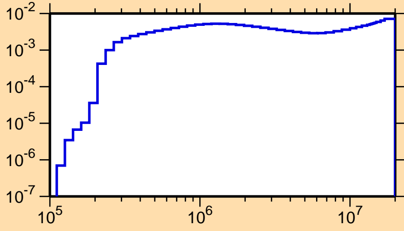
\sigma vs. E for ^{227}\text{Po}(n,n_1)
