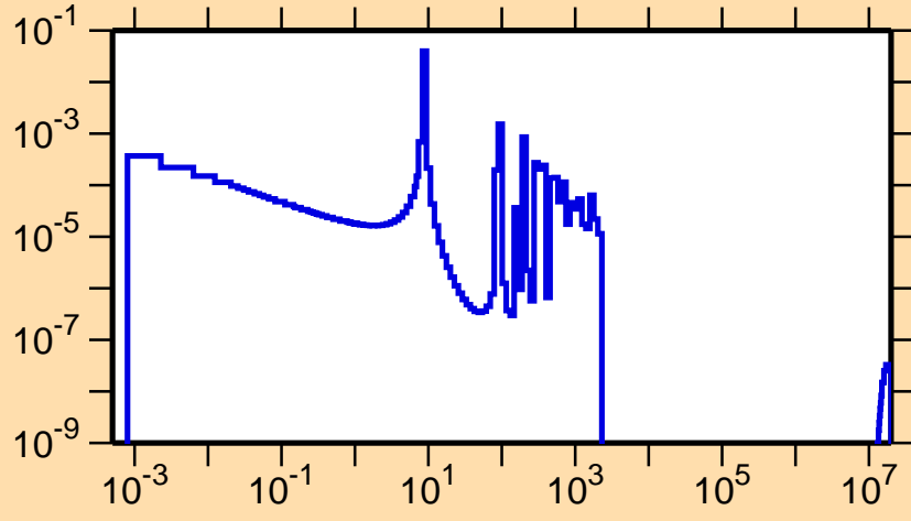
\sigma vs. E for ^{227}\text{Po}(n,f)
