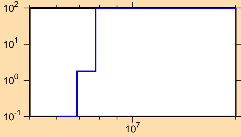
\Delta\sigma/\sigma vs. E for ^{227}\text{Po}(n,p)
