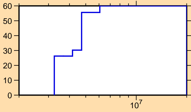
\Delta\sigma/\sigma vs. E for ^{227}\text{Po}(n,\text{el.})
