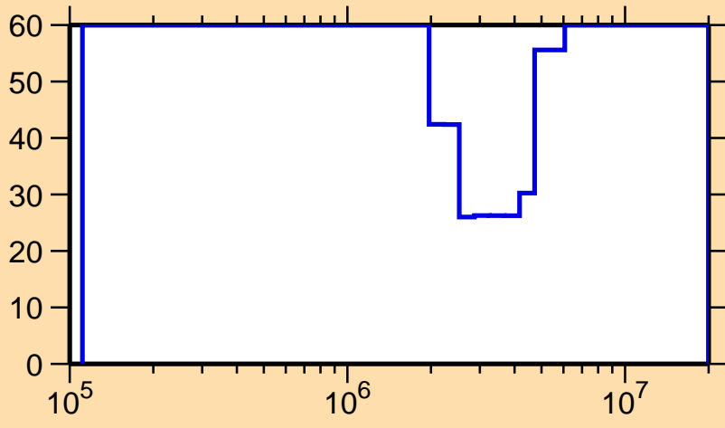
\Delta\sigma/\sigma vs. E for ^{227}\text{Po}(n, el.)
