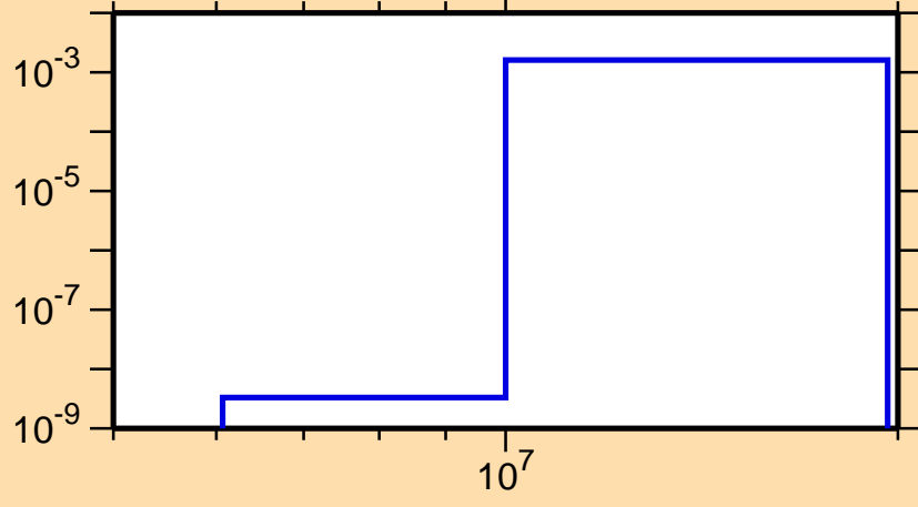
\sigma vs. E for ^{227}\text{Po}(n,p)
