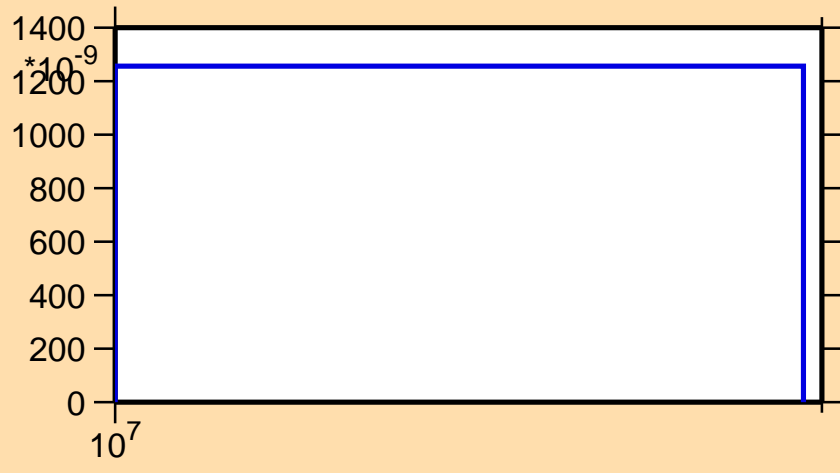
\sigma vs. E for ^{227}\text{Po}(n,nt)
