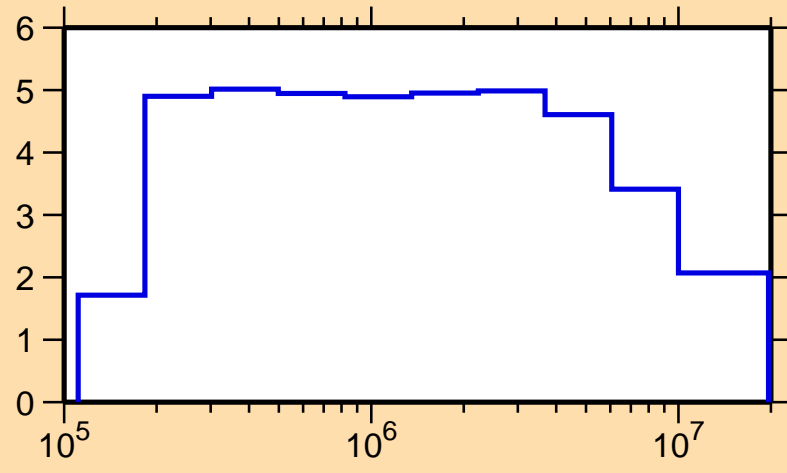
\sigma vs. E for ^{227}\text{Po}(n,\text{inel.})
