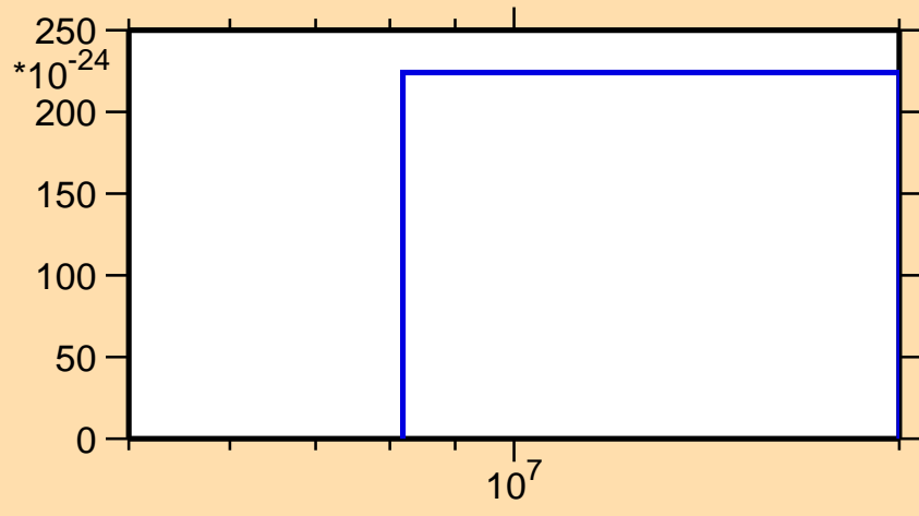
\sigma vs. E for ^{227}\text{Po} (mt 42)
