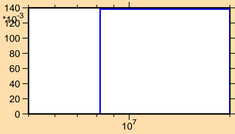
\sigma vs. E for ^{227}\text{Po}(n,t)
