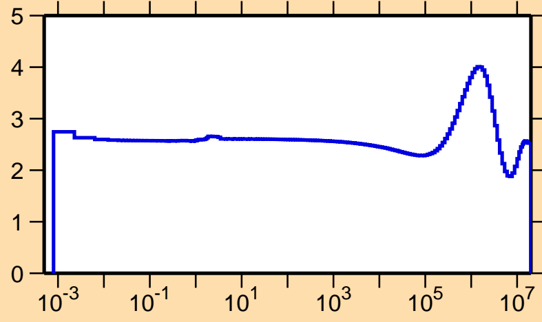
\sigma vs. E for ^{124}\text{Pr}(n,\text{el.})
