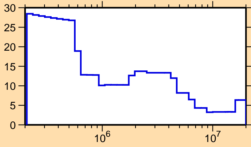
\Delta\sigma/\sigma vs. E for ^{124}\text{Pr}(n,\text{tot.})
