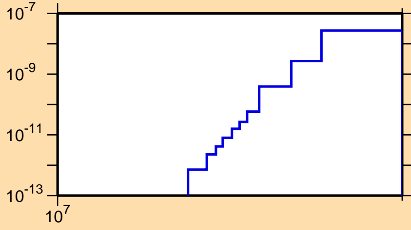
\sigma vs. E for ^{124}\text{Pr}(\text{mt } 34)
