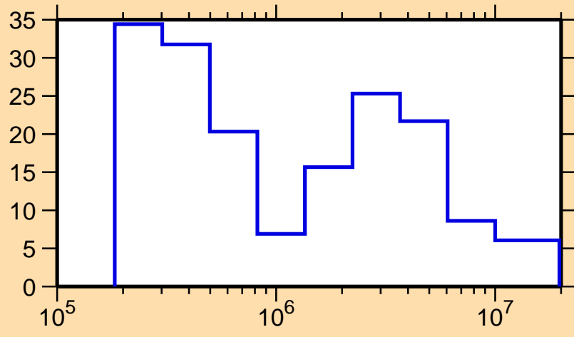
\Delta\sigma/\sigma vs. E for ^{124}\text{Pr}(n,\text{el.})
