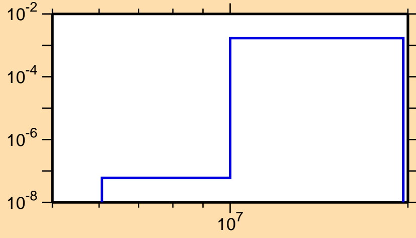
\sigma vs. E for ^{124}\text{Pr}(n,\text{pd})
