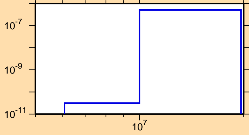
\sigma vs. E for ^{124}\text{Pr}(\text{mt117})
