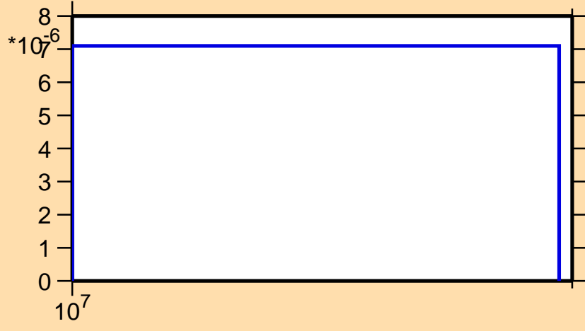
\sigma vs. E for ^{124}\text{Pr}(n,2np)
