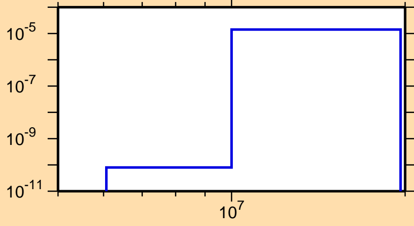
\sigma vs. E for ^{124}\text{Pr}(\text{mt } 45)
