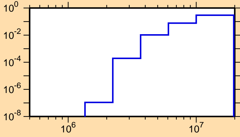
\sigma vs. E for ^{124}\text{Pr}(n,np)
