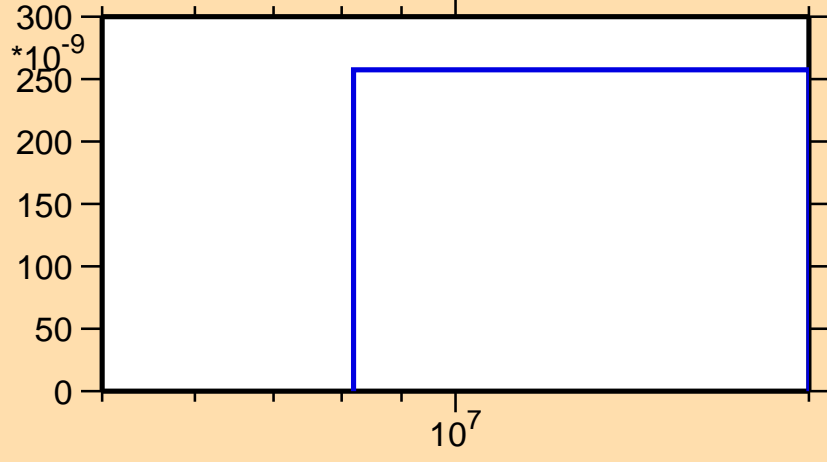
\sigma vs. E for ^{124}\text{Pr}(n,\text{nd})
