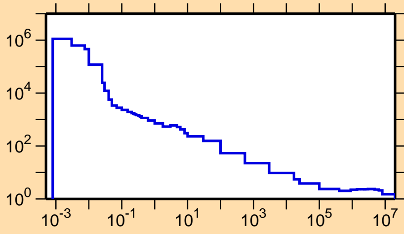
\sigma vs. E for ^{124}\text{Pr}(n,\text{nonel.})
