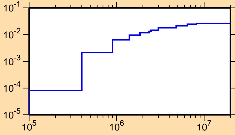
\sigma vs. E for ^{124}\text{Pr}(n,n_1)
