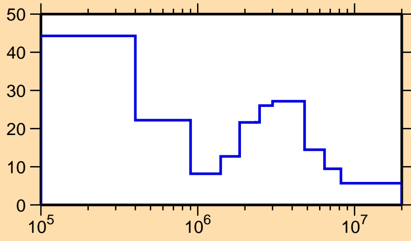
\Delta\sigma/\sigma vs. E for ^{124}\text{Pr}(n, el.)
