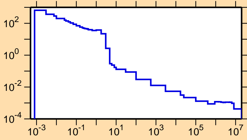
\sigma vs. E for ^{124}\text{Pr}(n,\gamma)
