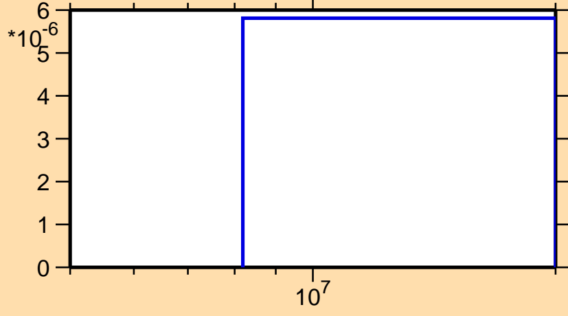
\sigma vs. E for ^{124}\text{Pr}(n,2np)
