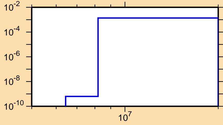
\sigma vs. E for ^{124}\text{Pr}(n,\text{pd})
