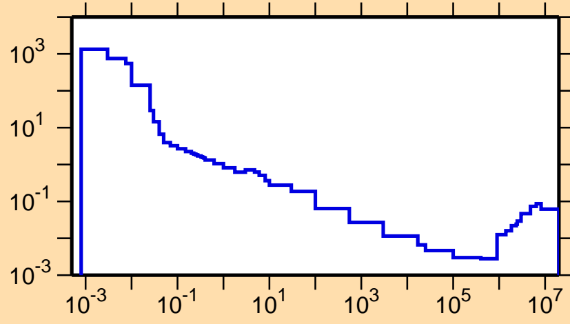
\sigma vs. E for ^{124}\text{Pr}(n,\alpha)
