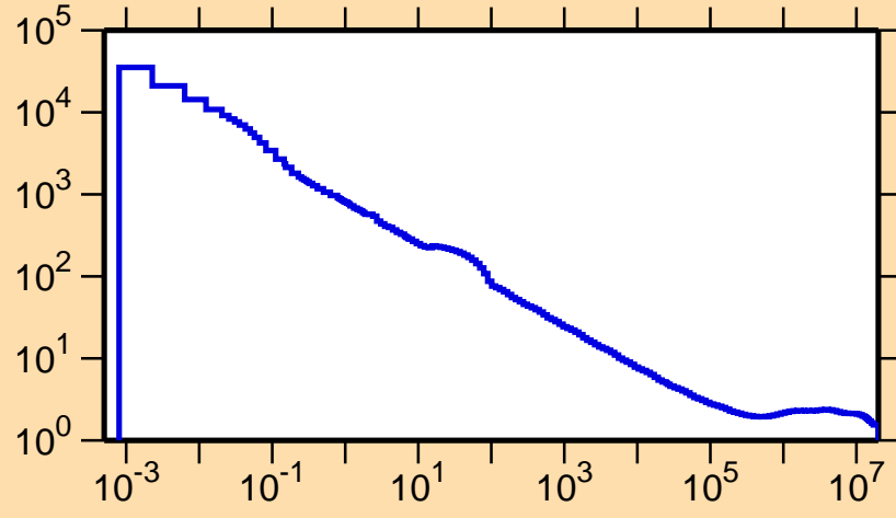
\sigma vs. E for ^{125}\text{Pr}(n,\text{nonel.})
