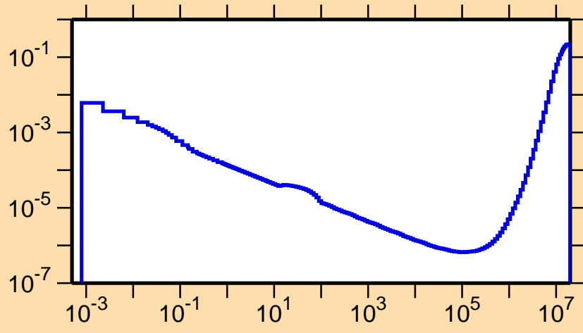
\sigma vs. E for ^{125}\text{Pr}(n,p\alpha)
