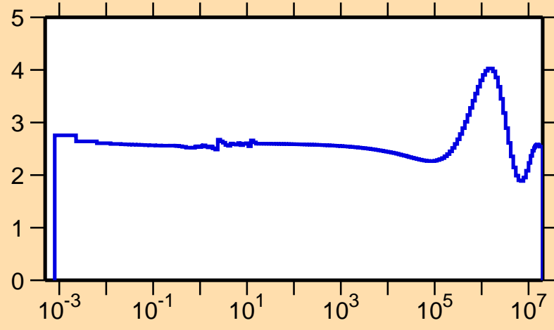
\sigma vs. E for ^{125}\text{Pr}(n,\text{el.})
