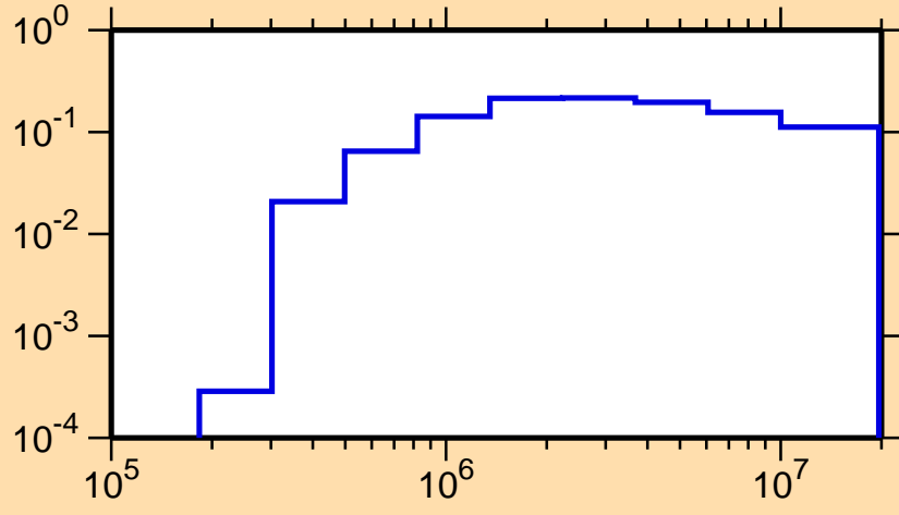
\sigma vs. E for ^{125}\text{Pr}(n,\text{inel.})
