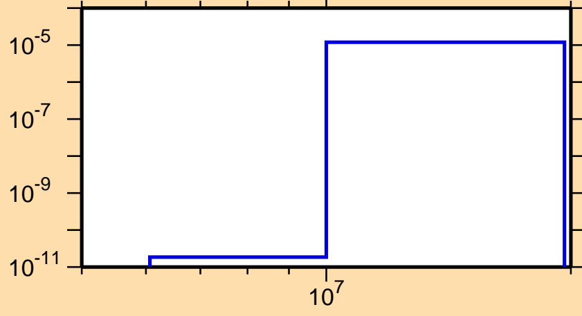
\sigma vs. E for ^{125}\text{Pr}(\text{mt } 45)
