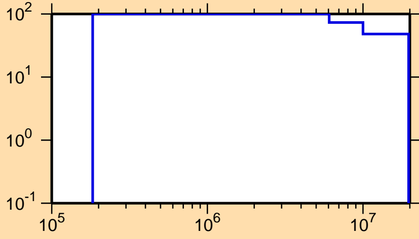
\Delta\sigma/\sigma vs. E for ^{125}\text{Pr}(n,n\text{cont.})
