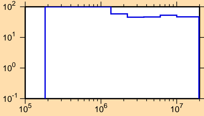
\Delta\sigma/\sigma vs. E for ^{125}\text{Pr}(n,n_1)
