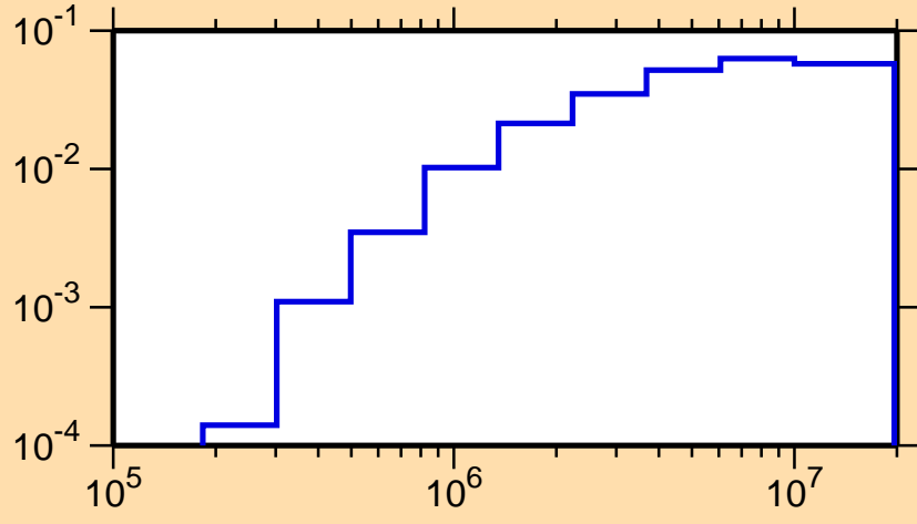
\sigma vs. E for ^{125}\text{Pr}(n,n\text{cont.})
