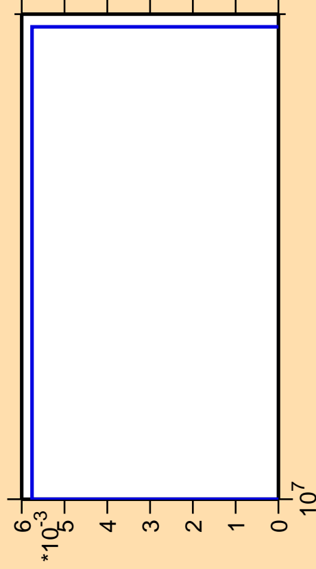
\Delta\sigma/\sigma vs. E for ^{125}\text{Pr}(n,2n\alpha)
