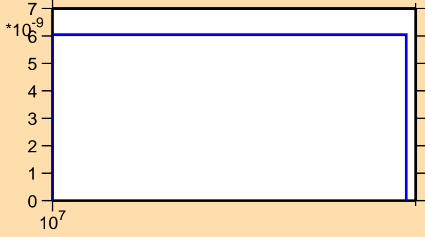
\sigma vs. E for ^{125}\text{Pr}(n,\text{nd})
