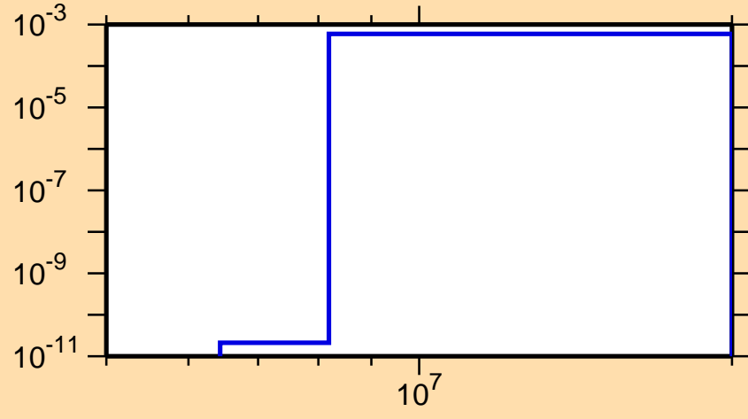
\sigma vs. E for ^{125}\text{Pr}(n,\text{pd})
