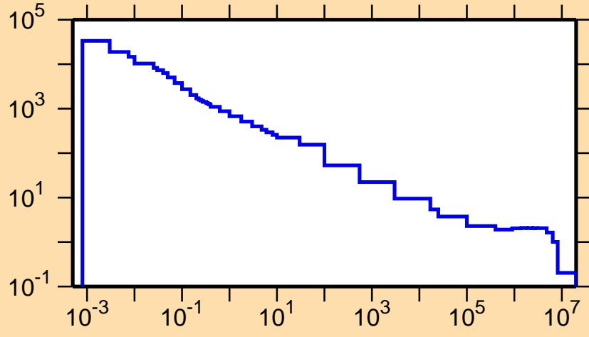
\sigma vs. E for ^{125}\text{Pr}(n,p)
