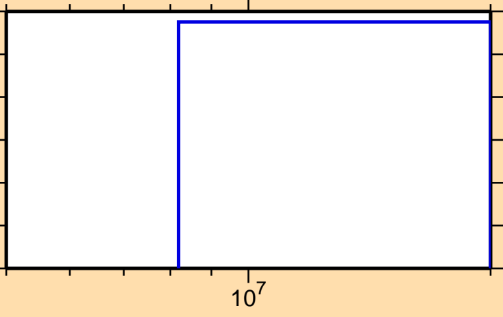
\sigma vs. E for ^{125}\text{Pr}(n,\text{pt})
