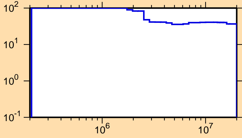
\Delta\sigma/\sigma vs. E for ^{126}\text{Pr}(n,\text{inel.})
