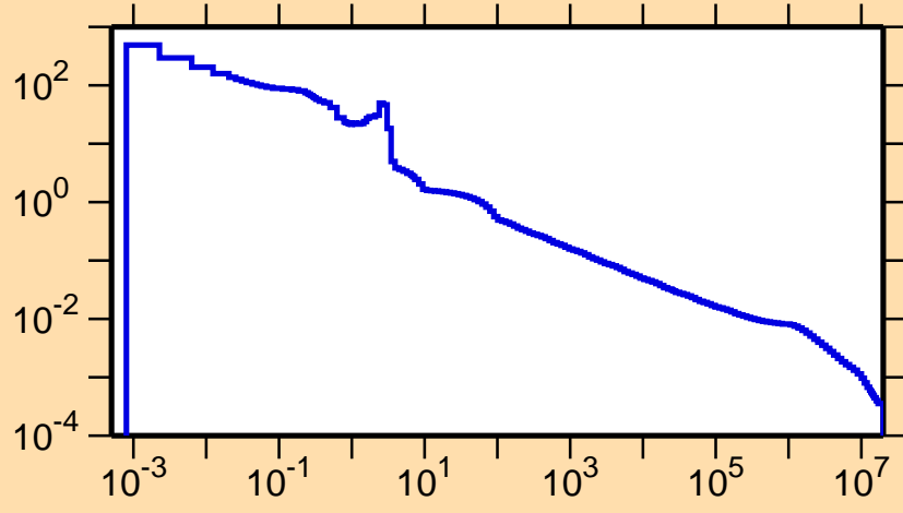
\sigma vs. E for ^{126}\text{Pr}(n,\gamma)
