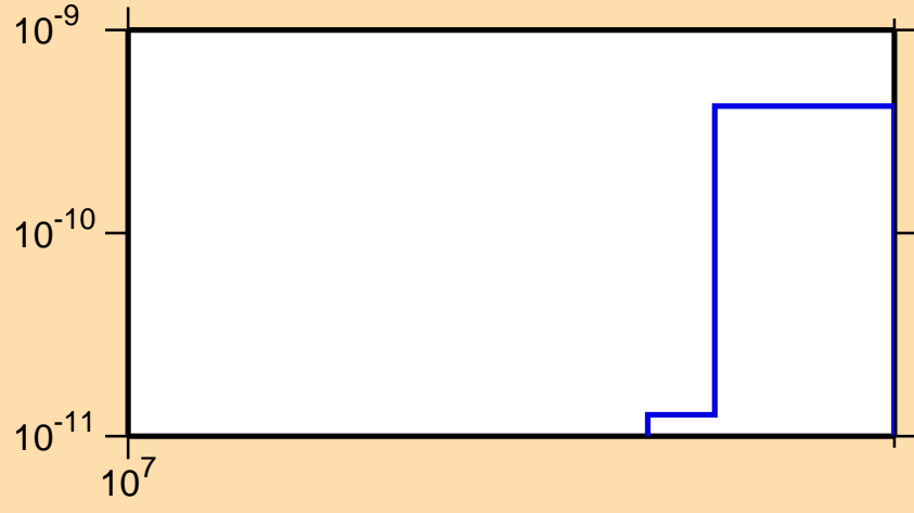
\sigma vs. E for ^{126}\text{Pr}(n,2n\alpha)
