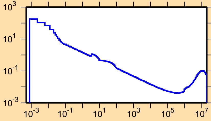
\sigma vs. E for ^{126}\text{Pr}(n,\alpha)
