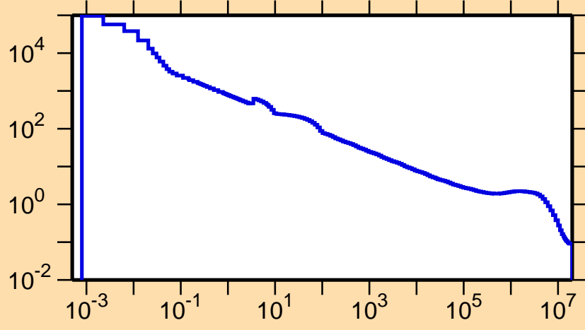
\sigma vs. E for ^{126}\text{Pr}(n,p)
