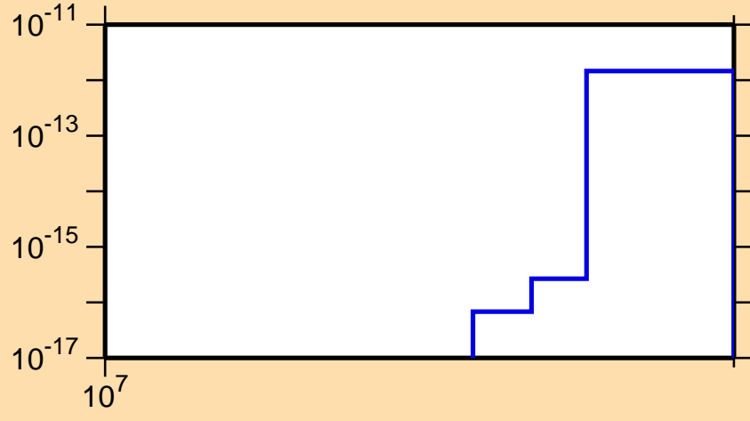
\sigma vs. E for ^{126}\text{Pr}(n,nt)
