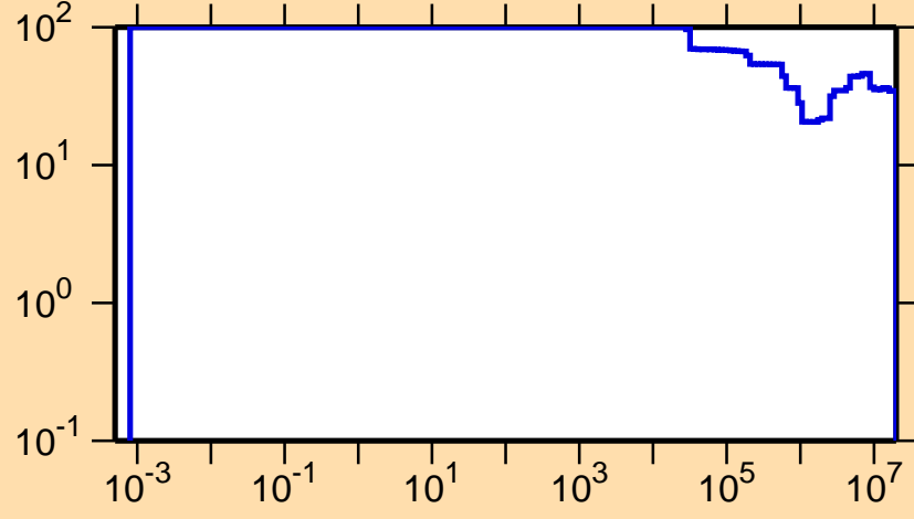
\Delta\sigma/\sigma vs. E for ^{126}\text{Pr}(n,p)
