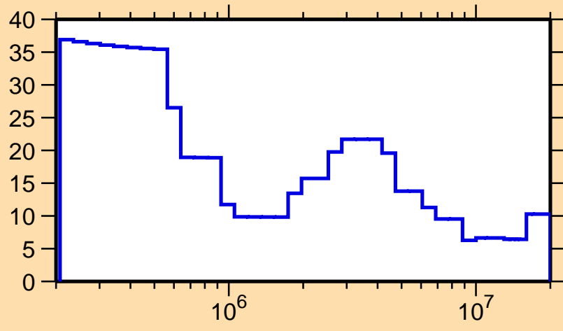
\Delta\sigma/\sigma vs. E for ^{126}\text{Pr}(n,\text{el.})
