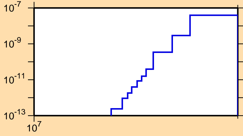
\sigma vs. E for ^{126}\text{Pr}(\text{mt } 34)
