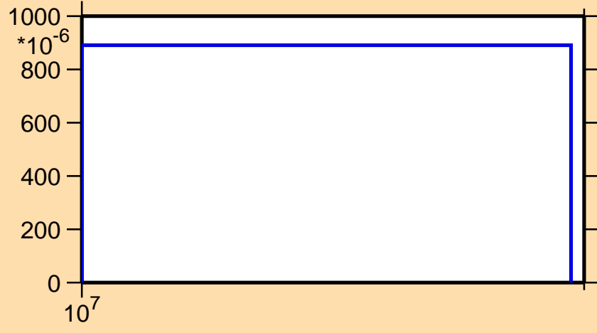
\sigma vs. E for ^{126}\text{Pr}(n,2n)
