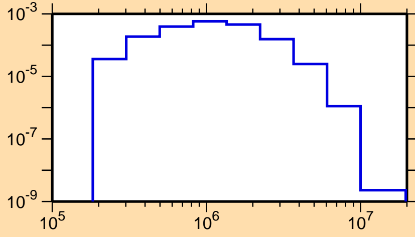
\sigma vs. E for ^{126}\text{Pr}(n,n_1)
